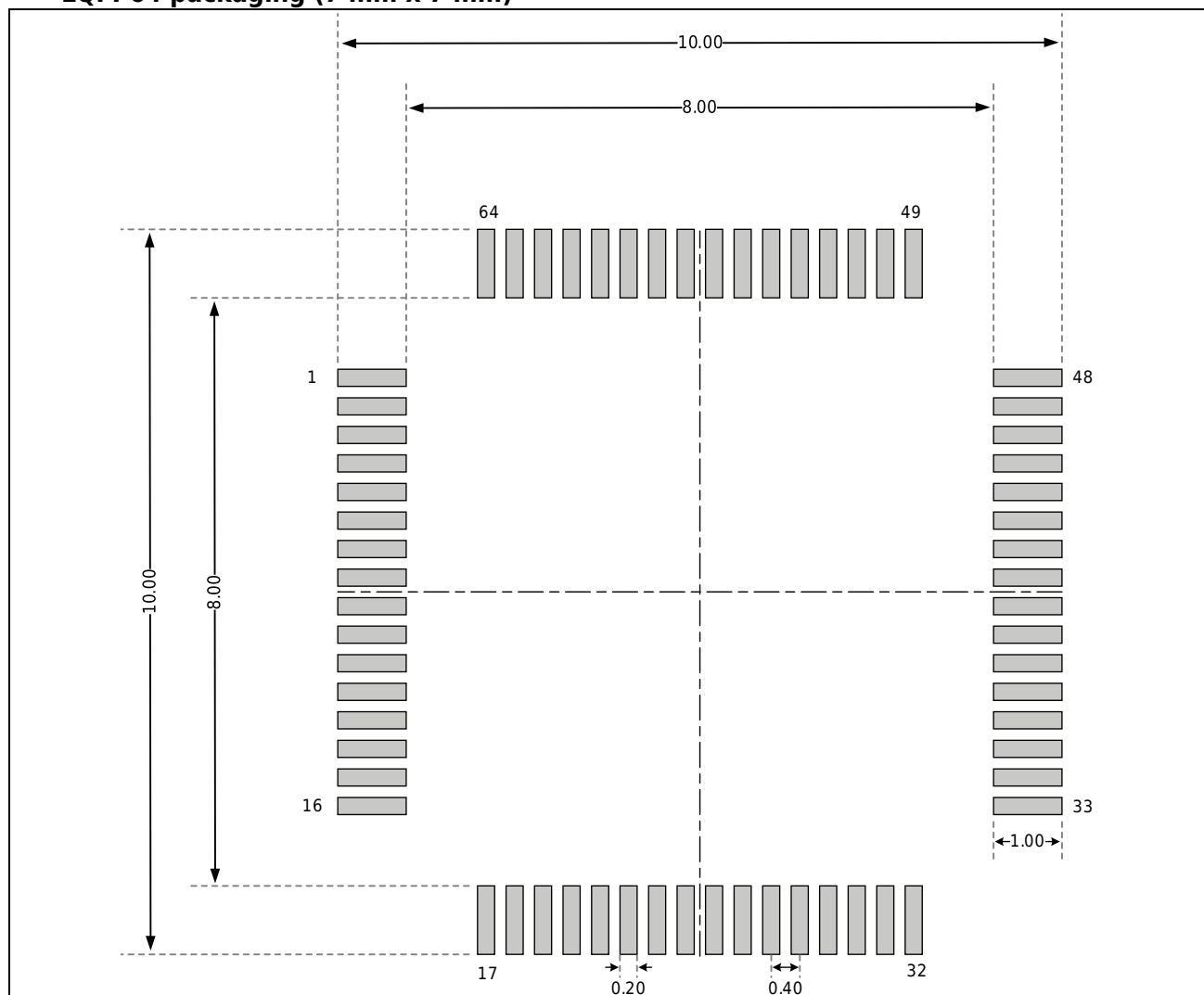
LQFP64 packaging (7 mm x 7 mm)
