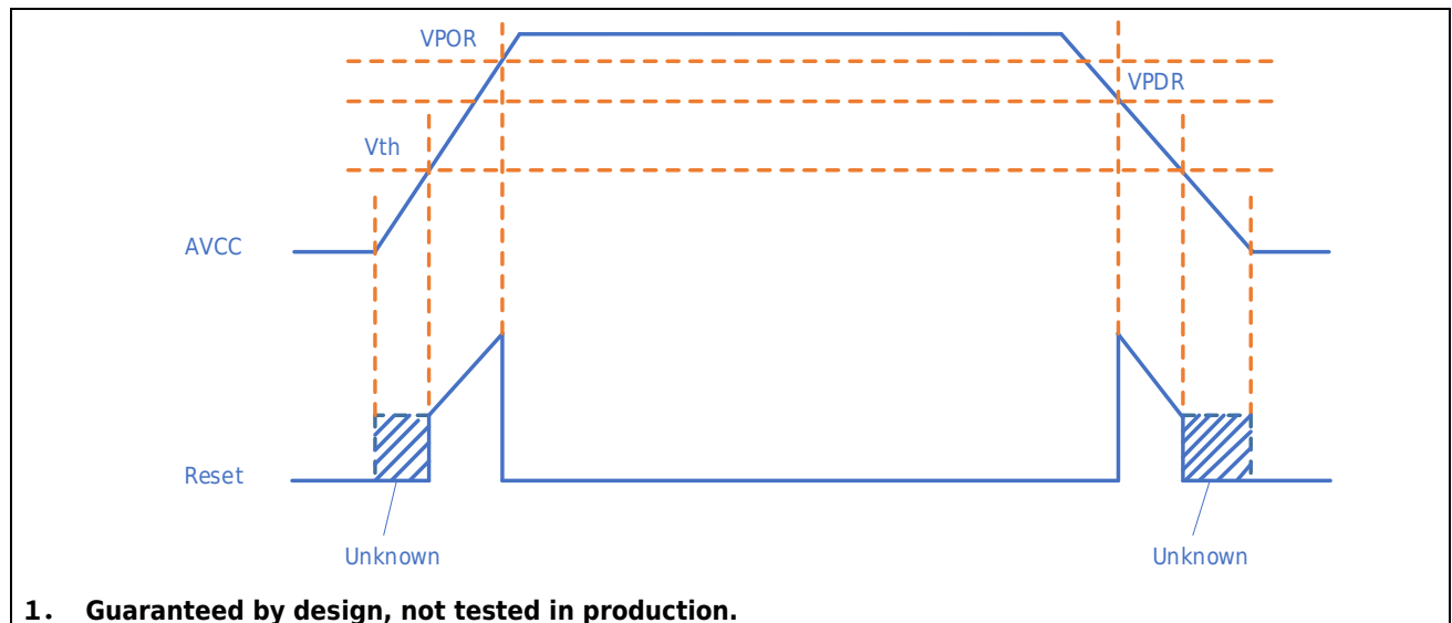
Figure 7-1 POR/PDR Schematic
