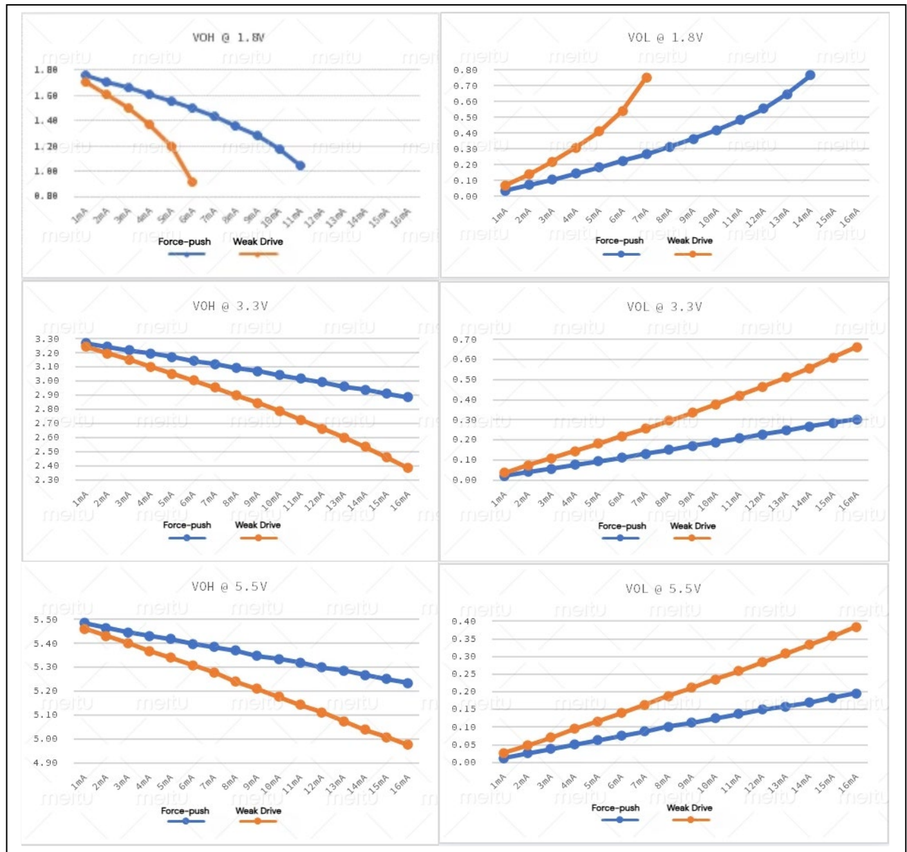
Figure 7-2 Output Port VOH/VOL Measured Curve
