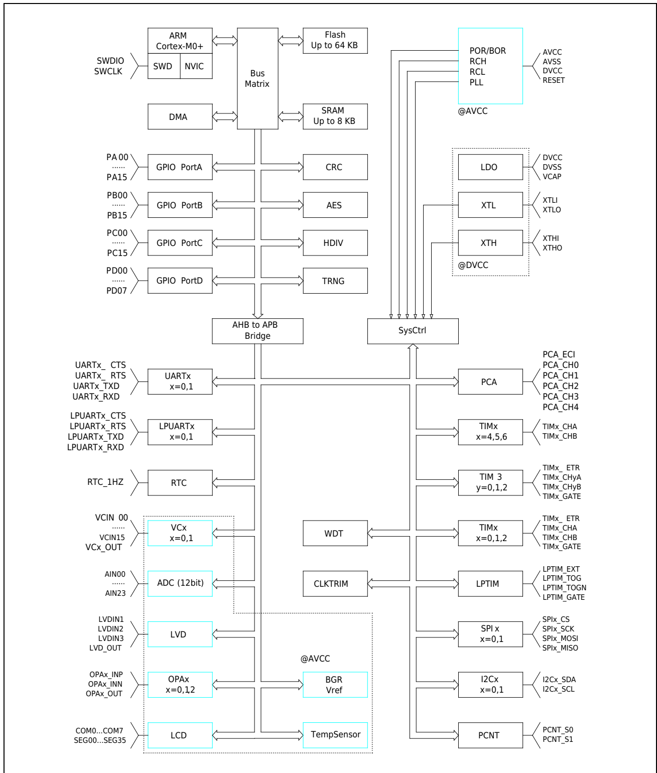
Figure 4-1 Functional Modules
