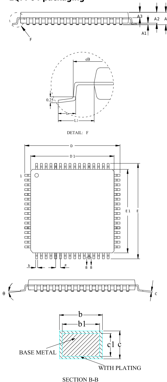
LQFP64 packaging
