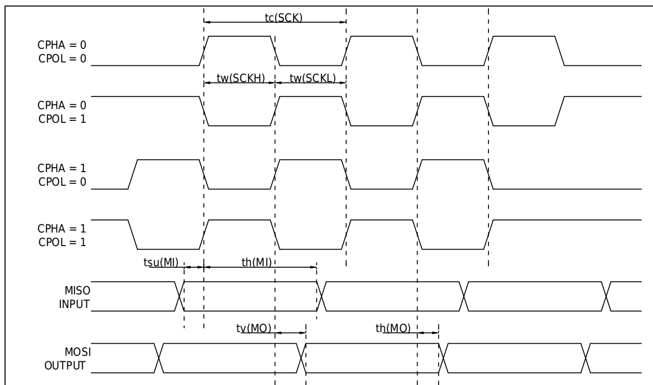
Figure 7-4 SPI Timing Diagram (Host Mode)
