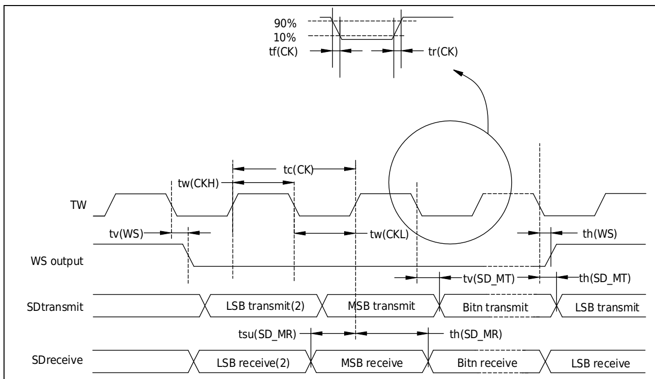
图 7-7 I2S slave timing diagram
