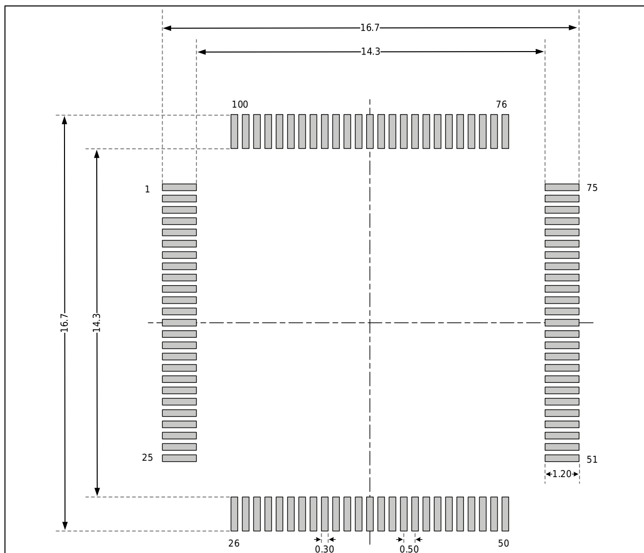
LQFP100 封装 (14mm x 14mm)
