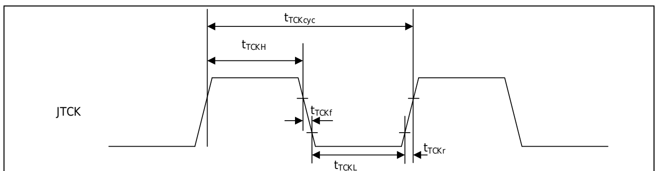
Figure 3-13 JTAG JTCK Clock
