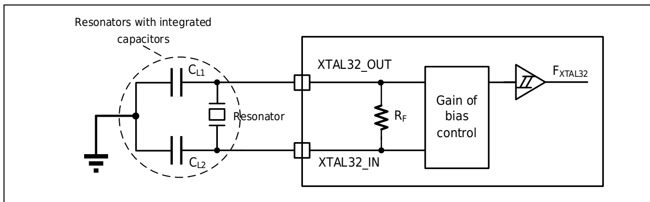
Figure 3-5 Typical Application with 32.768KHz Crystal
