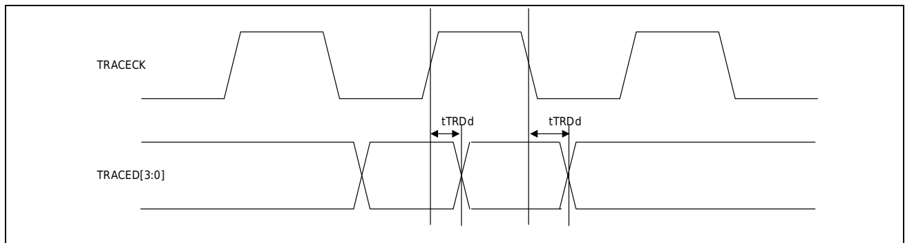
Figure 3-18 TRACE Data Output
