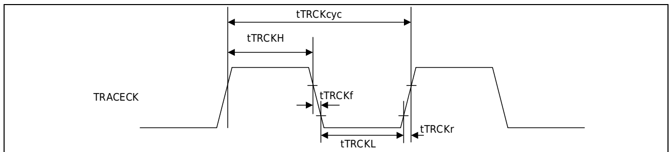
Figure 3-17 TRACE Clock
