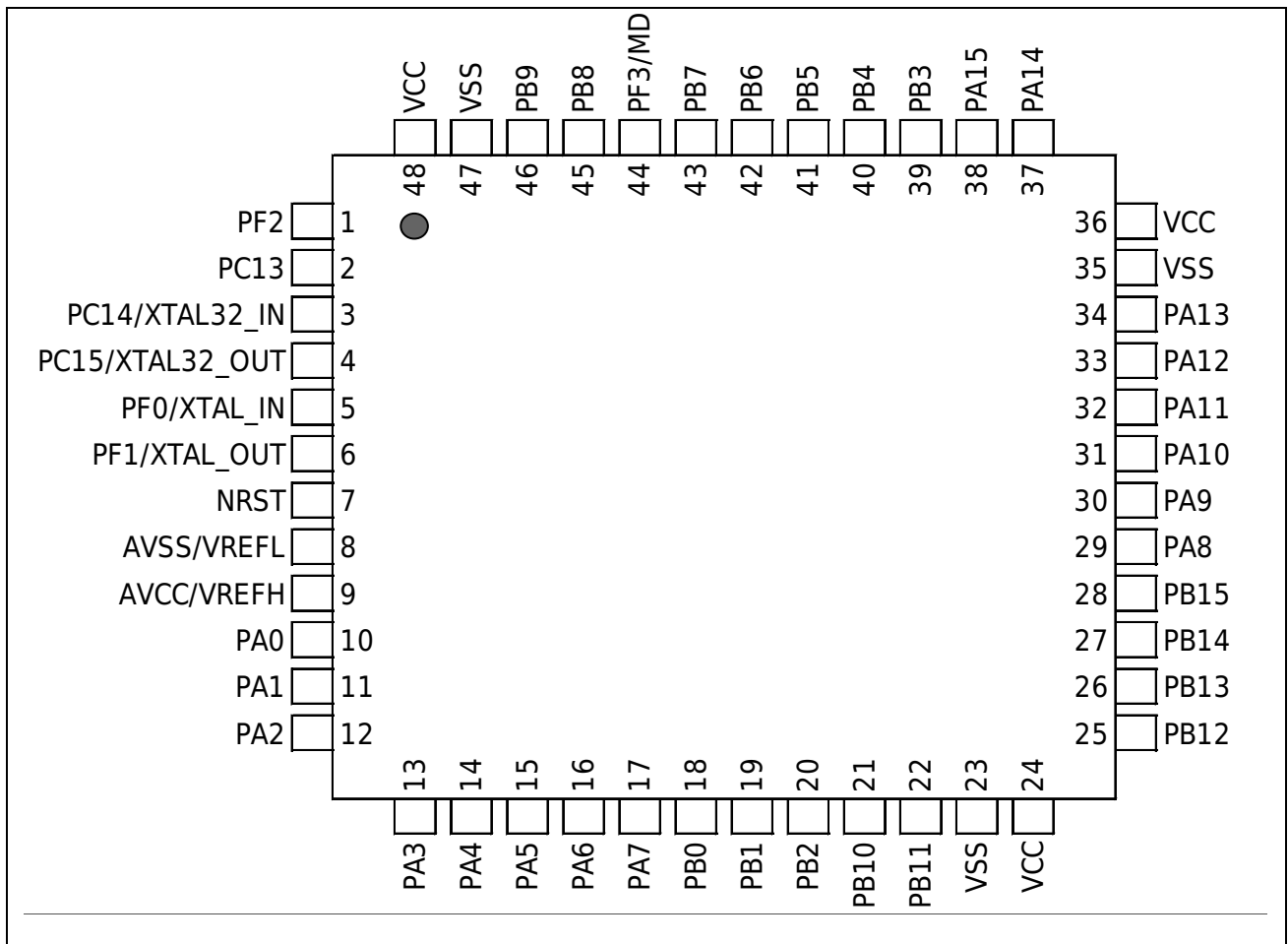
Figure 2-1 Pin Configuration Diagram
