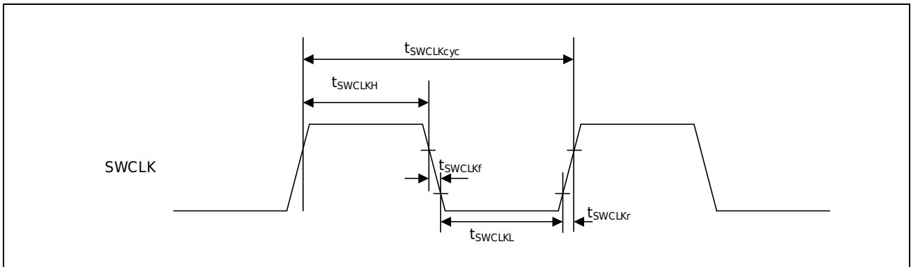
Figure 3-15 SWD SWCLK Clock
