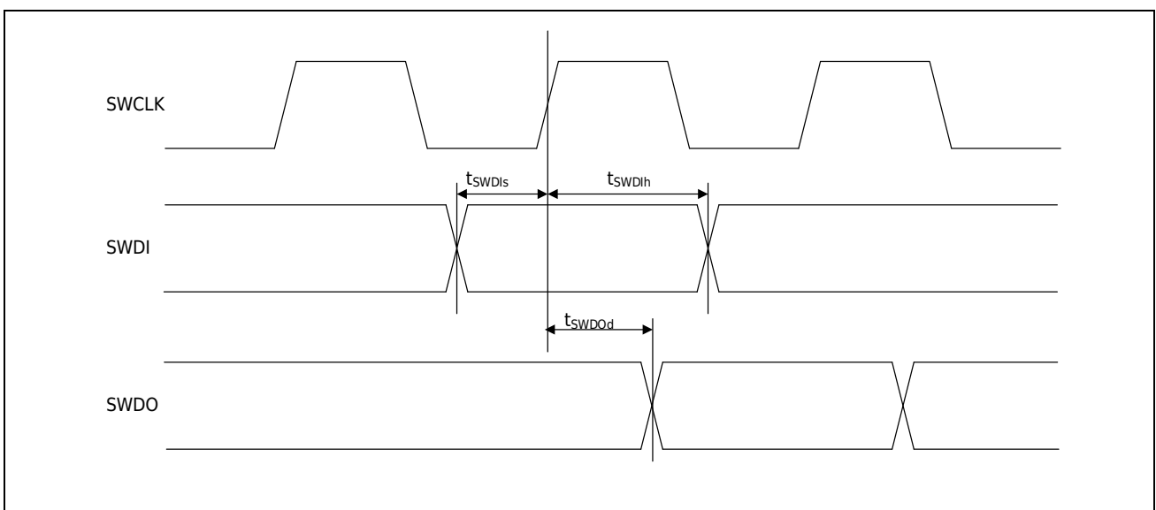
Figure 3-16 SWDIO Input and Output
