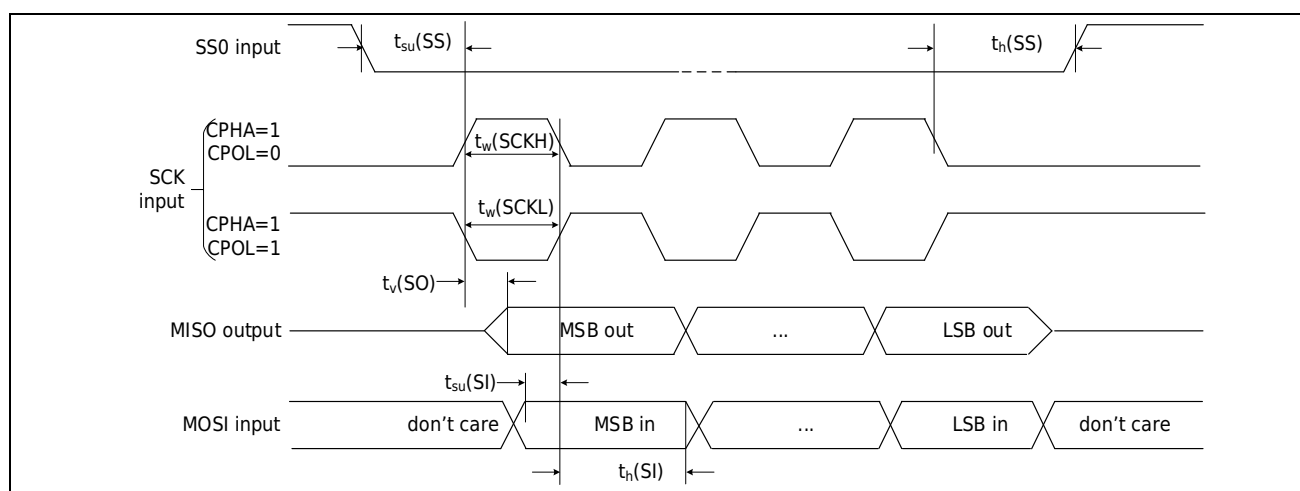
Figure 3-9 SPI Timing Definition (Slave Mode, CPHA=1)
