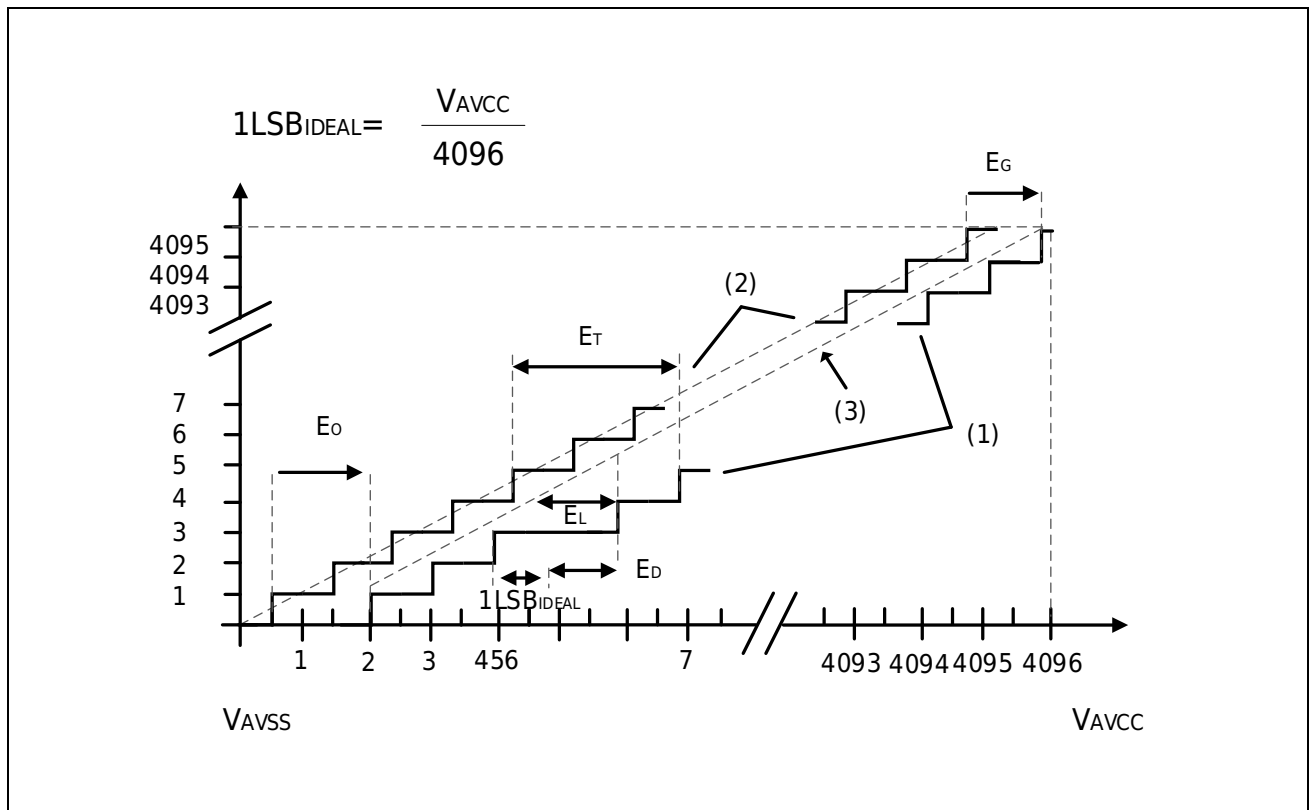
Figure 3-19 ADC Accuracy Features
