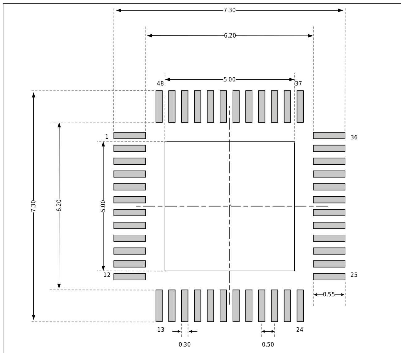
Figure 7-3 Schematic diagram of QFN48 pad
