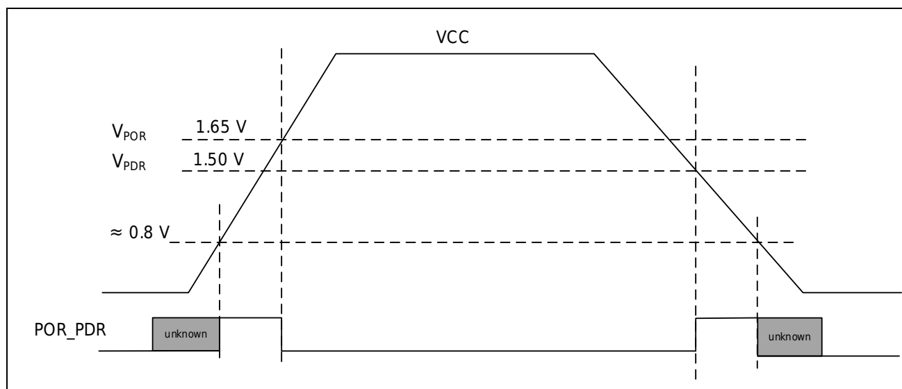
Figure 6-2 POR/PDR Schematic
