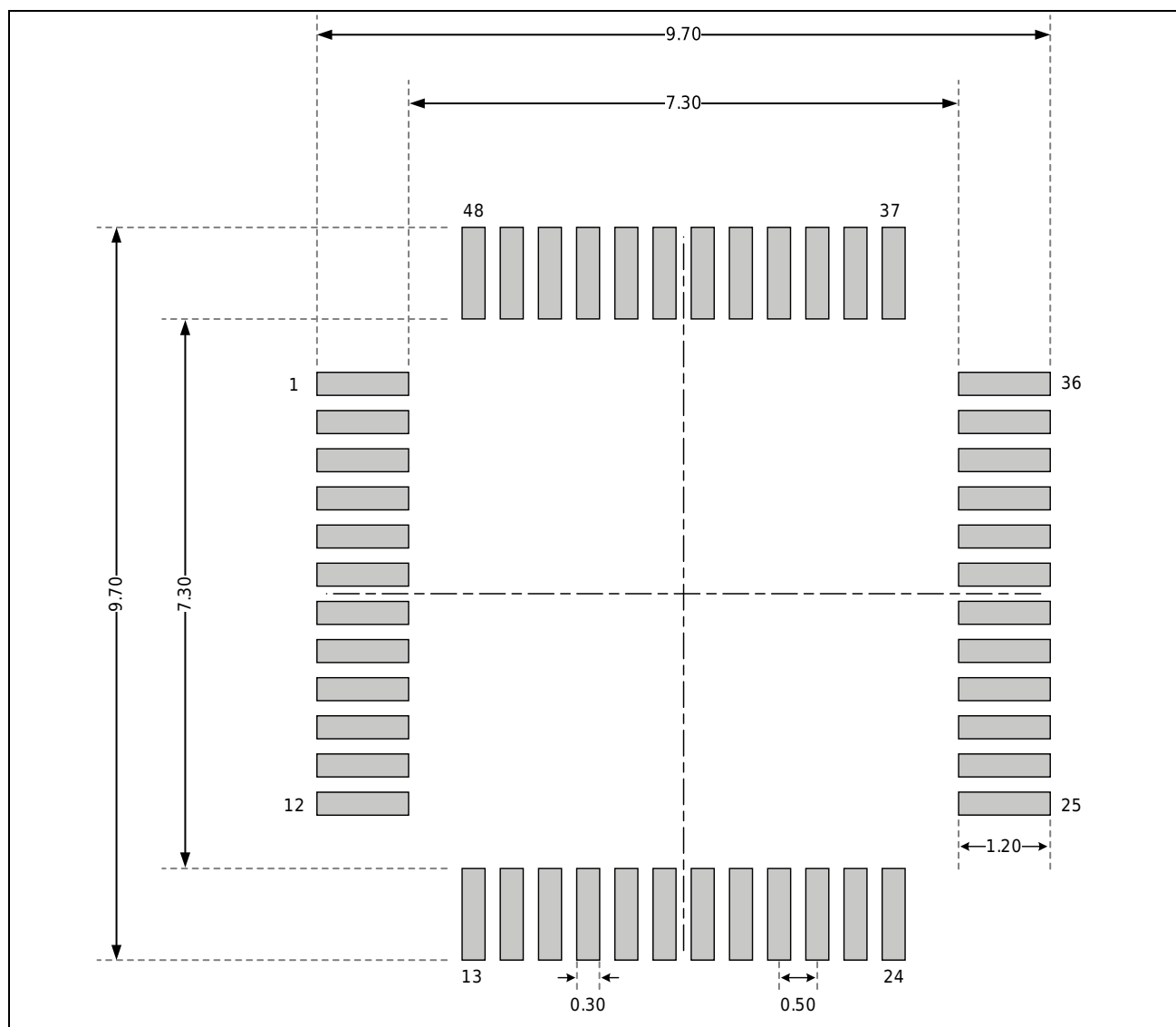
Figure 7-2 Schematic diagram of LQFP48 pad
