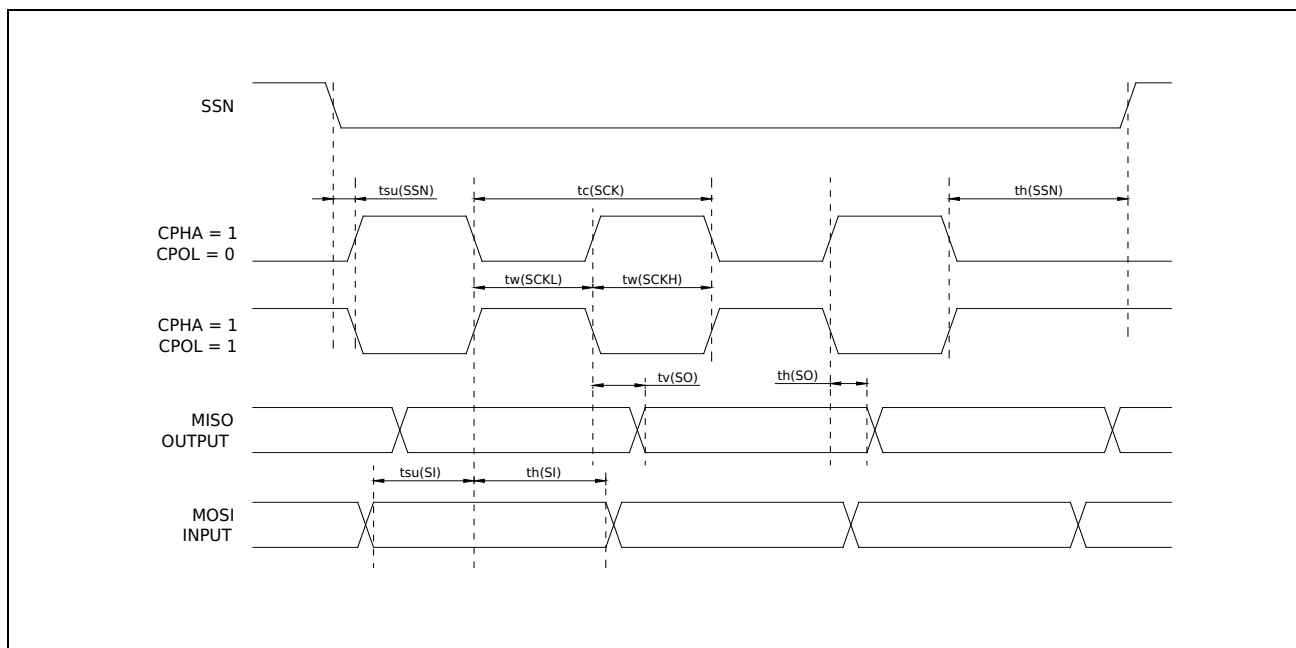
Figure 6-7 SPI timing diagram (slave mode CPHA=1)
