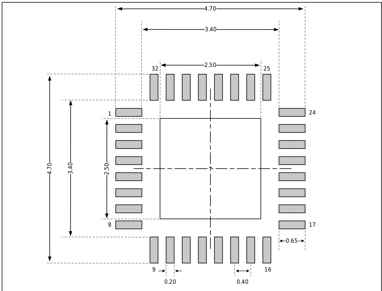
Figure 7-4 Schematic diagram of QFN32 pad
