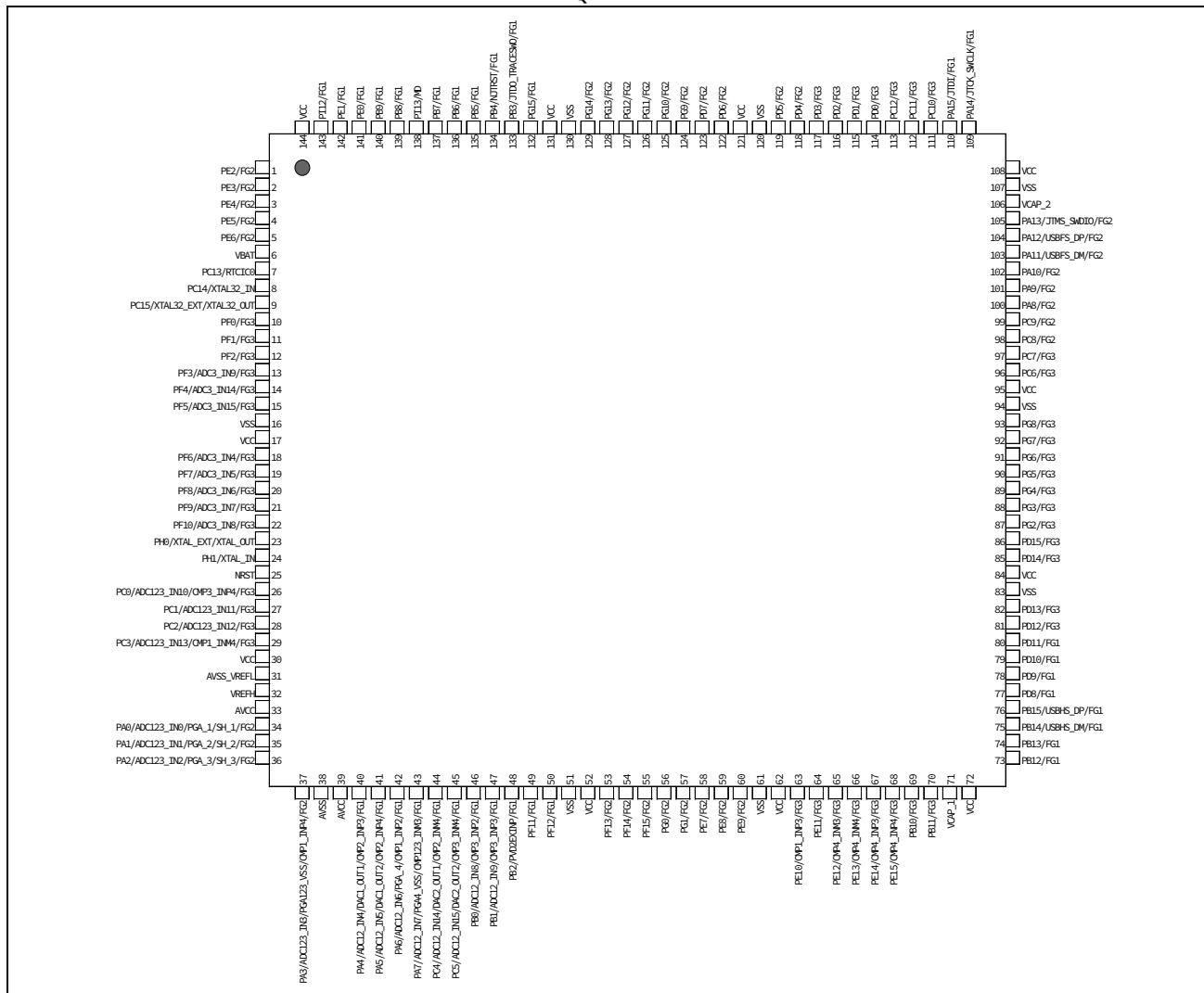
LQFP144
