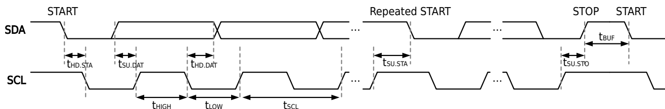
Figure 5-8 I2C Interface Timing
