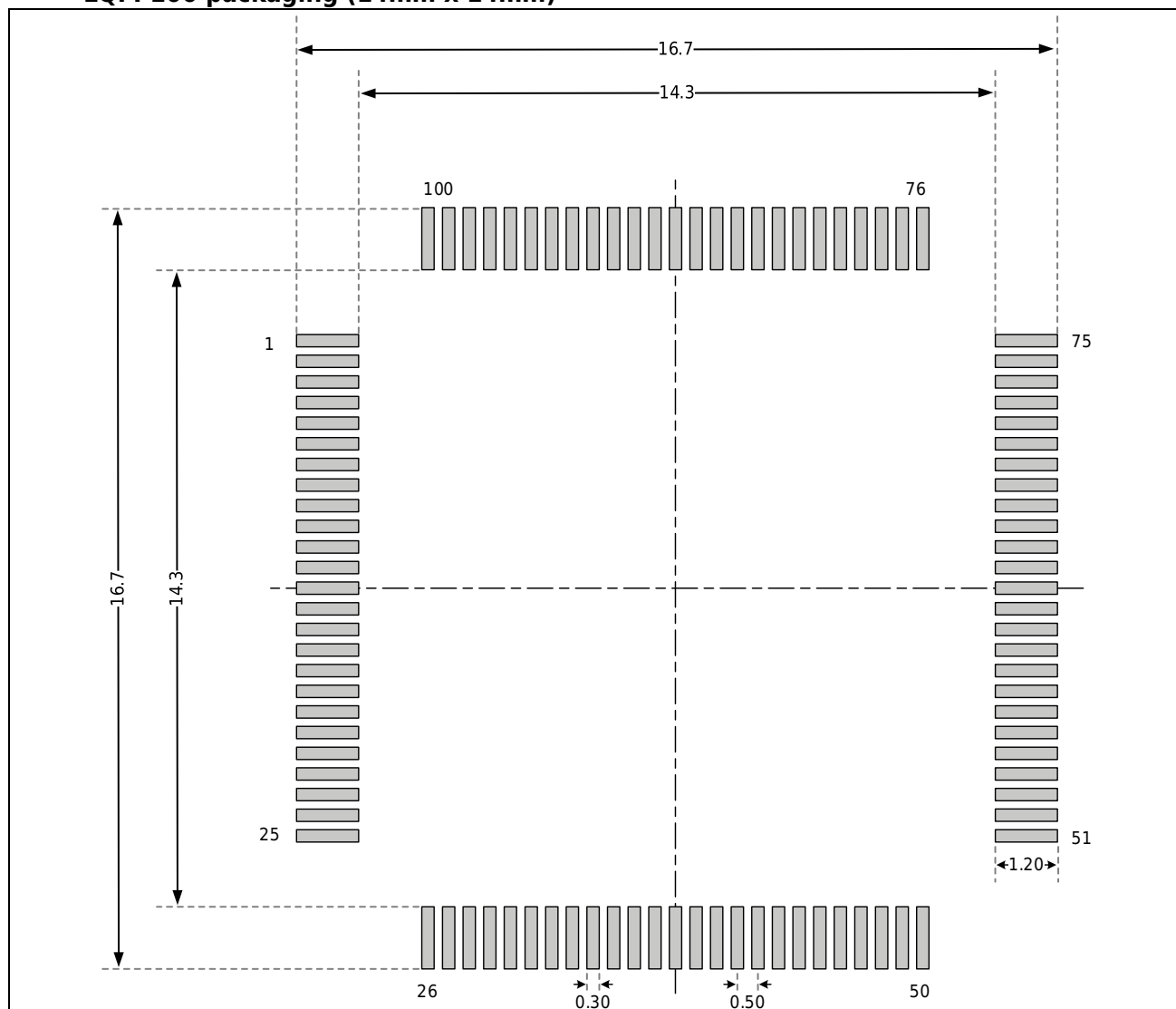
LQFP100 packaging (14mm x 14mm)
