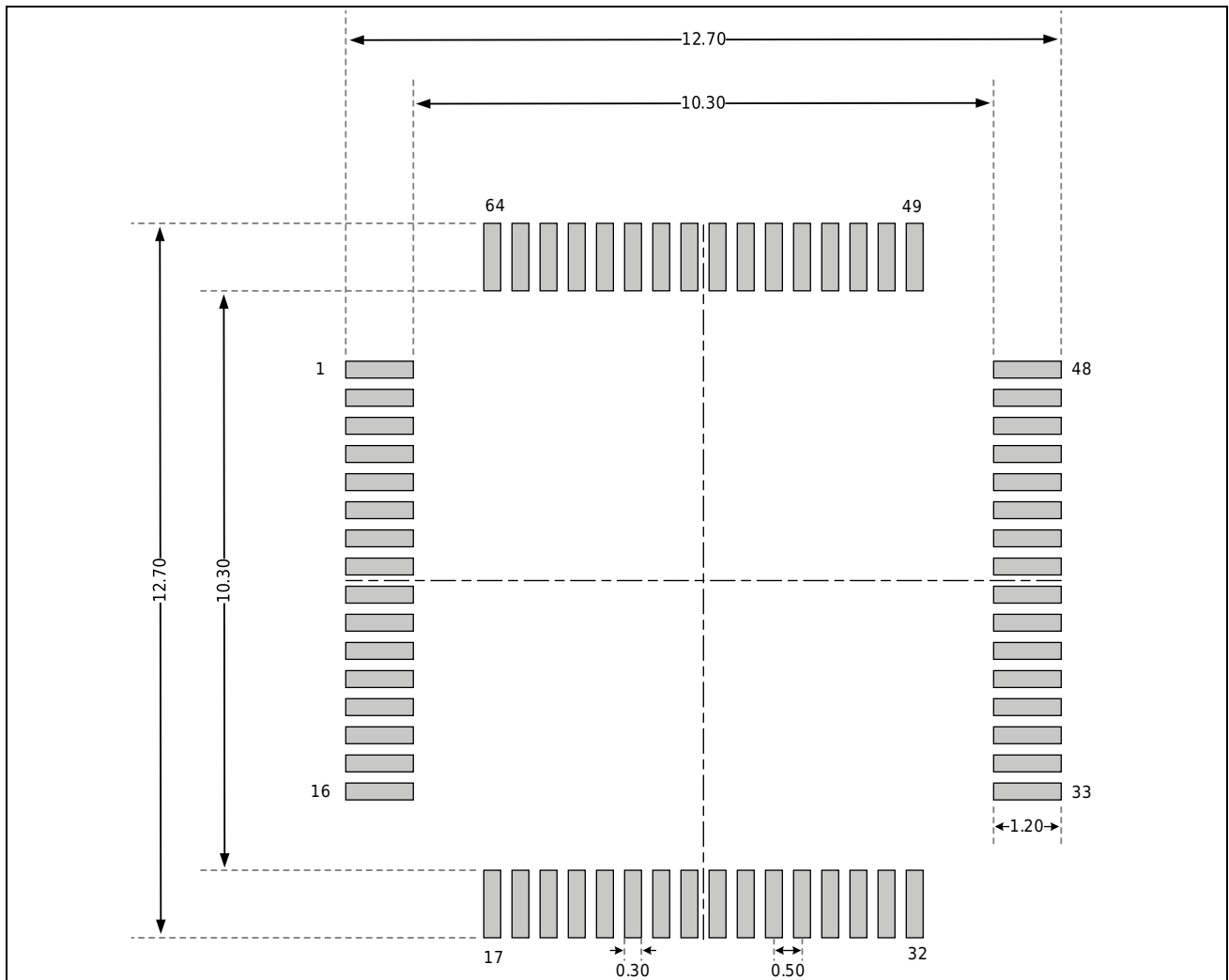
LQFP64 封装 (10mm x 10mm)
