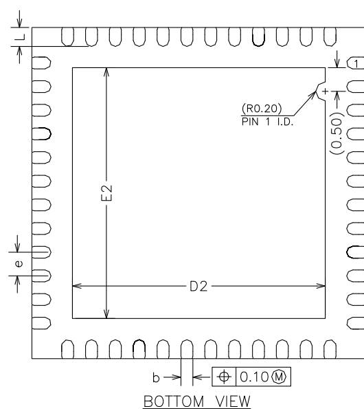
DETAIL A
