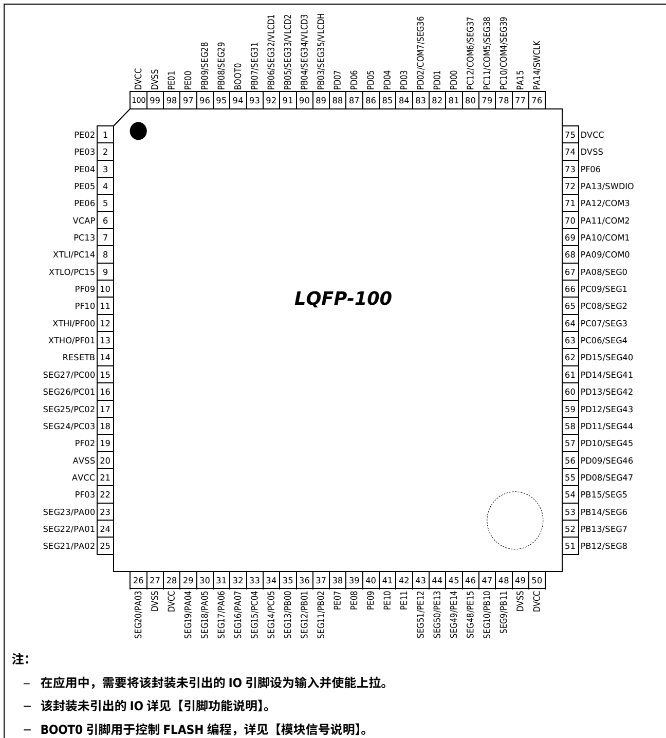
HC32L176PATA-LQFP100
