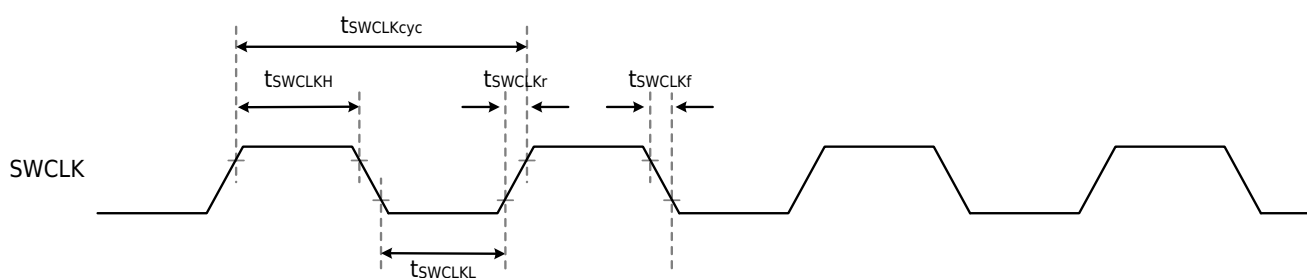
Figure 4-12 SWCLK Clock
