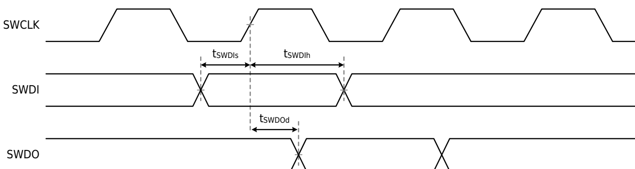
Figure 4-13 SWDIO Input/Output
