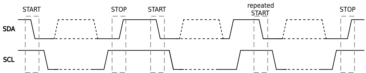
Figure 7-2 START, Repeated START and STOP
