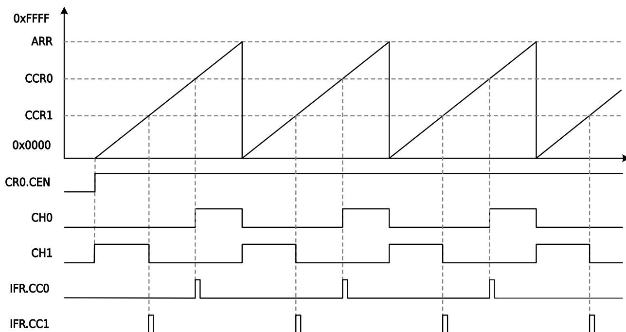
Figure 14-21 GTIM Compare Function Diagram
