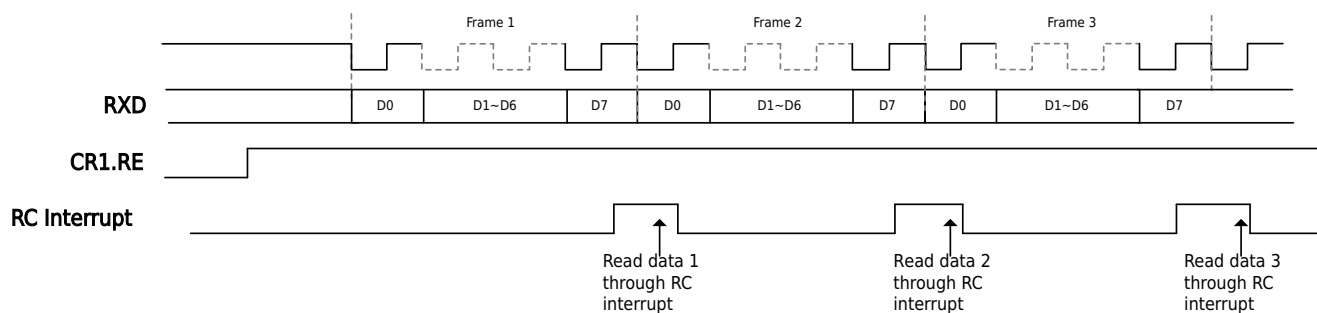
Figure 19-12 Synchronous Serial Port Mode Receiving Data Legend 1 (LSB/No RTS Function)
