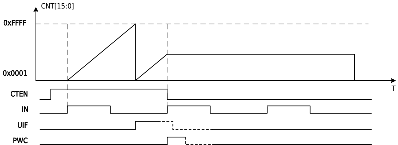
Figure 13-13 Model1: Pulse Width Measurement PWC Rising Edge to Rising Edge Period Measurement Single Mode
