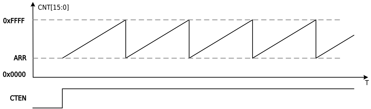
Figure 13-5 Mode0 Count Timer 16-Bit Reload Counting Waveform
