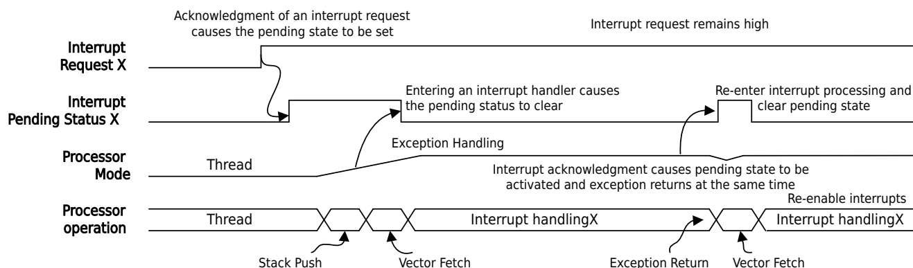
Figure 5-4 When the Interrupt Exits, If the Interrupt Request Remains High, It Will Cause the Interrupt Processing to Be Executed Again
