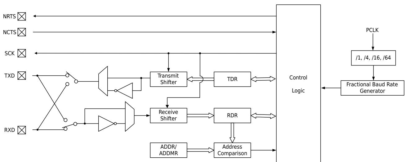
Figure 19-4 Asynchronous Serial Port Function Block Diagram
