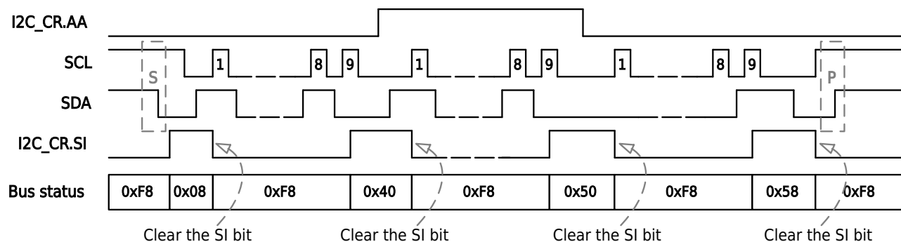
Figure 7-9 Data Synchronization Diagram of Master Receiving Mode
