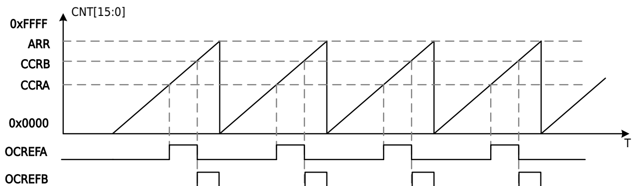
Figure 13-36 Sawtooth Counting Dual Point Comparison OCREF Output Waveform (OCMyx=0b111)
