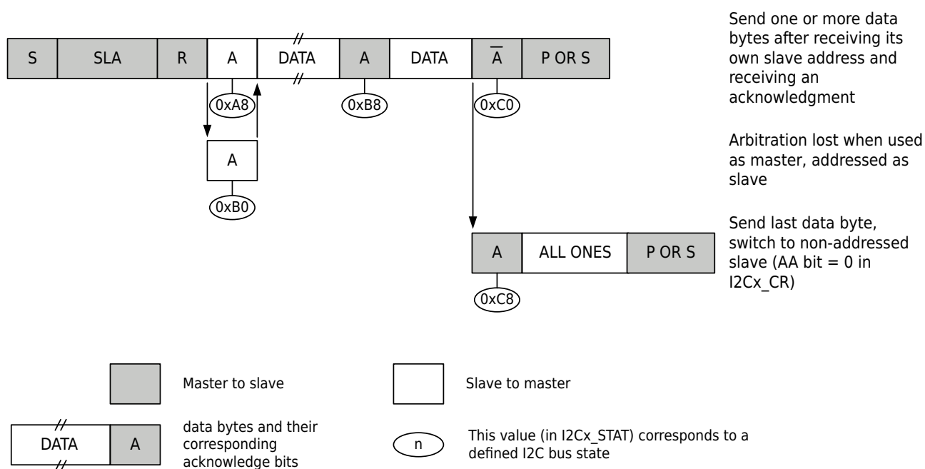
Figure 7-14 I2C Slave Sending State Diagram
