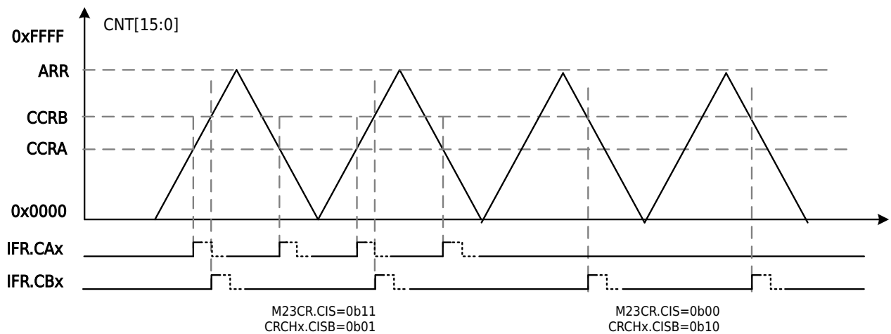
Figure 13-48 Compare Interrupt Diagram
