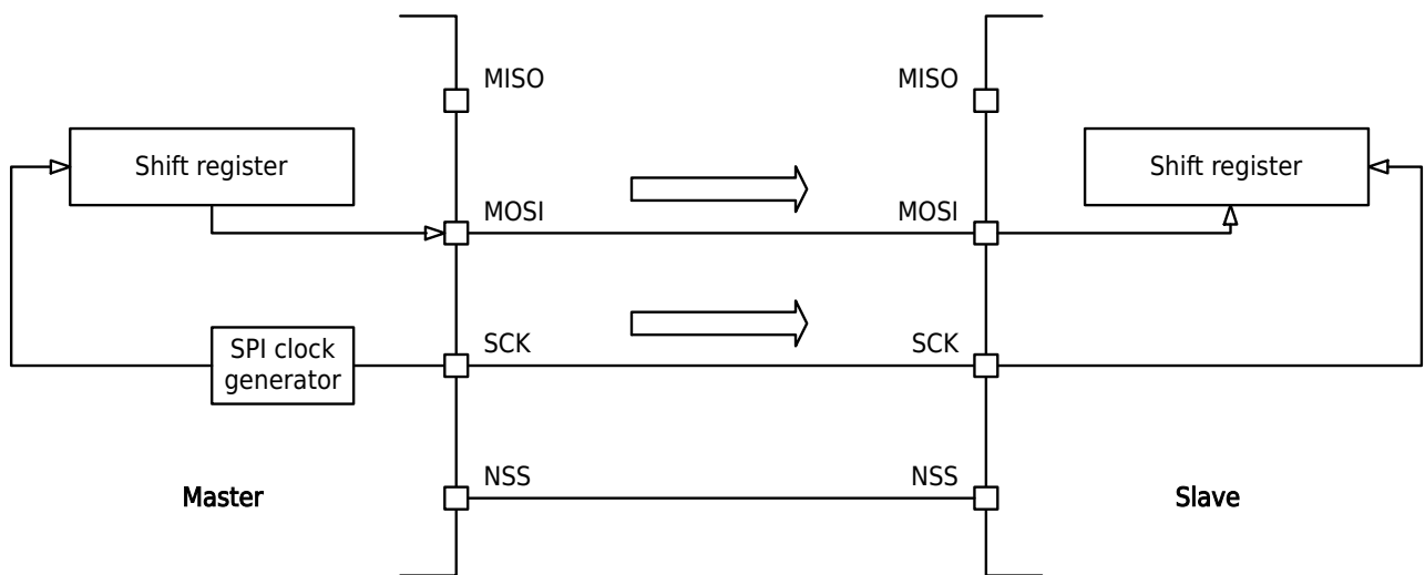
Figure 8-6 SPI Simplex Transmit Communication Diagram
