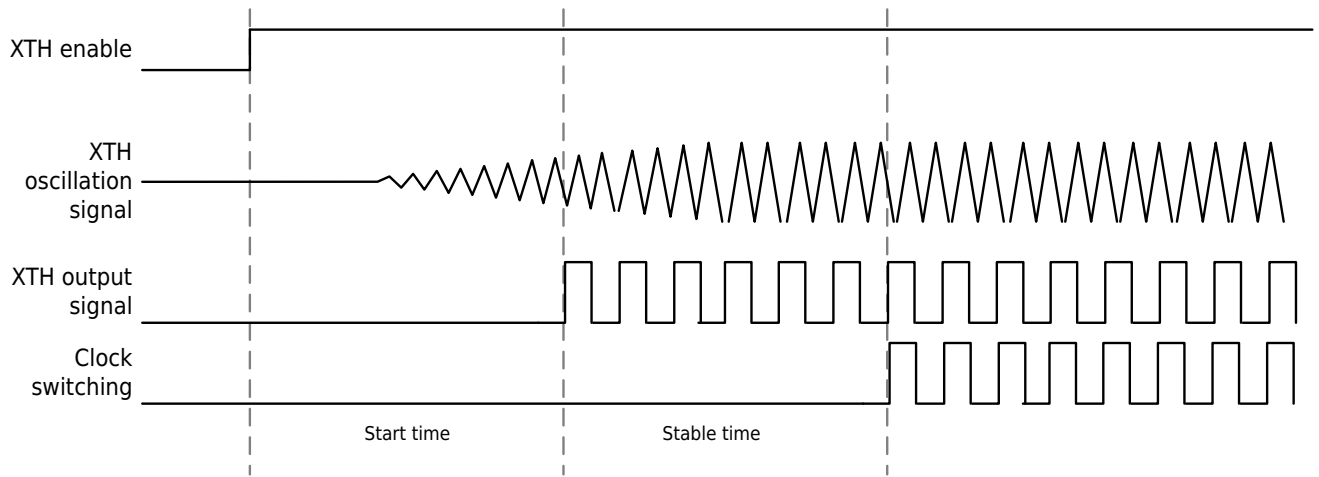
Figure 4-3 Crystal Oscillator Clock Startup Diagram
