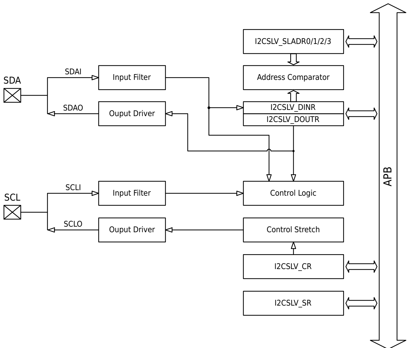
Figure 23-1 I2C SLAVE Module Block Diagram
