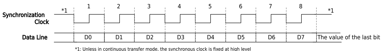
Figure 19-9 Synchronize Serial Port Mode Data Format
