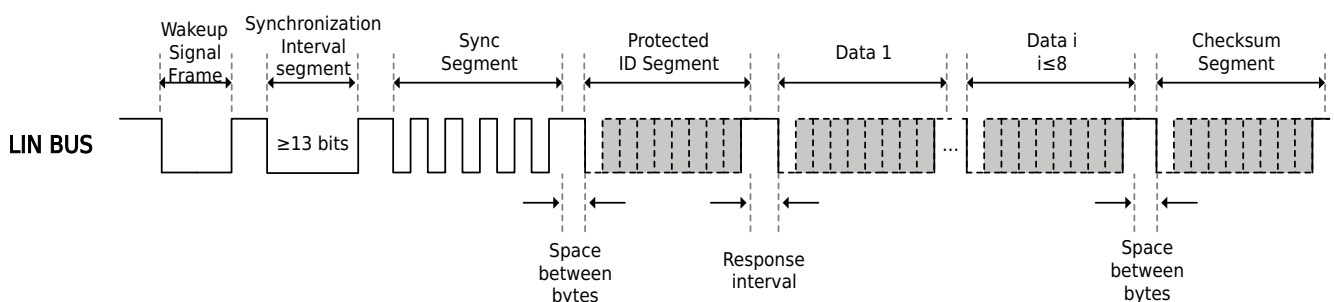
Figure 19-23 LIN Bus Data and Frame Structure
