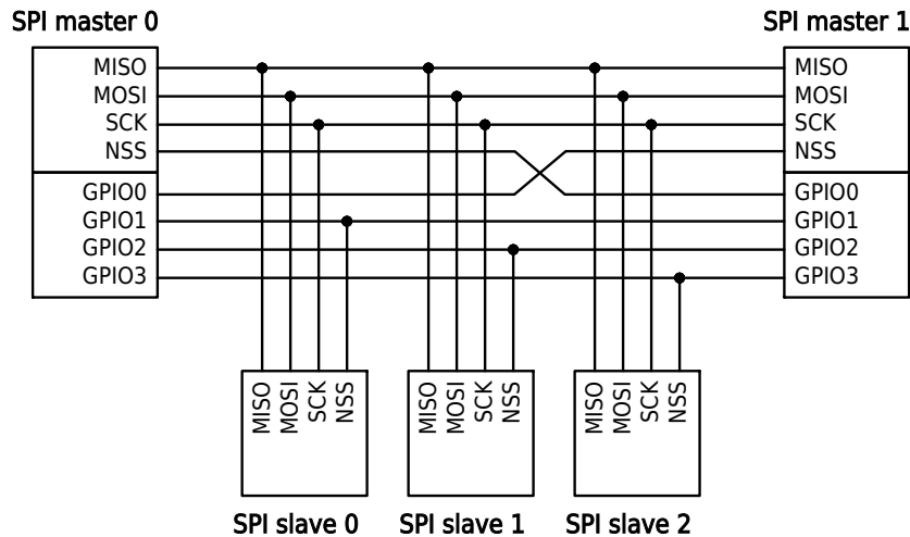
Figure 8-8 SPI Multi-machine System
