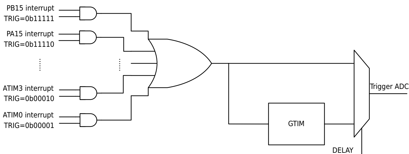
Figure 25-6 Diagram of External Trigger Sources for ADC Single and SQR Scan Conversions
