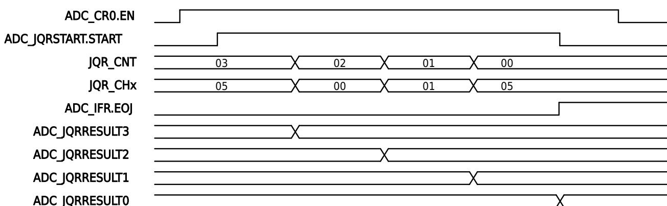
Figure 25-4 Examples of ADC JQR Scan Conversion Process
