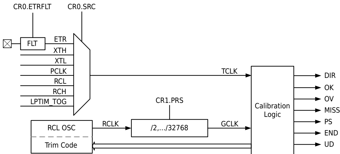
Figure 9-2 RCL Clock Calibration Operational Block Diagram
