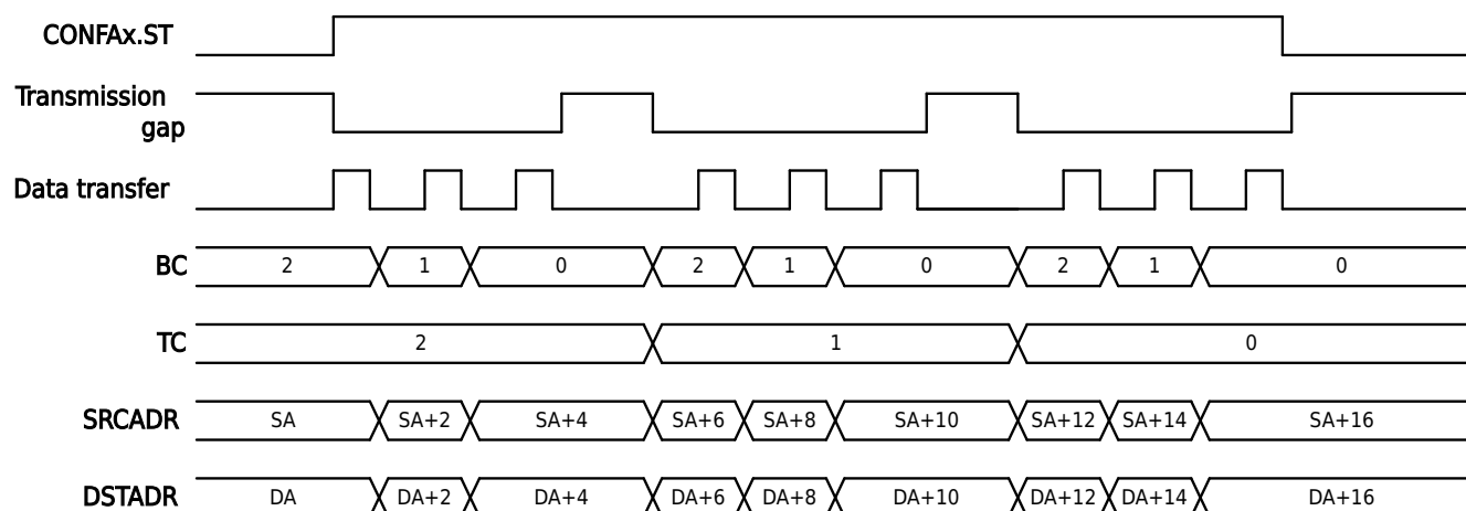
Figure 12-2 DMA Software Block Transfer Mode
