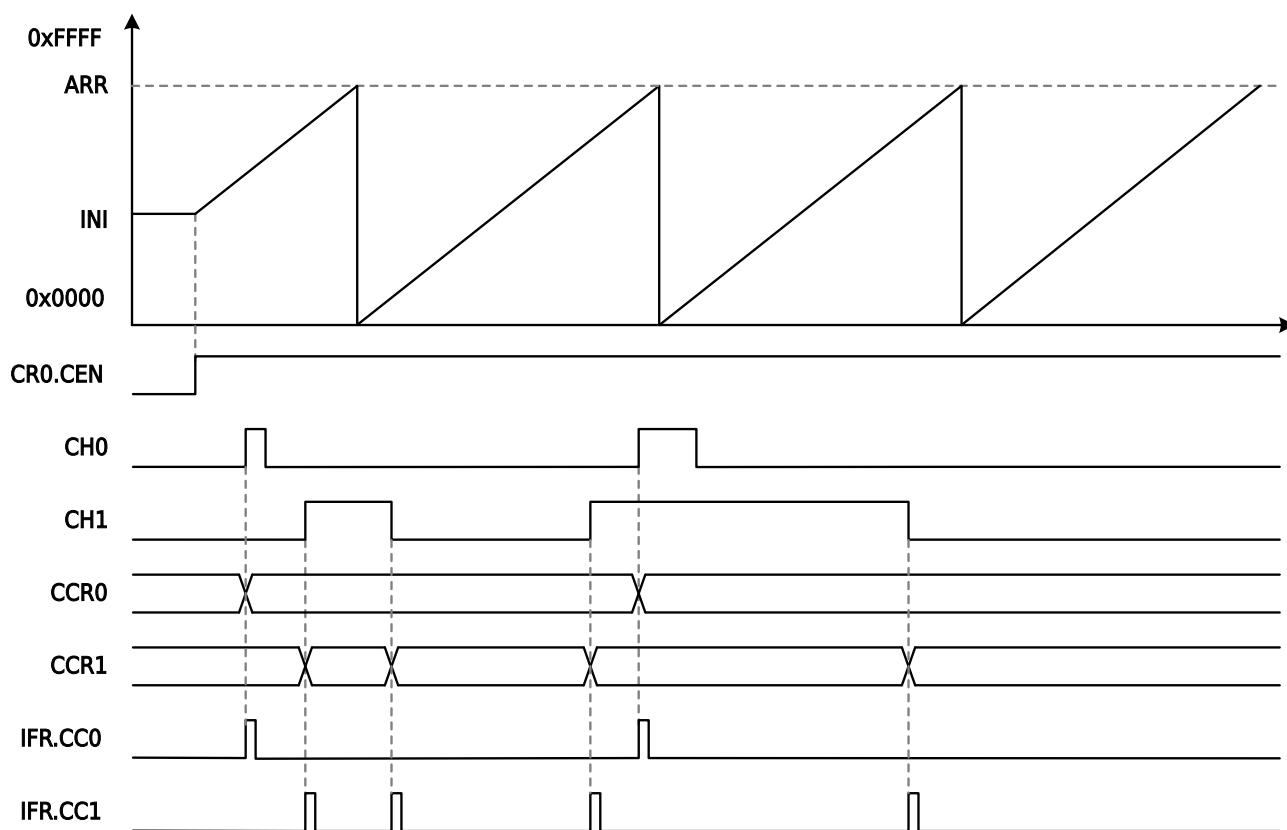
Figure 14-20 GTIM Capture Function Diagram
