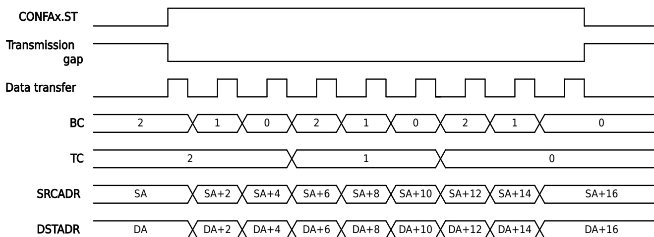
Figure 12-3 DMA Software Burst Transfer Mode
