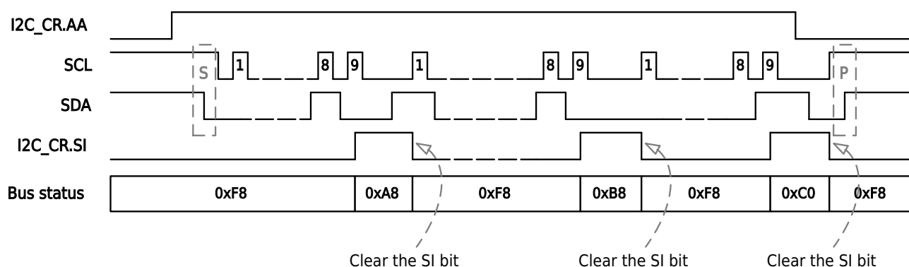
Figure 7-13 Slave Sending Mode Data Synchronization Diagram
