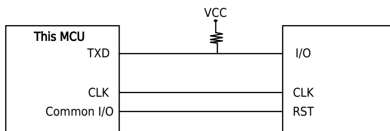
Figure 19-15 Smart Card Connection Schematic Diagram
