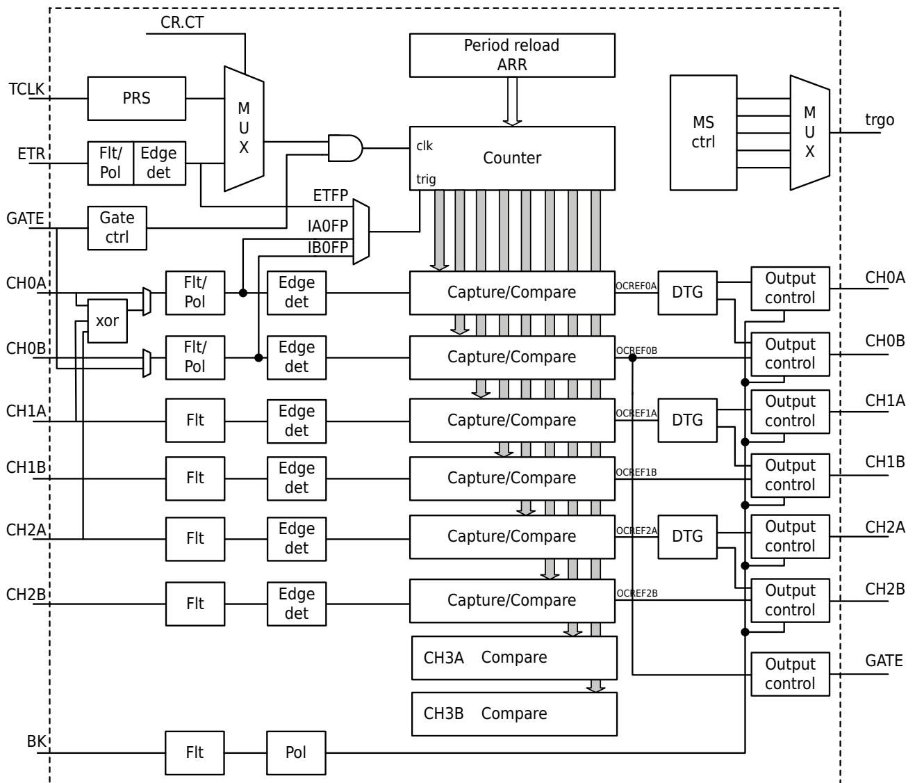
Figure 13-2 ATIM3 Block Diagram
