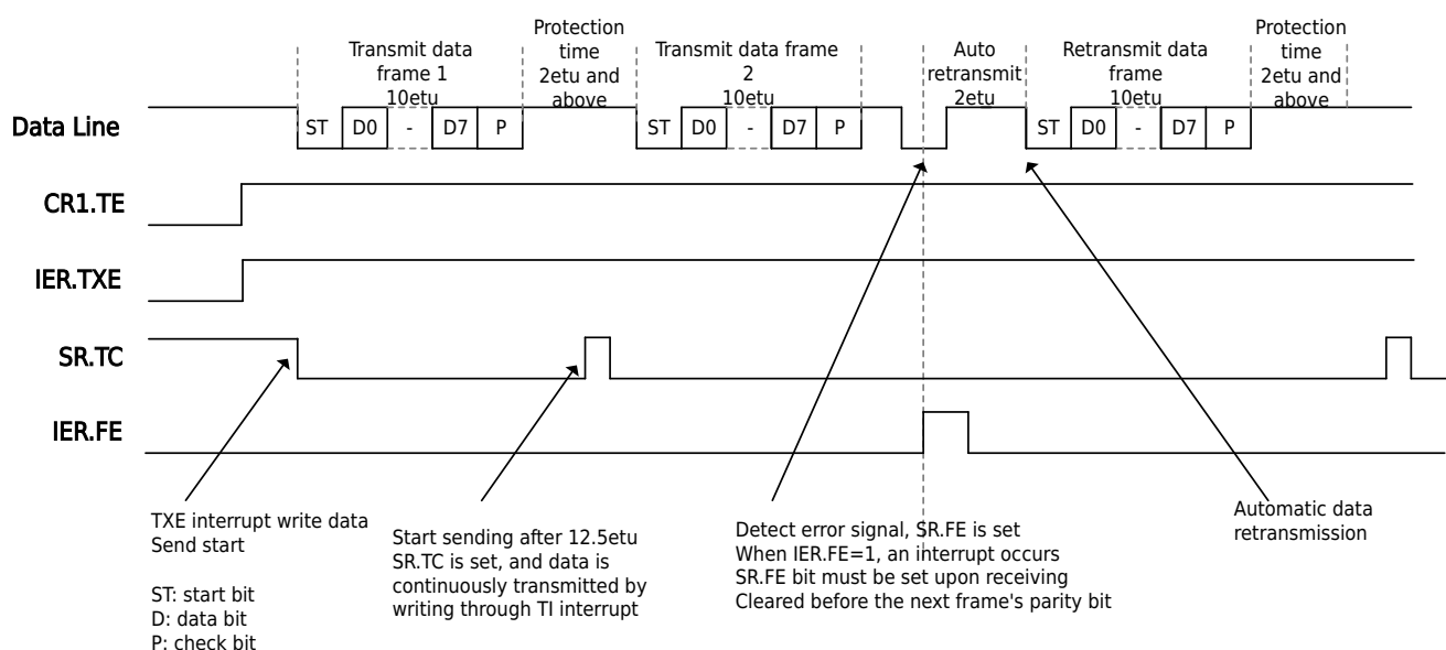
Figure 19-19 Smart Card Mode Transmit Data Legend
