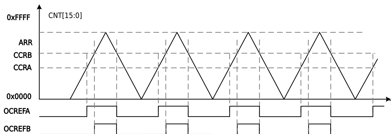
Figure 13-37 Triangular Counting Dual Point Comparison OCREF Output Waveform (OCMyx=0b111)
