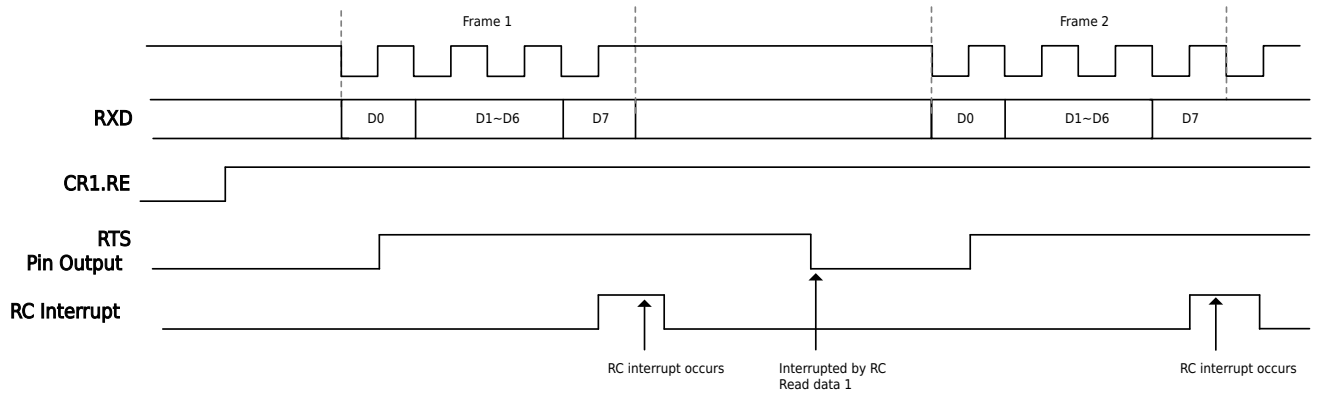
Figure 19-13 Synchronous Serial Port Mode Receiving Data Legend 2 (LSB/RTS Function)
