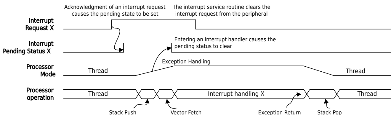
Figure 5-2 Interrupt Active and Pending States
