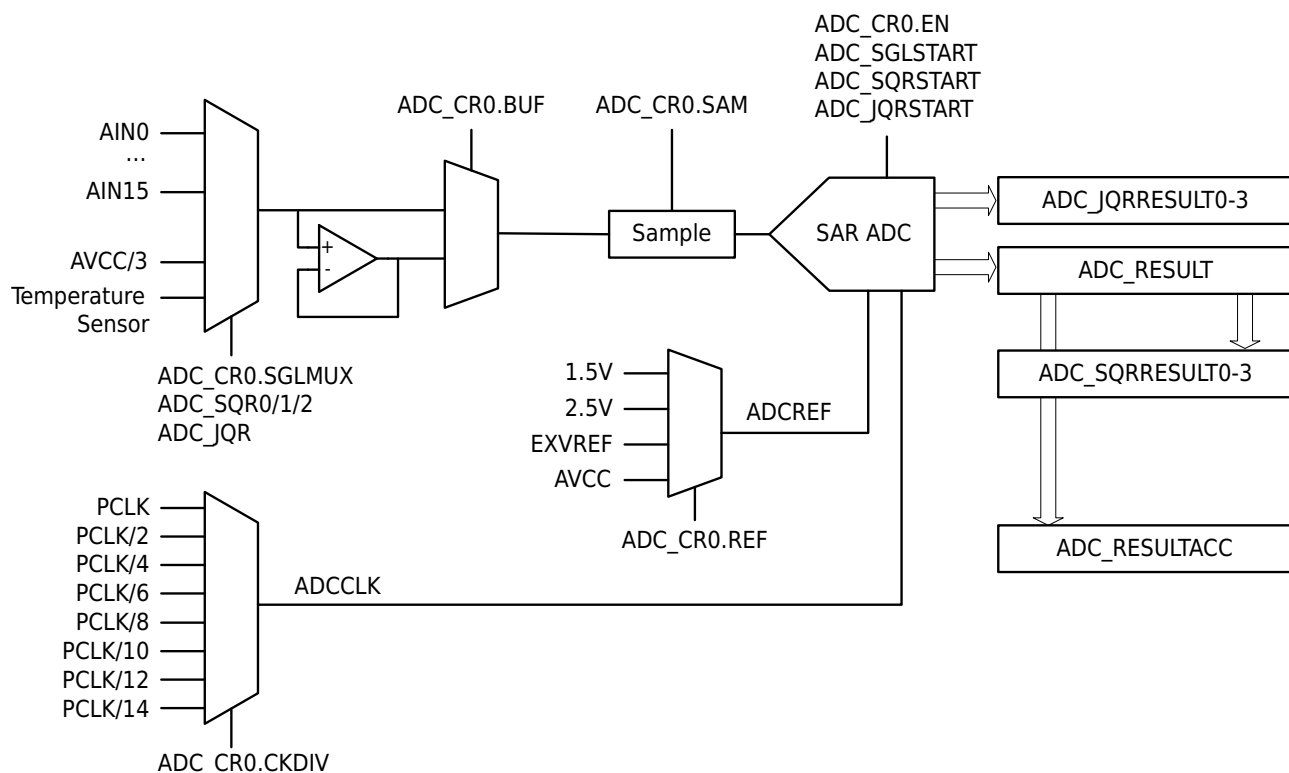
Figure 25-1 ADC Block Diagram
