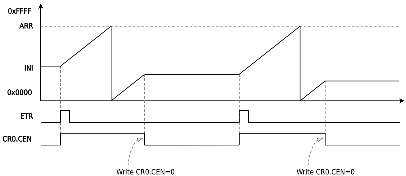
Figure 14-17 GTIM Trigger Start Mode Counting Diagram
