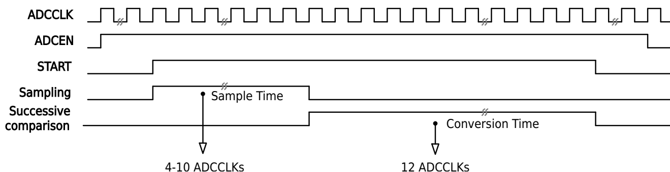
Figure 25-2 ADC Conversion Timing Diagram
