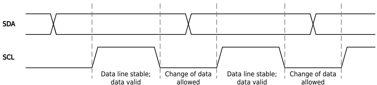
Figure 7-3 Bit Transfer on I2C Bus
