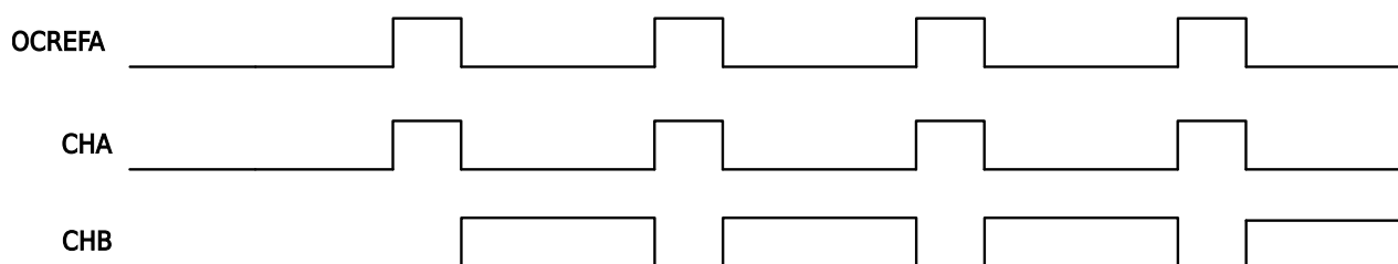
Figure 13-42 Complementary PWM Output Waveform
