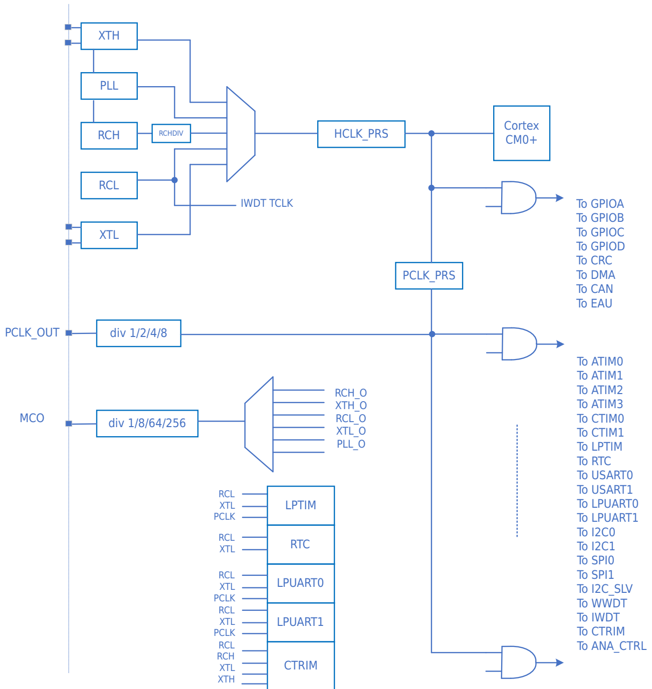
Figure 4-1 Clock Architecture Diagram
