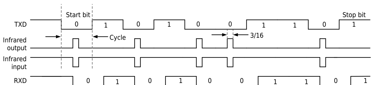
Figure 19-21 Infrared Data Modulation
