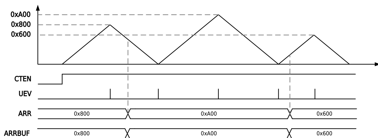
Figure 13-27 Mode 3 Triangular Wave Mode with Cache Invalid
