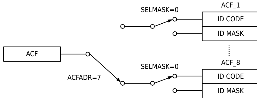
Figure 21-6 CAN ACF Register Access Filter Group Schematic Diagram
