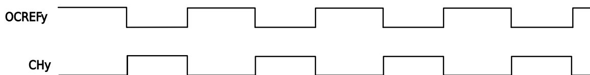
Figure 13-40 PWM Output Waveform When CCPy=1
