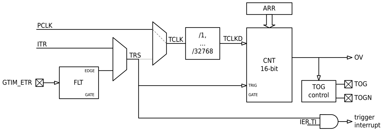
Figure 14-16 GTIM Trigger Start Mode Block Diagram
