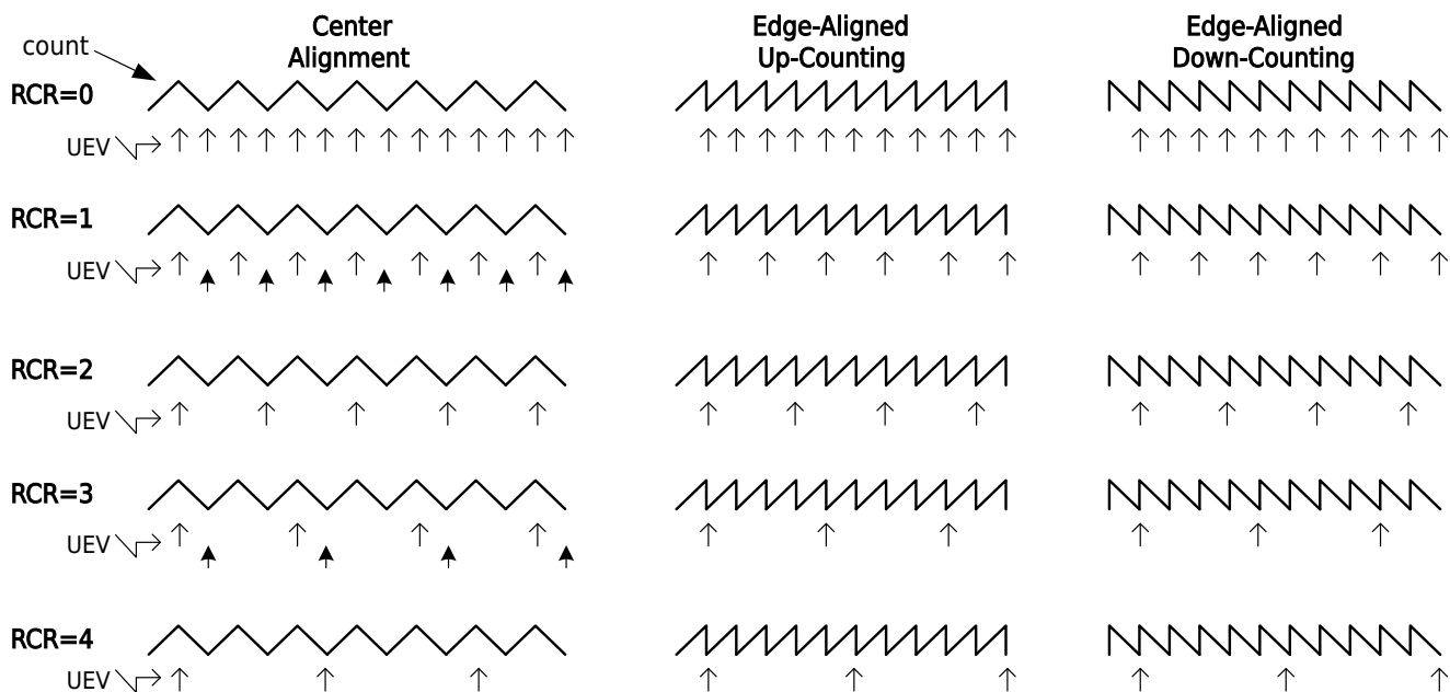
Figure 13-23 Repetition Counter Generates Update Timing ( RCR.OV=0 , RCR.UD=0 )
