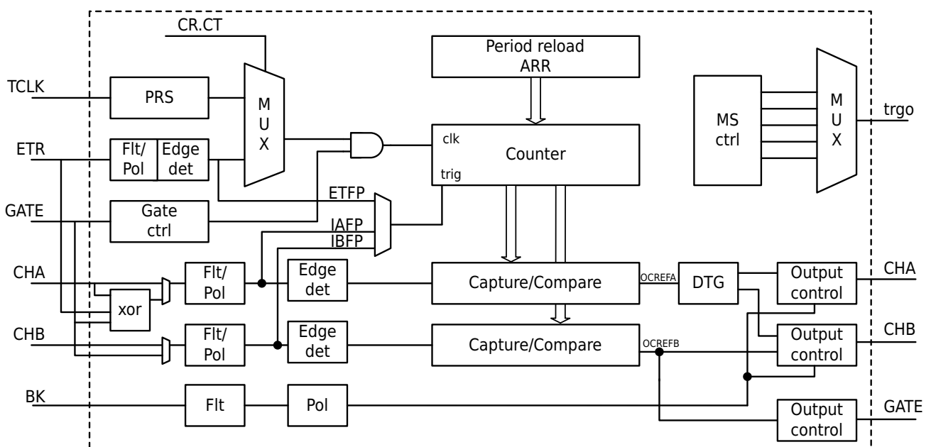
Figure 13-1 ATIM0/1/2 Block Diagram
