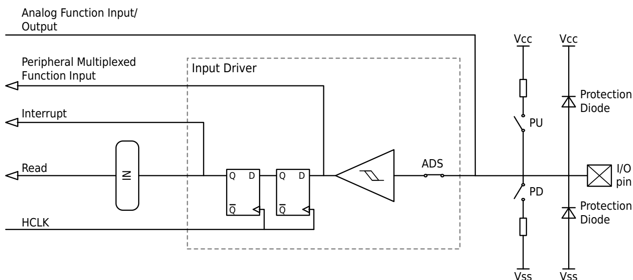
Figure 6-4 Input Floating/Pull-up/Pull-down Configuration Diagram
