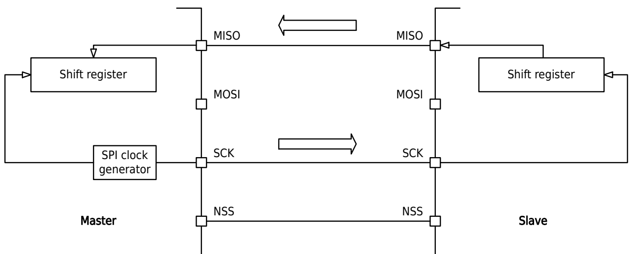
Figure 8-7 SPI Simplex Receive Communication Diagram
