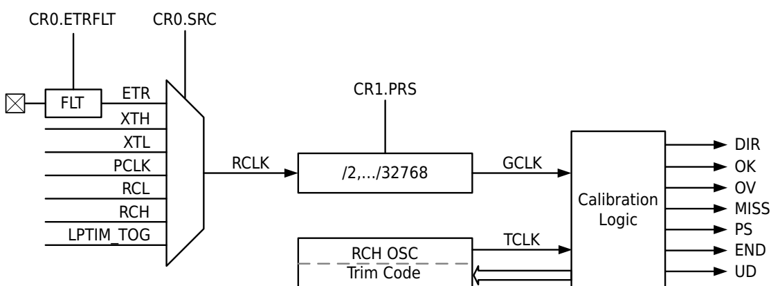
Figure 9-1 RCH Clock Calibration Operational Block Diagram
