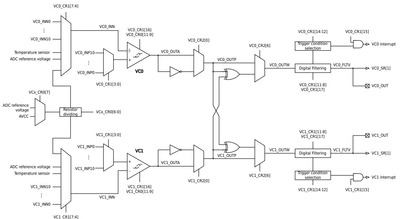
Figure 26-1 VC Function Block Diagram
