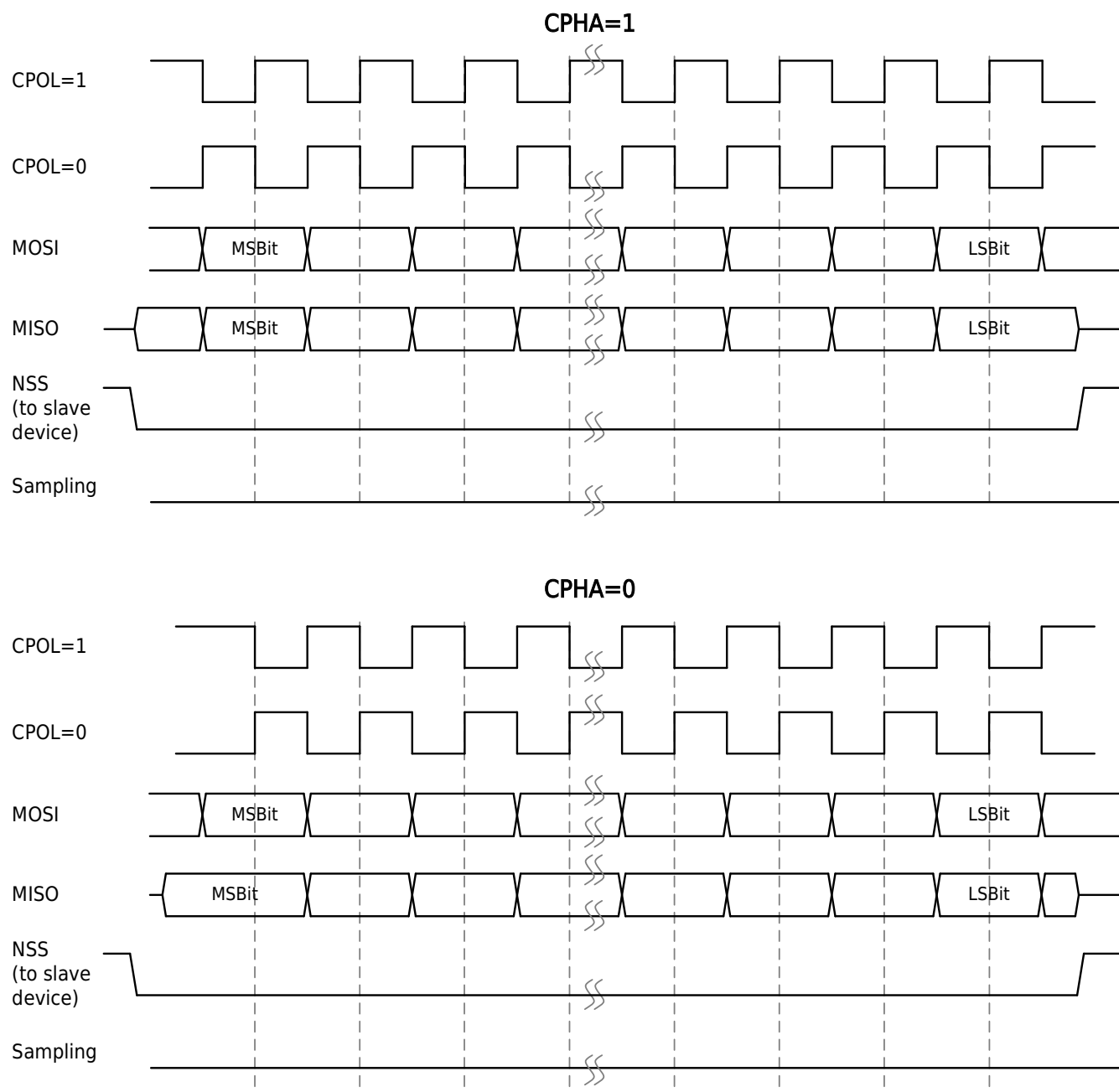
Figure 8-2 SPI Communication Format Timing Diagram
