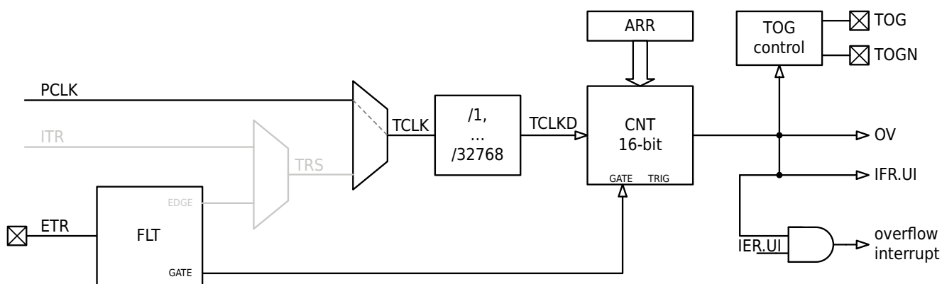
Figure 14-8 BTIM Gating Mode Block Diagram
