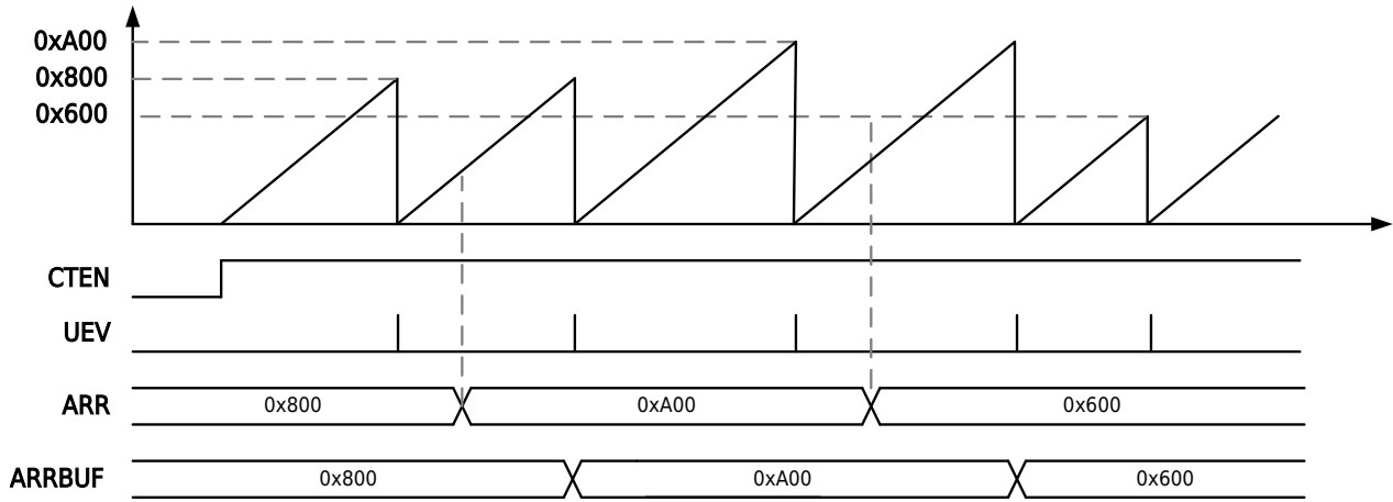
Figure 13-28 Mode 2 Sawtooth Wave Mode Up-Counting with Cache Enable
