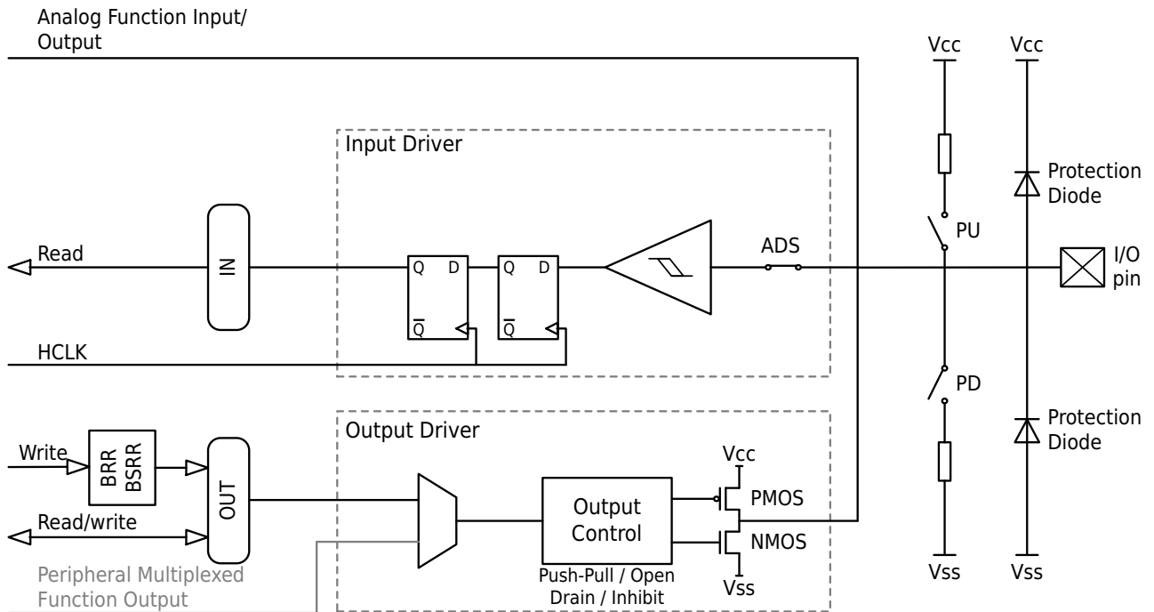
Figure 6-6 Output Configuration Diagram
