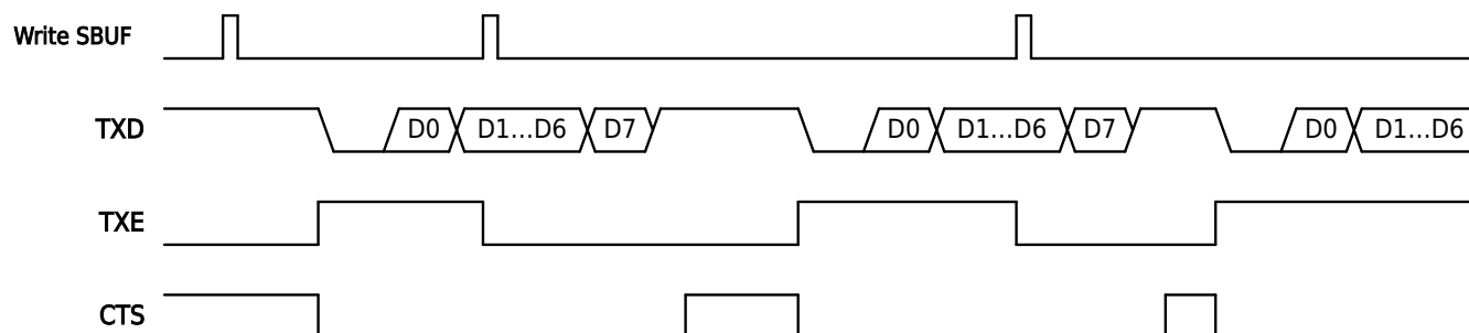
Figure 20-10 CTS Hardware Flow Control Signal
