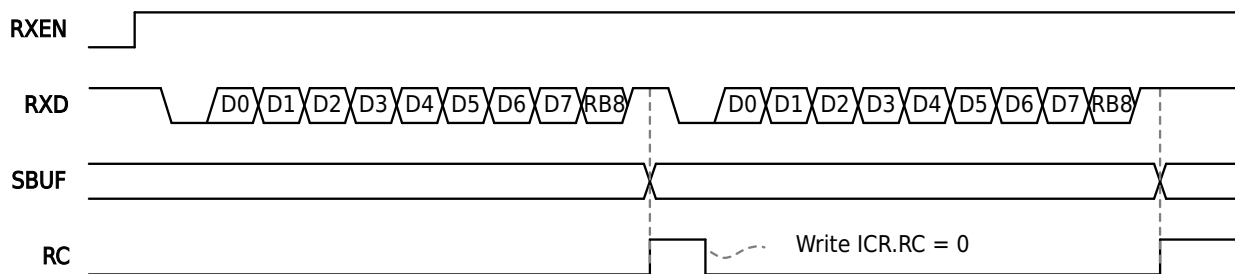
Figure 20-7 Mode2/Mode3 Data Receiving
