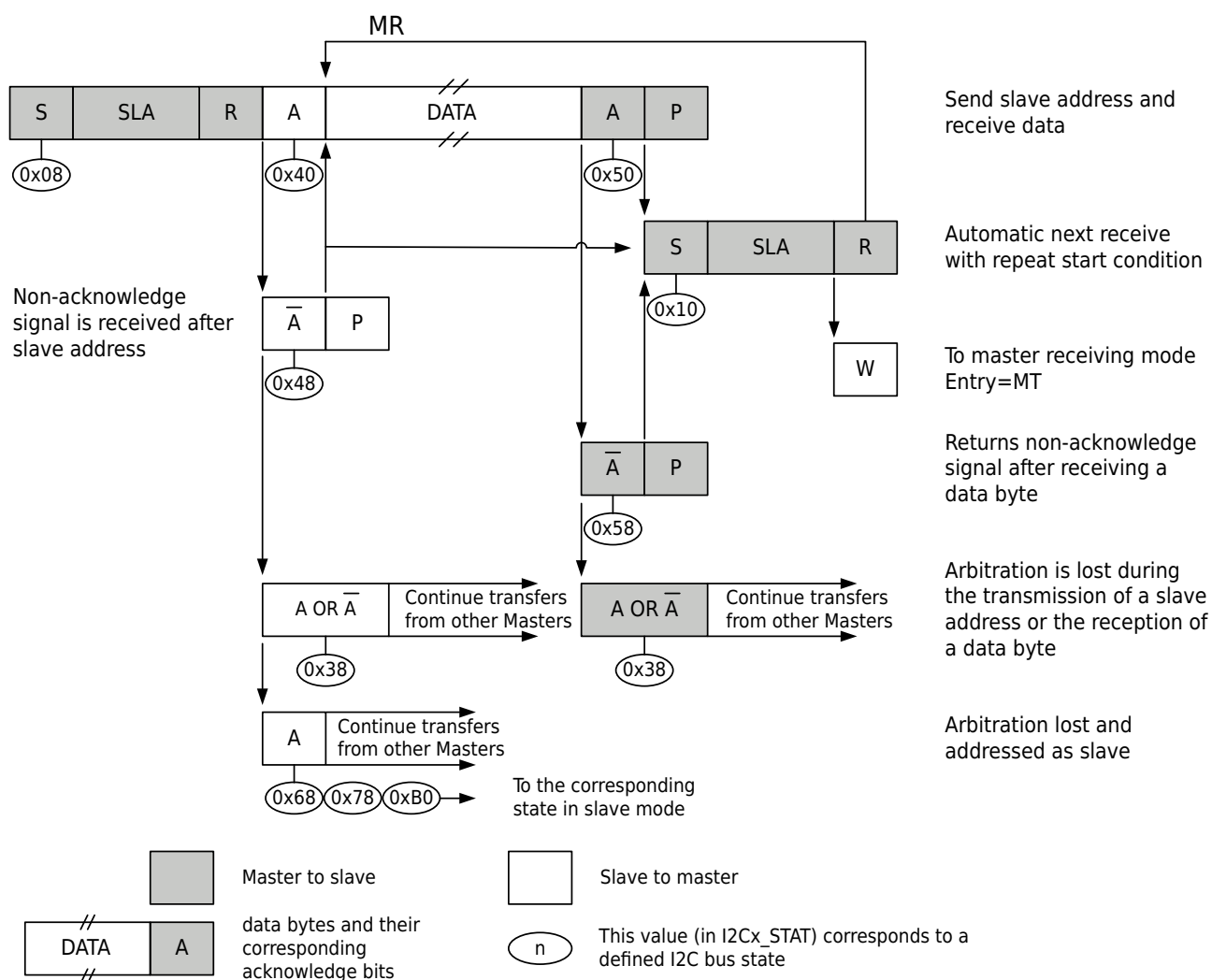
Figure 7-10 I2C Master Receiving State Diagram
