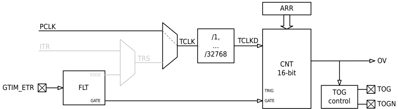
Figure 14-18 GTIM Gating Mode Block Diagram
