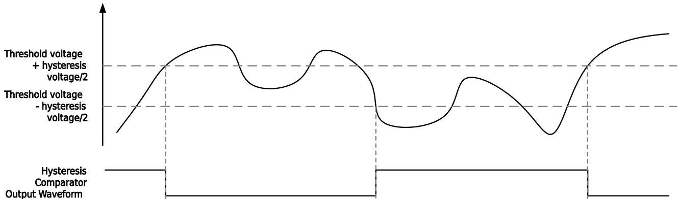
Figure 27-3 LVD Hysteresis Response
