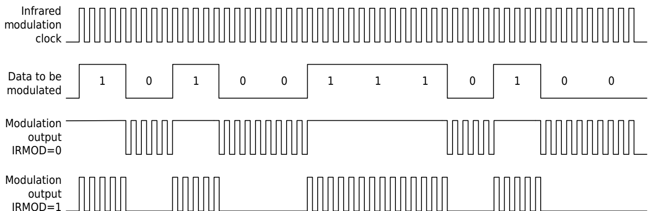
Figure 19-22 38K Infrared Modulation
