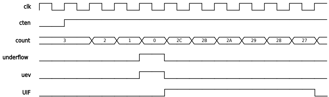
Figure 13-17 Mode 2 Compare Capture Mode Down-Counting Without Prescaler
