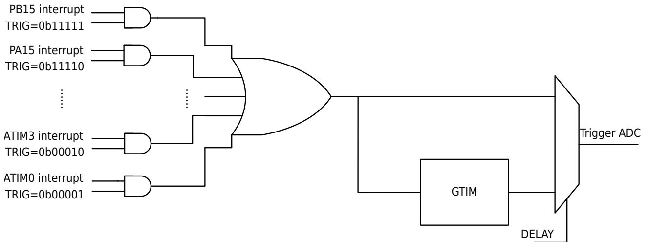
Figure 25-7 Diagram of External Trigger Sources for ADC JQR Scan Conversion
