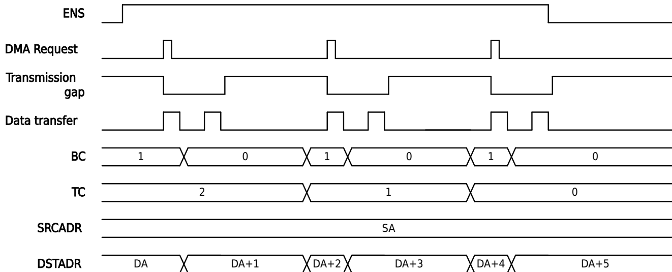
Figure 12-4 DMA Hardware Block Transfer Mode
