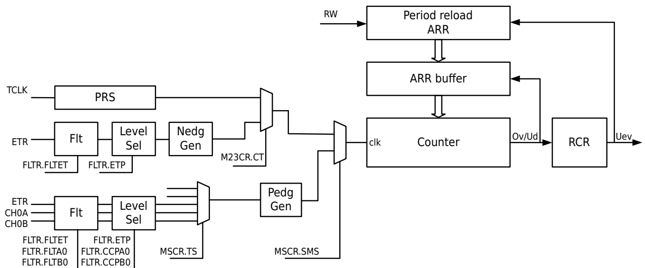
Figure 13-14 Mode 2/3 Compare Capture Mode Counter Block Diagram
