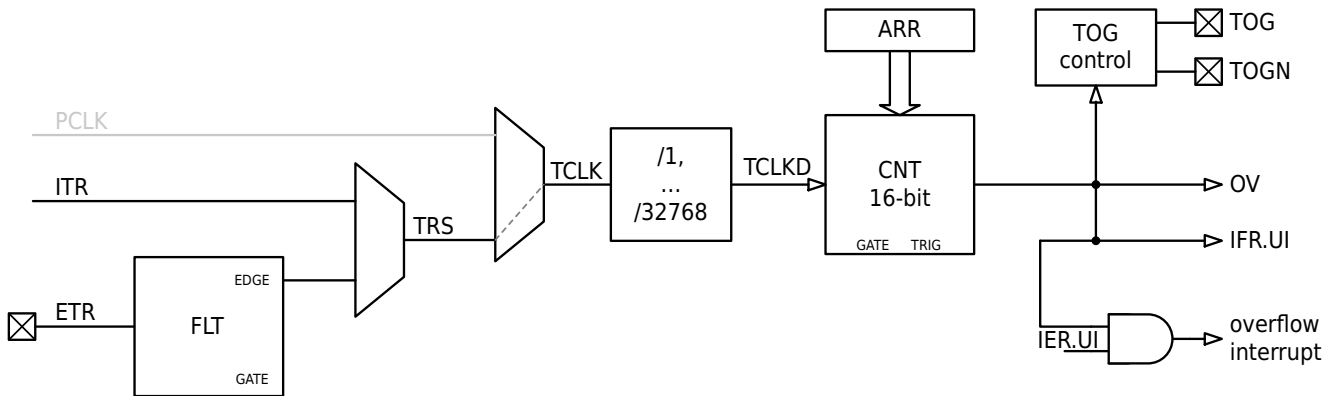
Figure 14-5 BTIM Counter Mode Block Diagram
