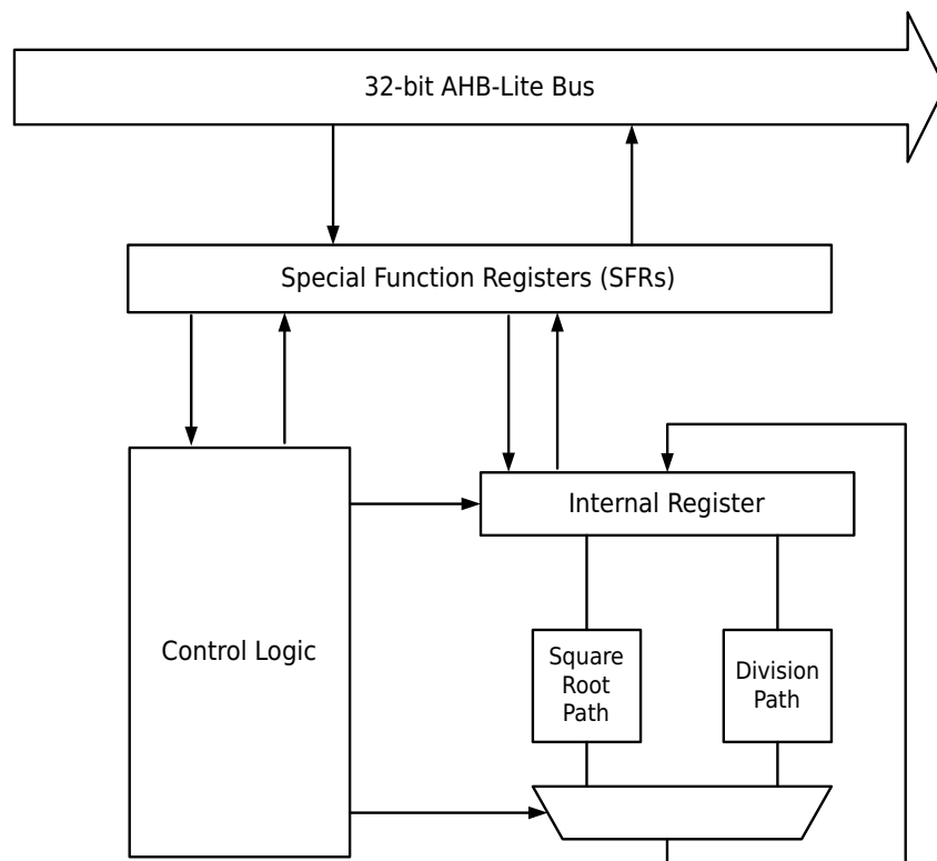
Figure 24-1 EAU Block Diagram
