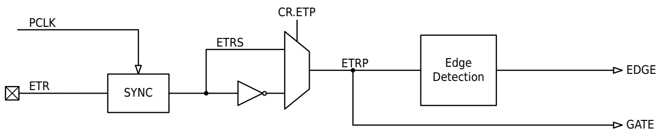
Figure 14-2 BTIM Filter Unit Diagram
