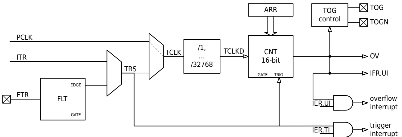
Figure 14-6 BTIM Trigger Start Mode Block Diagram
