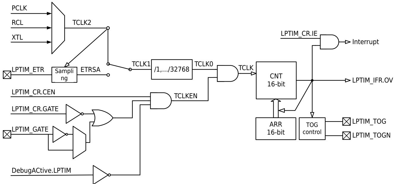
Figure 15-2 Low Power Timer Mode 2
