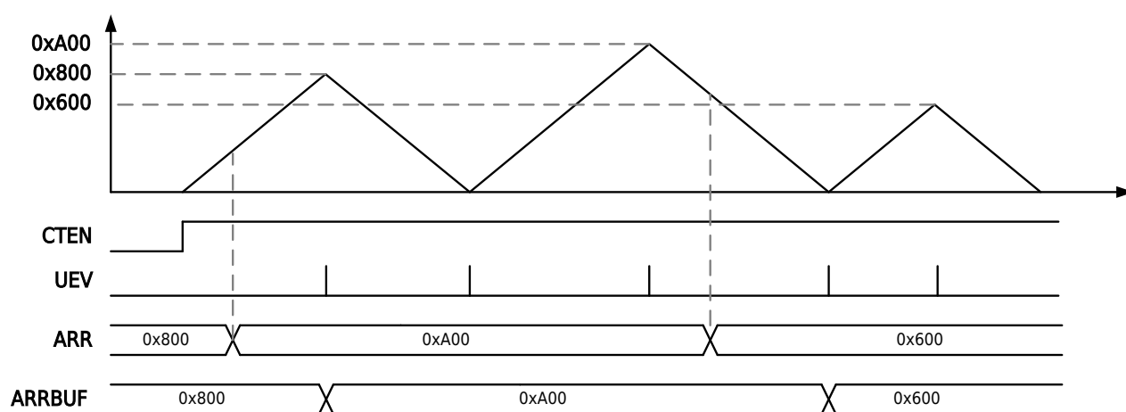
Figure 13-26 Mode 3 Triangular Wave Mode with Cache Enable
