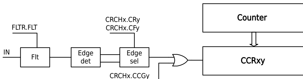
Figure 13-49 Capture Function Block Diagram
