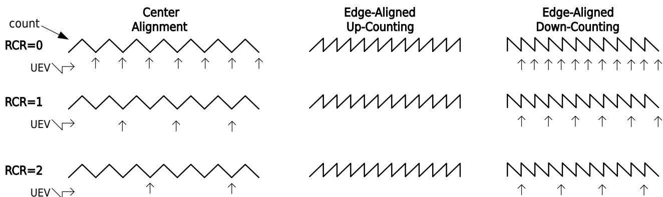
Figure 13-24 Update Timing Generated by Repetition Counter when Overflow Is Masked ( RCR.OV=1 , RCR.UD=0 )
