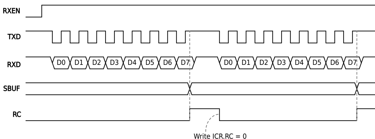
Figure 20-3 Mode0 Data Receiving
