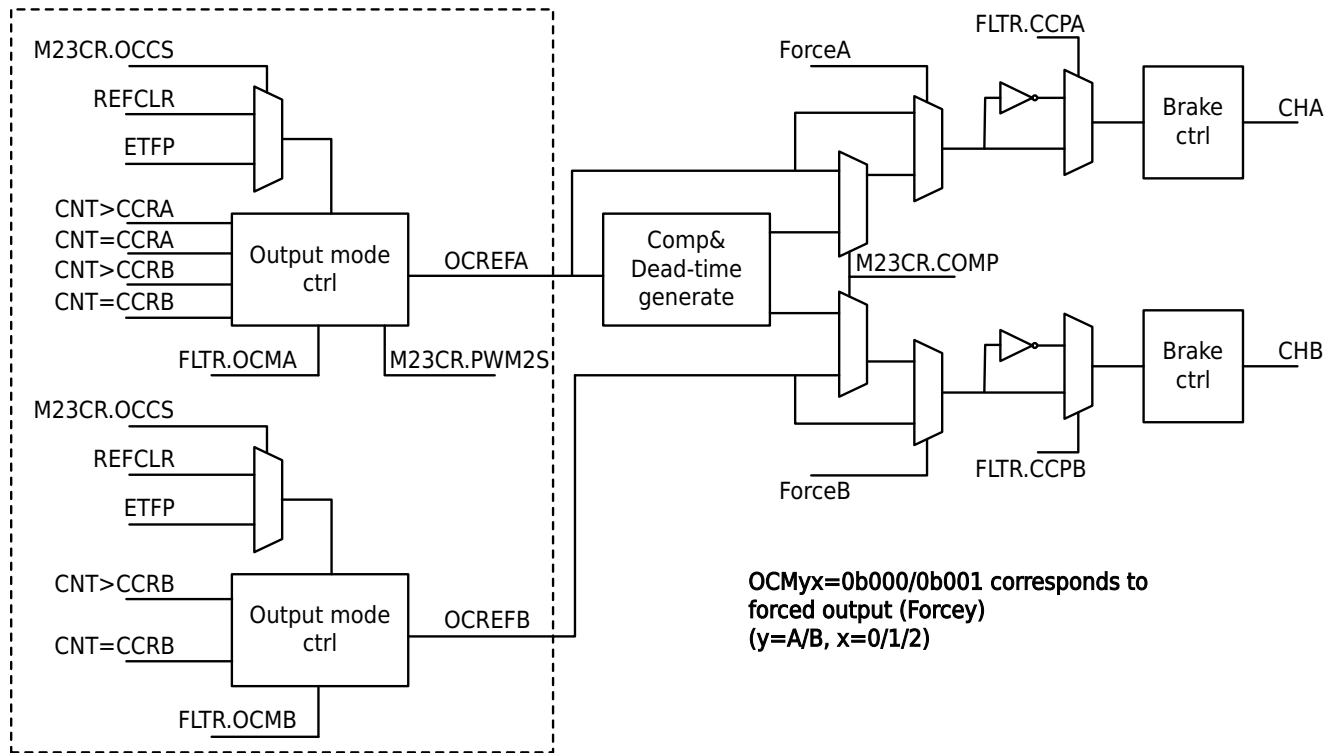
Figure 13-33 OCREF Output Block Diagram
