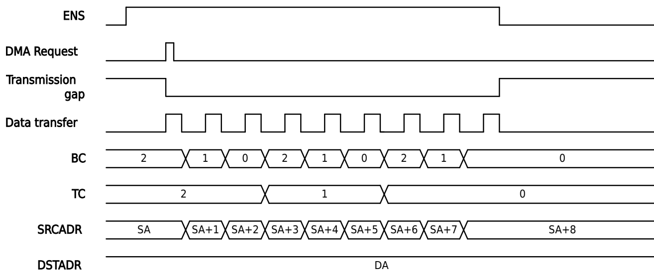
Figure 12-5 DMA Hardware Burst Transfer Mode
