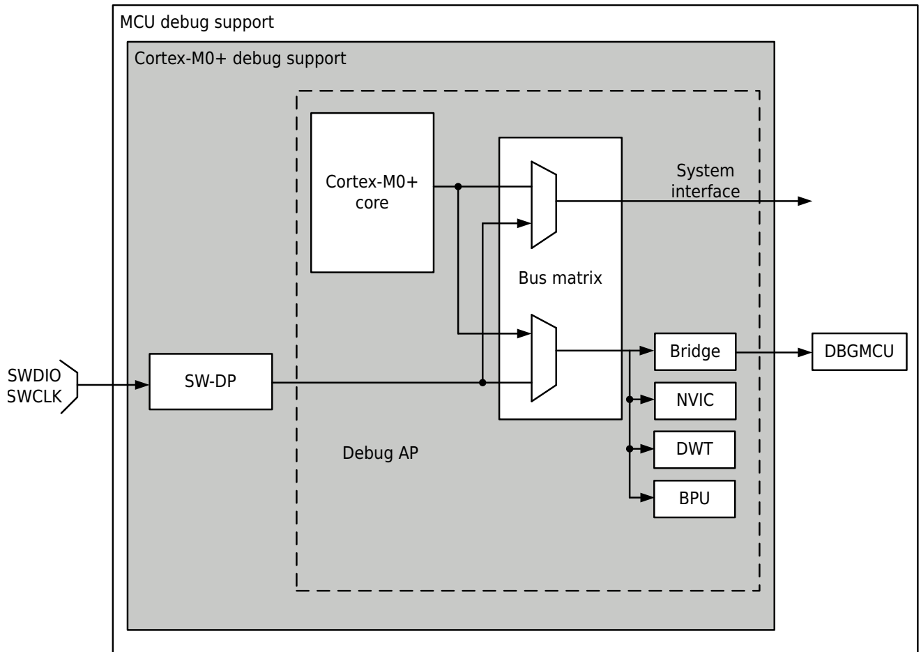
Figure 29-1 Debug Support Block Diagram
