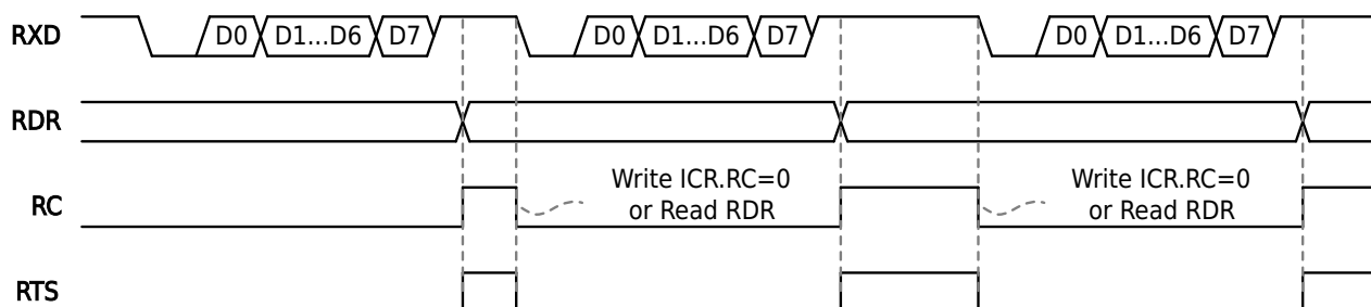
Figure 19-3 RTS Hardware Flow Control Signal
