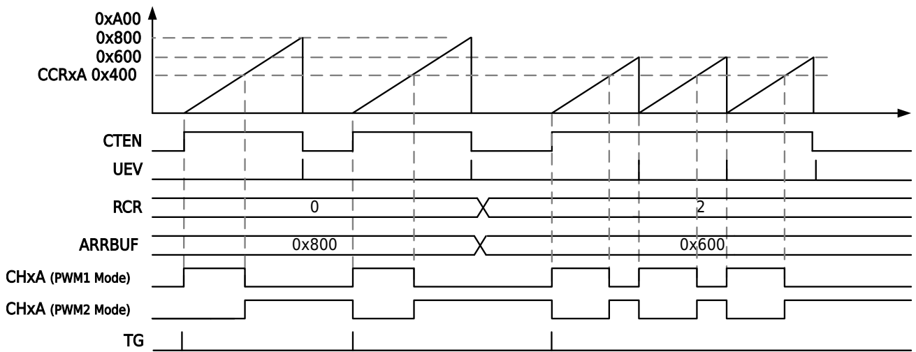
Figure 13-46 Sawtooth Up-Counting Single Pulse Mode
