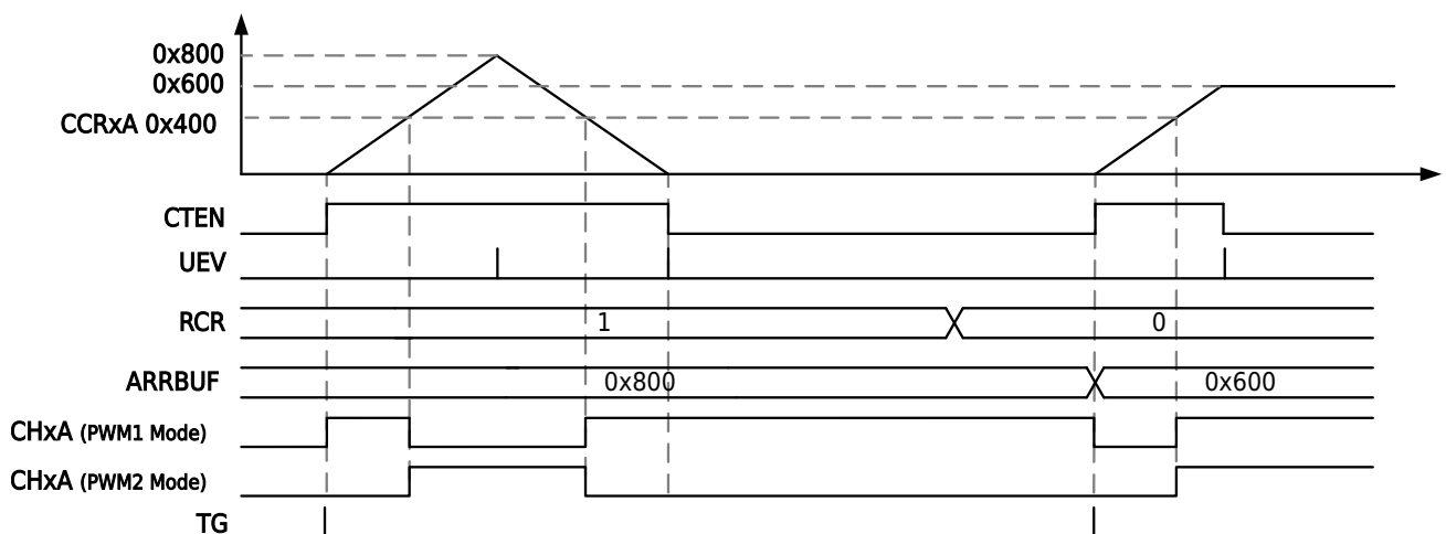
Figure 13-45 Triangular Wave Mode Single Pulse Counting
