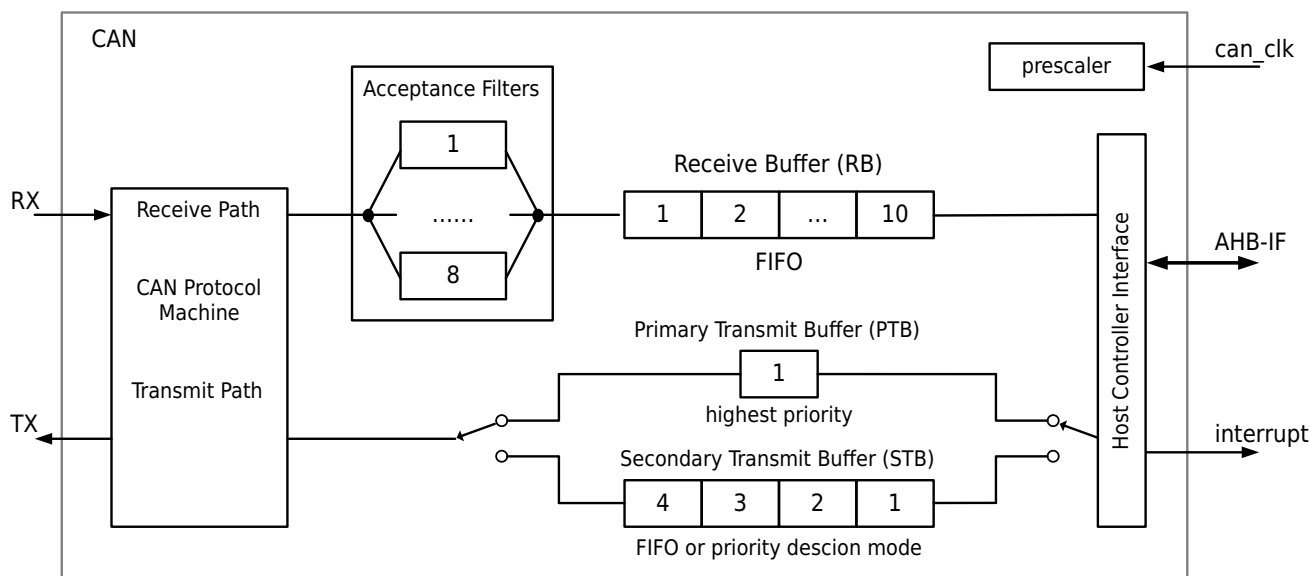
Figure 21-1 CAN System Block Diagram
