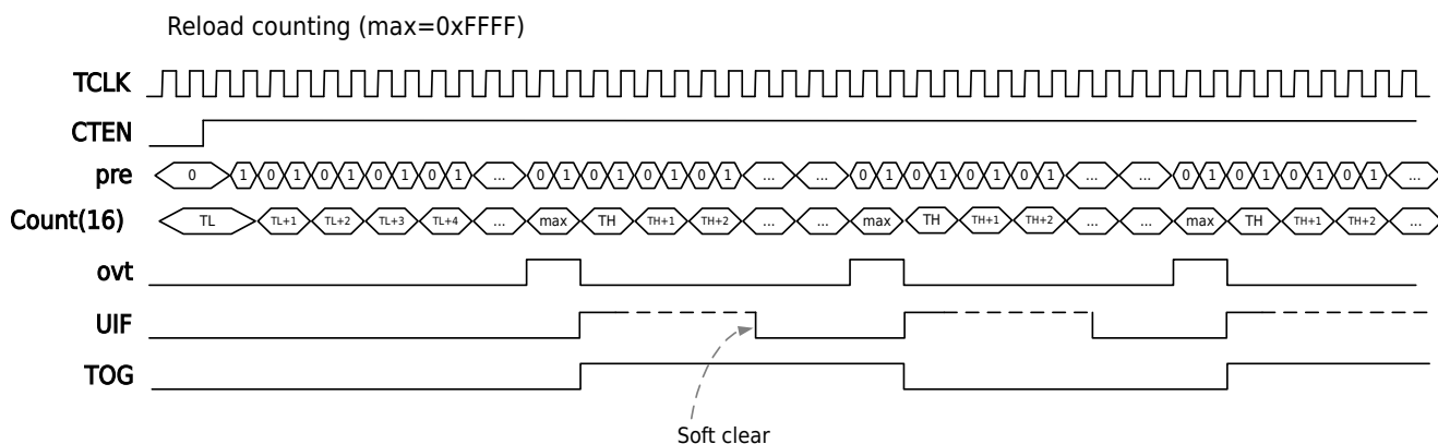
Figure 13-8 Mode0 Count Timer Reload Counting Timing Diagram (Prescaler=2)
