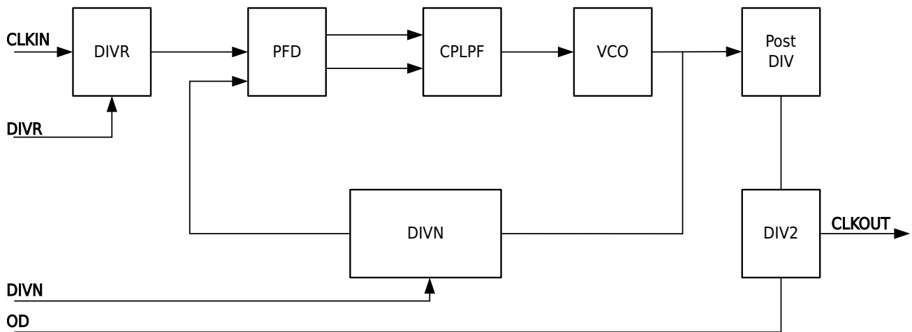
Figure 4-2 PLL System Block Diagram
