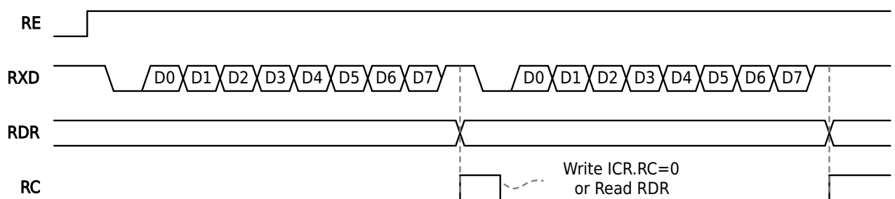
Figure 19-7 Receive Data Example
