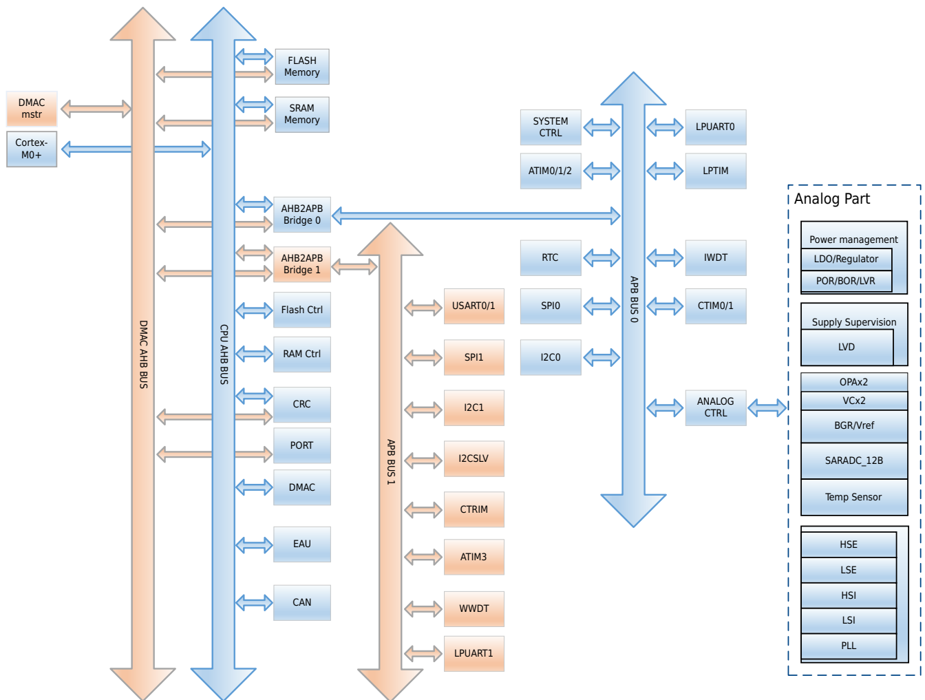
Figure 2-1 System Architecture Schematic Diagram
