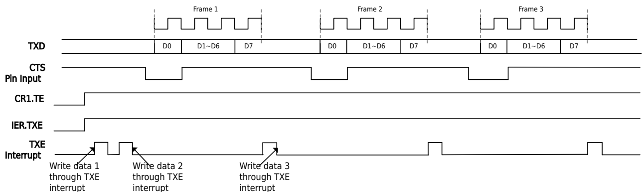
Figure 19-11 Synchronous Serial Port Mode to Send Data Legend 2 (LSB/CTS Function)
