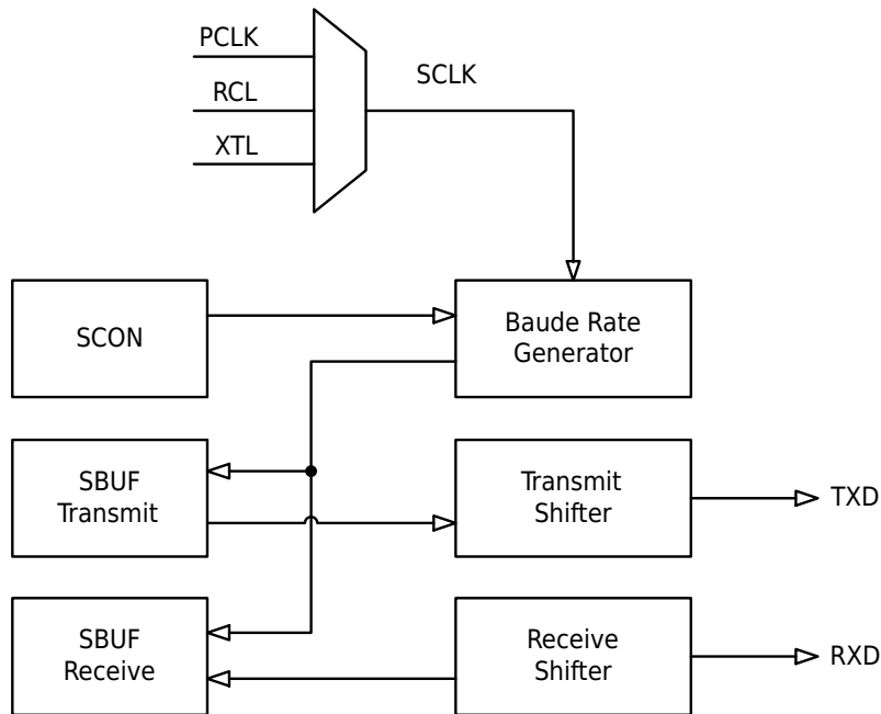
Figure 20-1 LPUART Function Block Diagram
