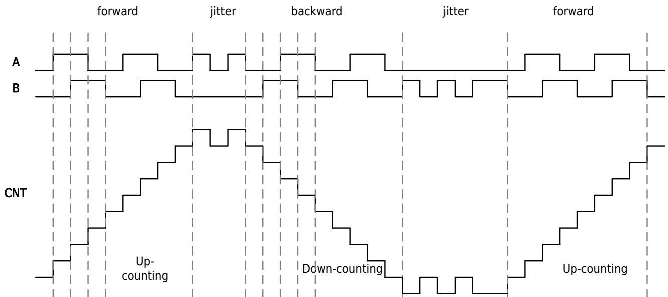
Figure 13-57 Quadrature Encoder Counting Mode3 Counting Diagram
