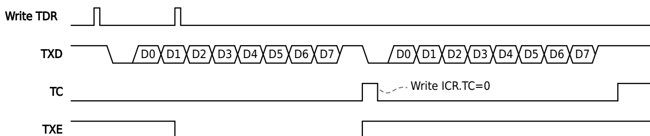
Figure 19-6 Transmit Data Example
