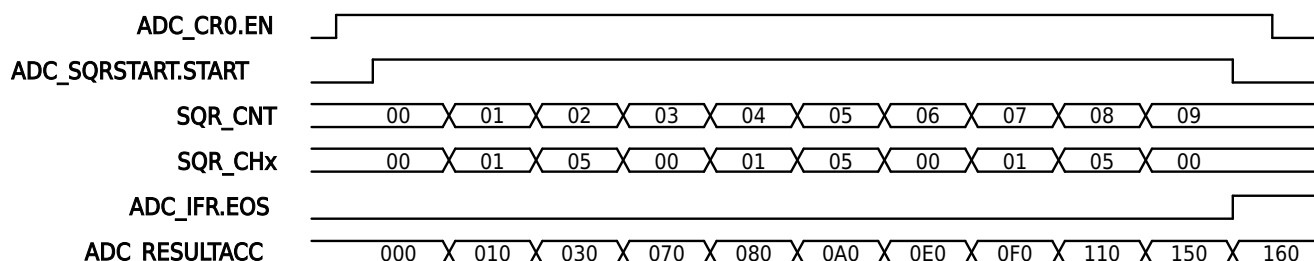
Figure 25-5 Examples of Continuous ADC Conversion Accumulation Process
