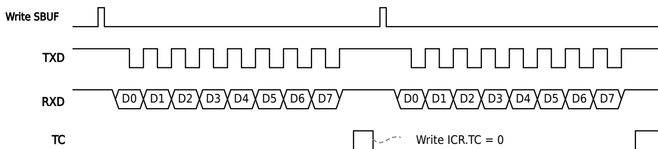
Figure 20-2 Mode0 Data Transmitting
