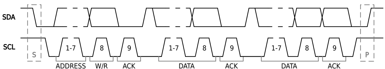
Figure 7-1 I2C Transmission Protocol
