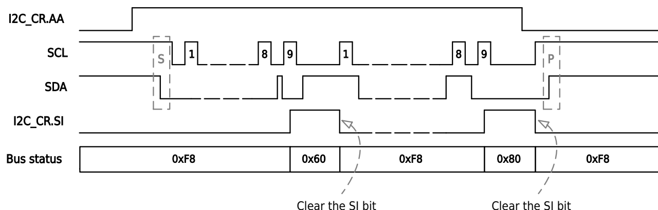
Figure 7-11 Slave Receiving Mode Data Synchronization Diagram
