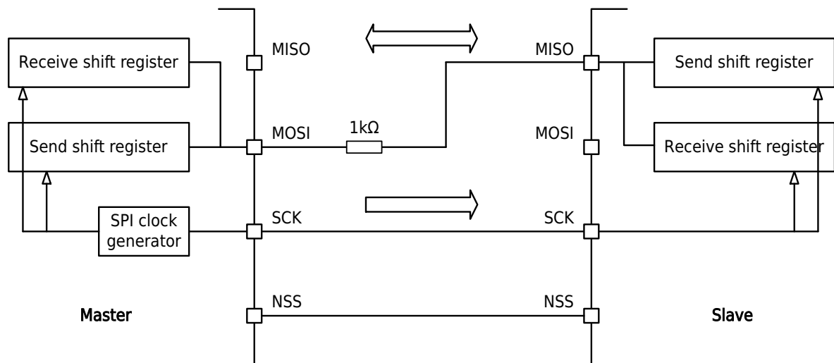
Figure 8-5 SPI Single-wire Half-duplex Communication
