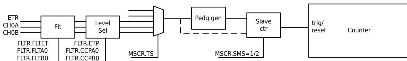
Figure 13-55 Mode2/3 Slave Mode Trigger and Reset Function
