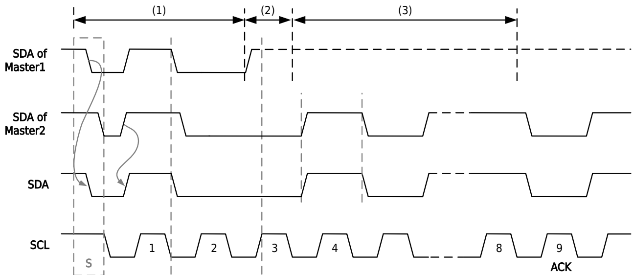
Figure 7-5 Arbitration on the I2C Bus
