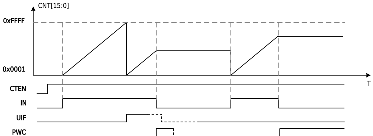
Figure 13-10 Model1: Pulse Width Measurement PWC High-Level Pulse Width Measurement
