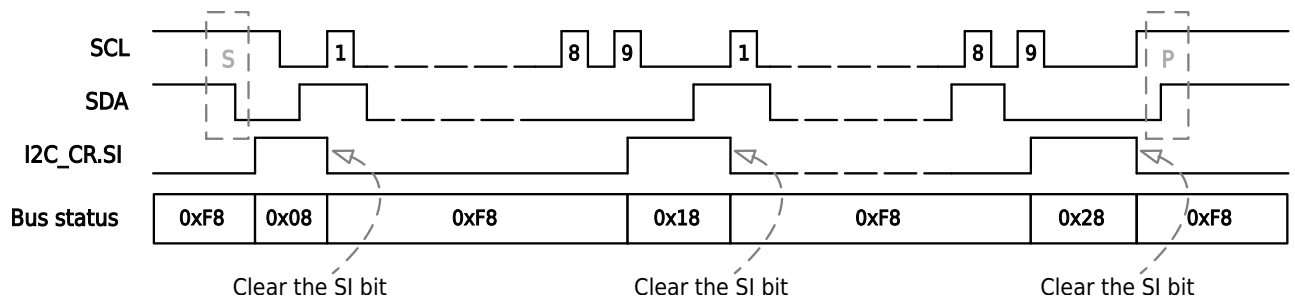
Figure 7-7 Data Synchronization Diagram of Master Sending Mode
