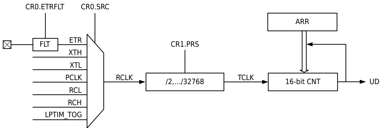
Figure 9-3 General Low Power Timer Scenario Operational Block Diagram
