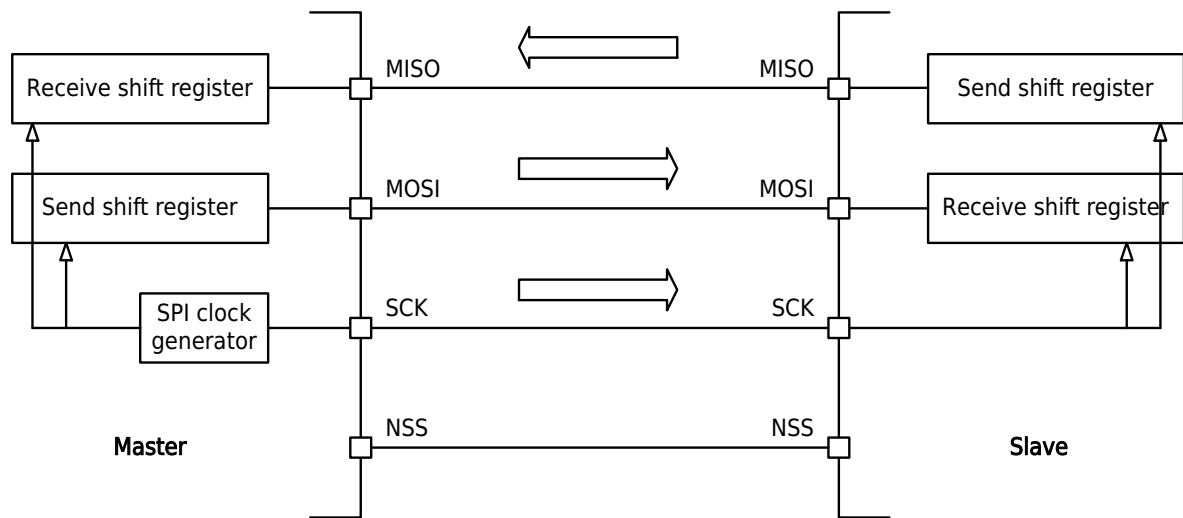
Figure 8-4 SPI Full-duplex Communication
