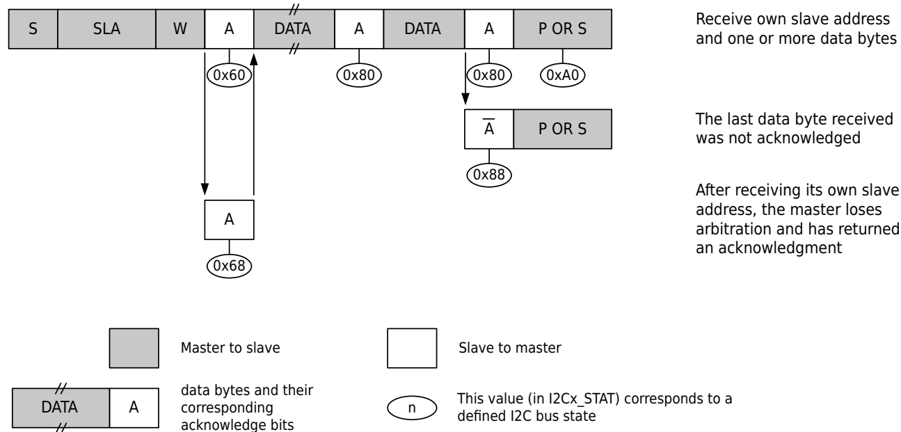
Figure 7-12 Slave Receiving State Diagram
