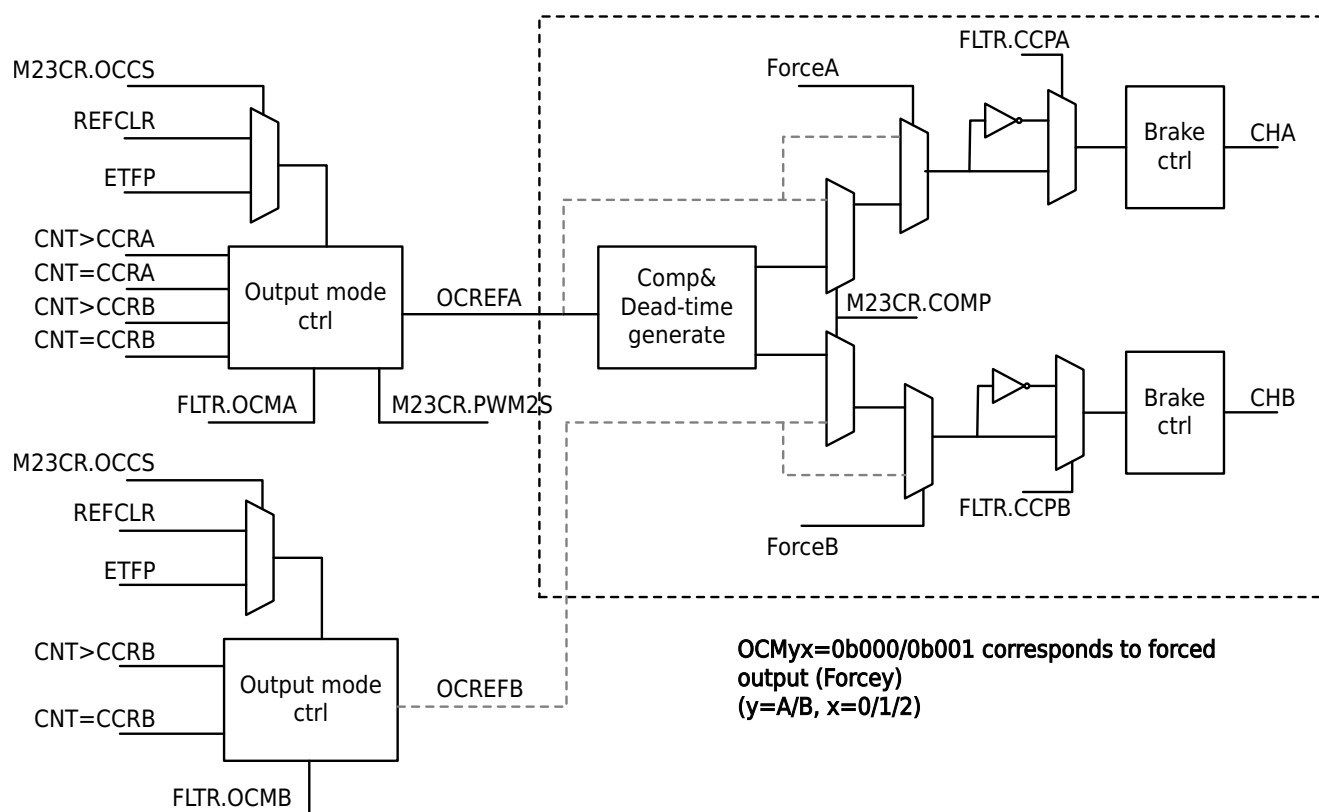
Figure 13-41 Complementary PWM Output Block Diagram
