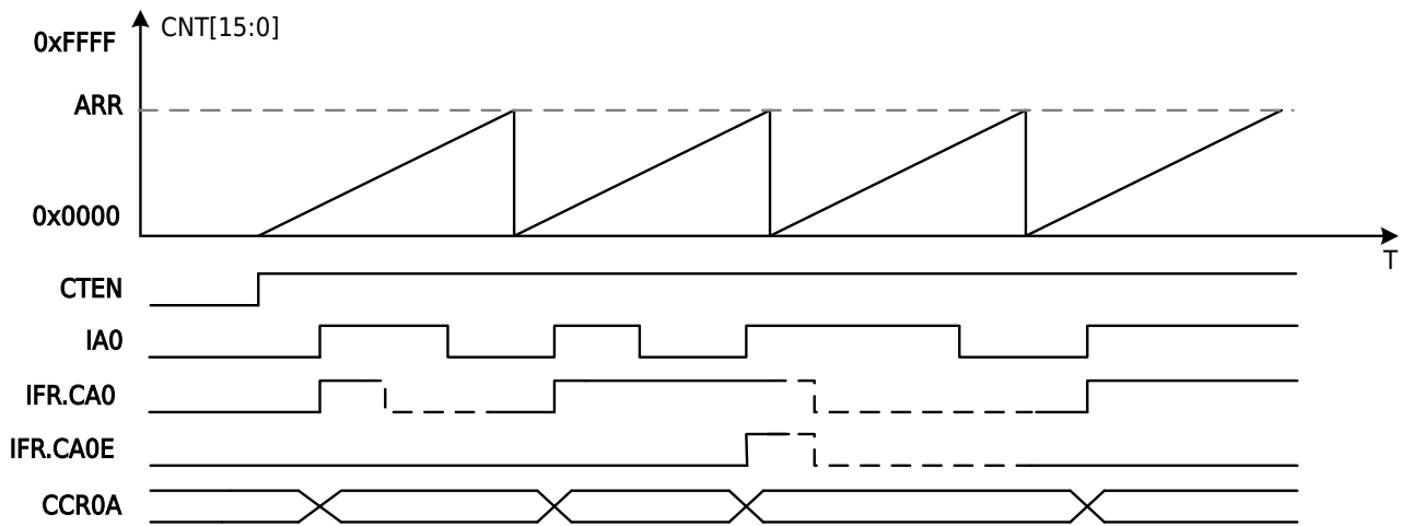
Figure 13-50 Capture Timing Diagram
