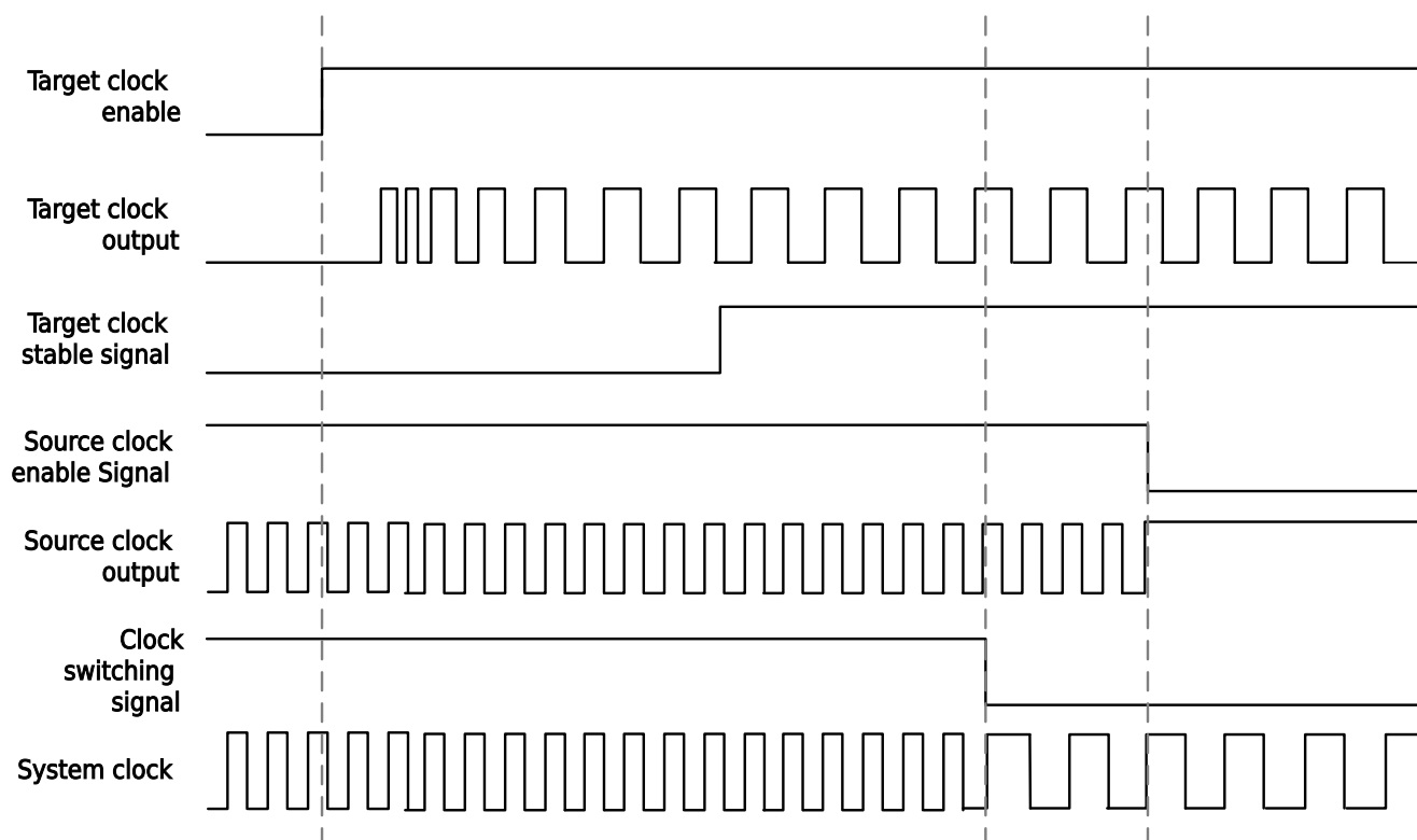
Figure 4-4 Clock Switching Diagram
