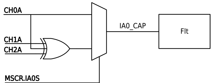
Figure 13-51 ATIM3 CH0A Capture Input Port Selection
