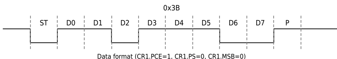
Figure 19-18 Smart Card Mode Data Format Example
