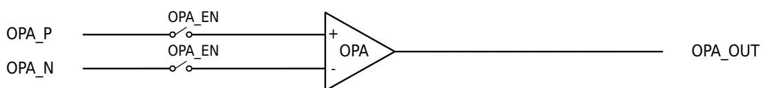
Figure 28-1 OPA Function Block Diagram
