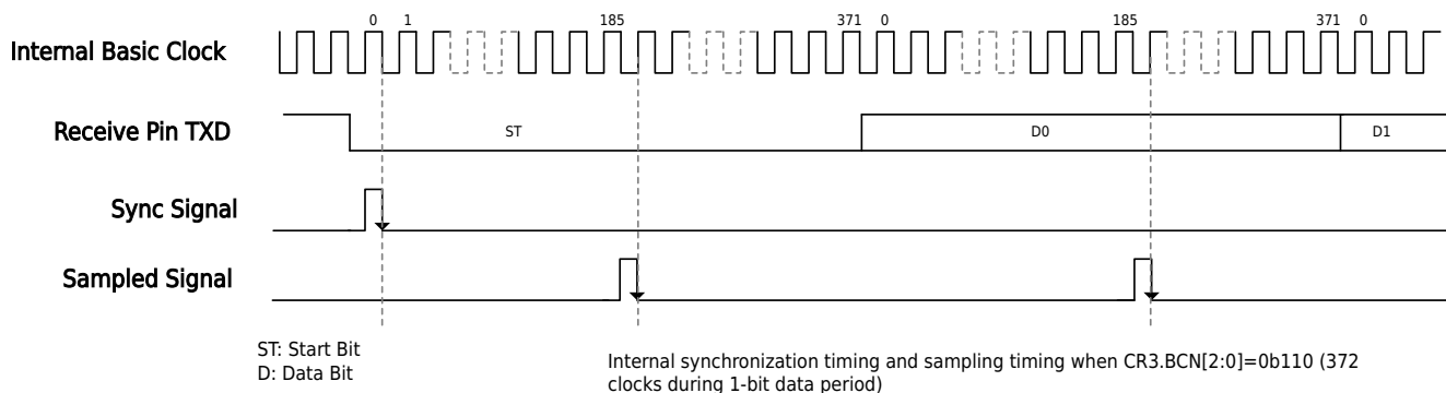
Figure 19-16 Smart Card Mode Internal Synchronization Timing and Sample Timing Diagram
