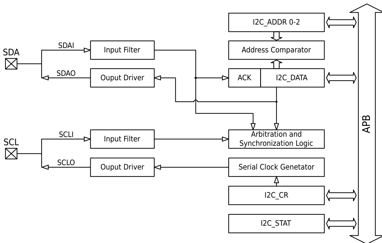
Figure 7-6 I2C Function Block Diagram
