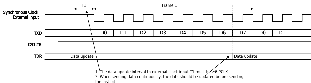
Figure 19-14 Precautions for Synchronous Serial Port Mode
