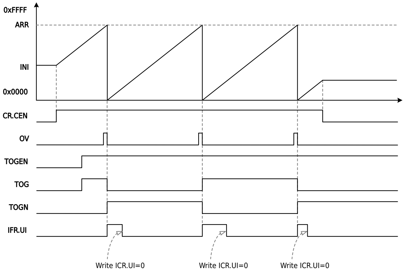
Figure 14-3 BTIM Counter Waveform
