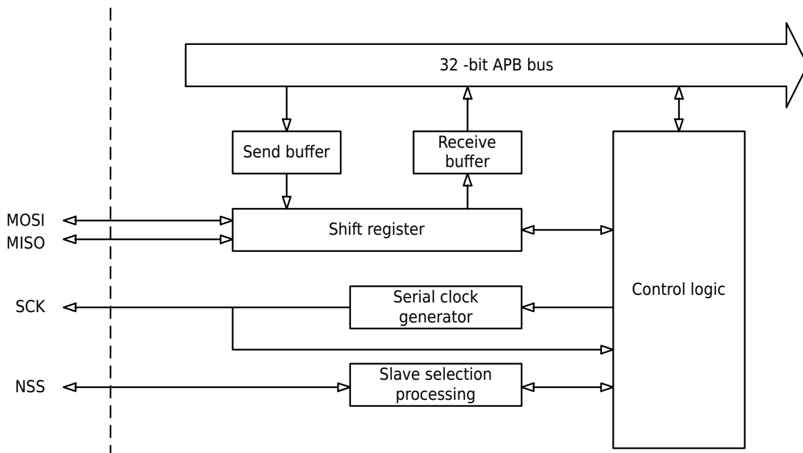
Figure 8-1 SPI Block Diagram
