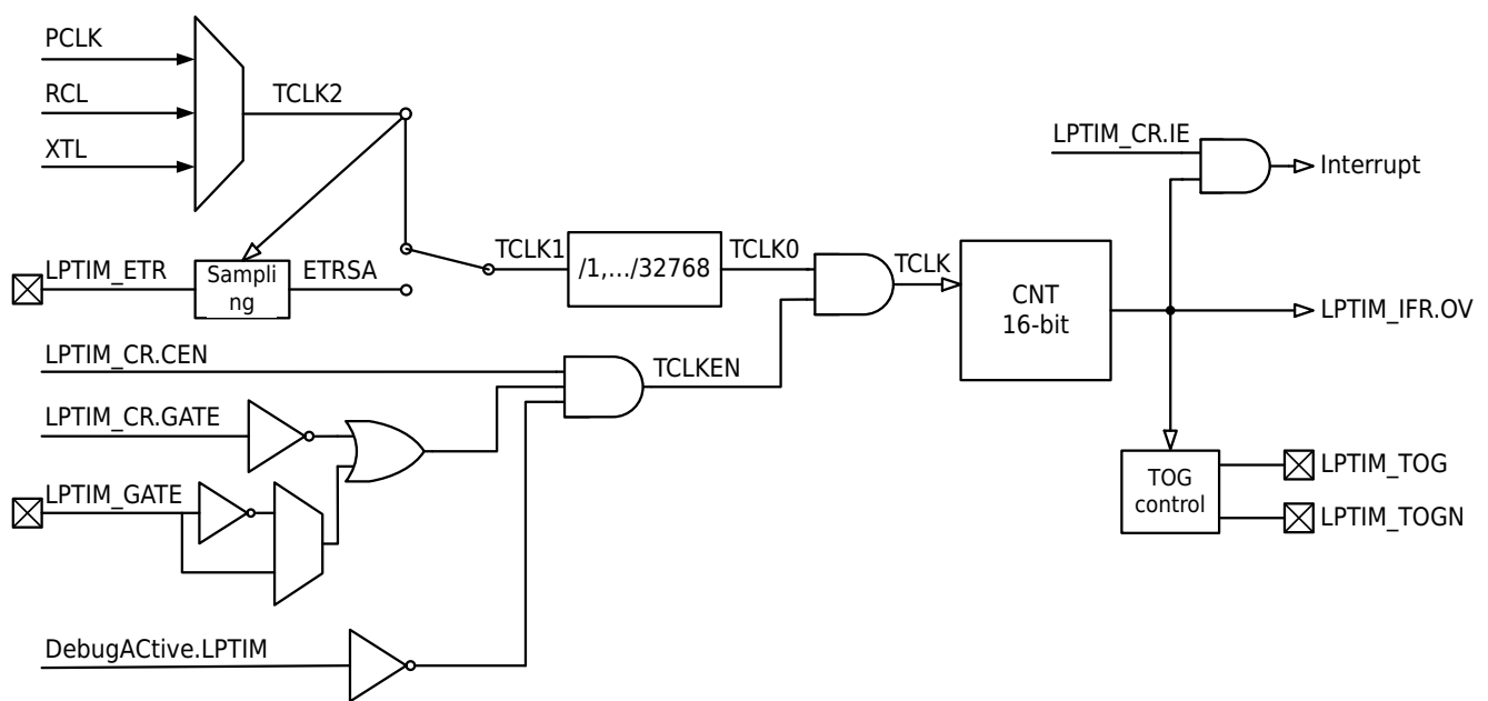
Figure 15-1 Low Power Timer Mode 1
