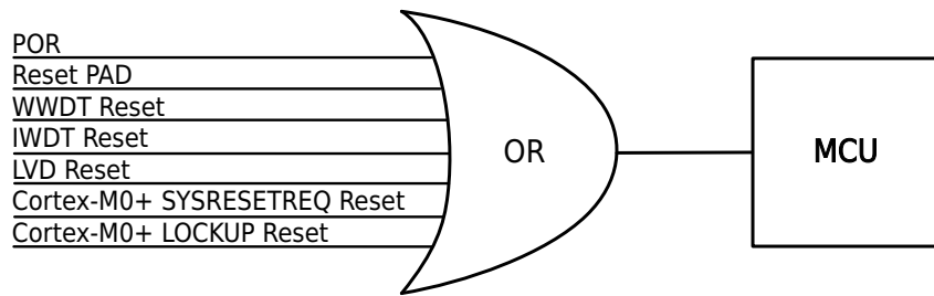
Figure 4-5 Reset Source Diagram
