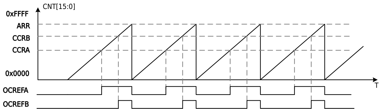
Figure 13-34 Sawtooth Counting Single Point Comparison OCREF Output Waveform (OCMyx=0b111)
