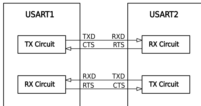
Figure 19-1 Asynchronous Serial Port Mode Hardware Flow Control Example
