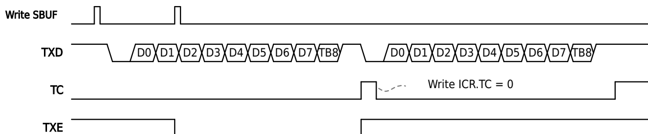
Figure 20-6 Mode2/Mode3 Data Transmitting
