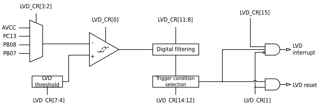
Figure 27-1 LVD Block Diagram
