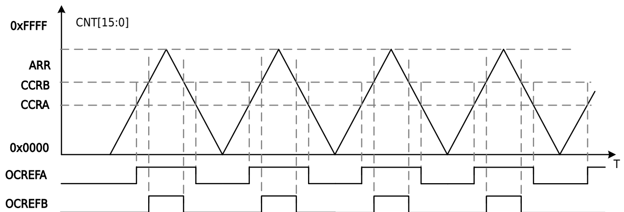
Figure 13-35 Triangular Counting Single Point Comparison OCREF Output Waveform (OCMyx=0b111)
