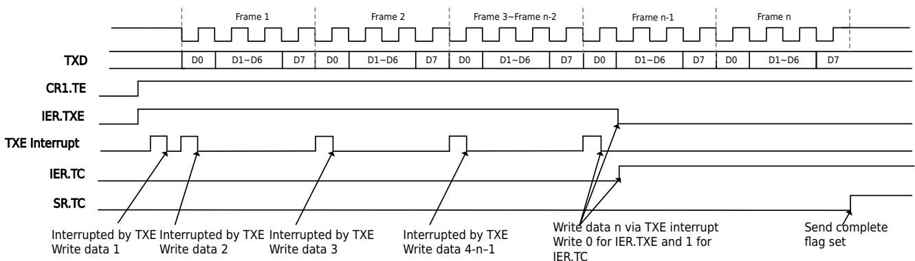
Figure 19-10 Synchronous Serial Port Mode Sending Data Legend 1 (LSB/No CTS Function)
