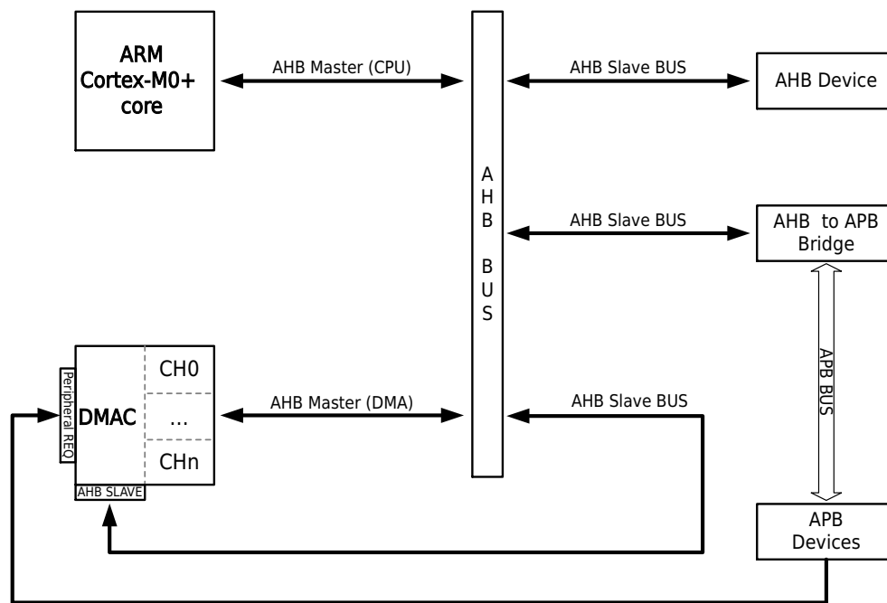
Figure 12-1 DMA Controller Functional Block Diagram
