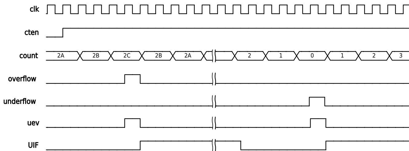
Figure 13-21 Mode3 Compare Capture Mode Up/Down-Counting with Prescaler
