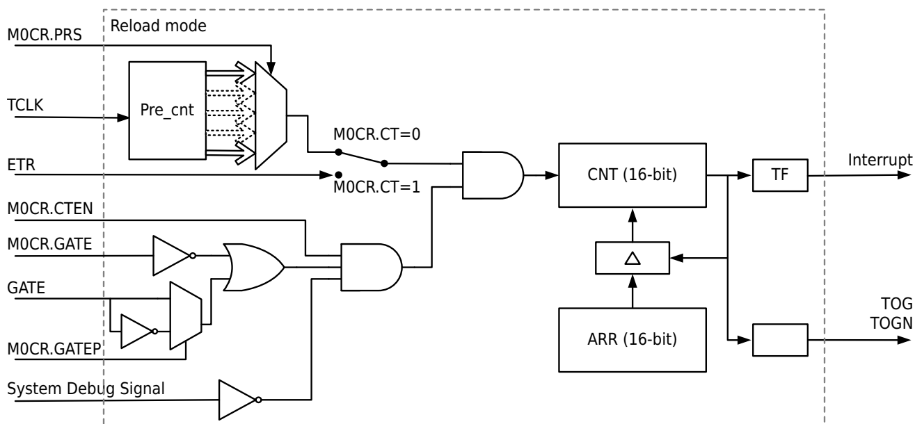
Figure 13-4 Mode0 Count Timer Reload Counting Block Diagram
