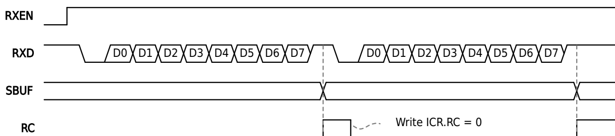
Figure 20-5 Mode1 Data Receiving
