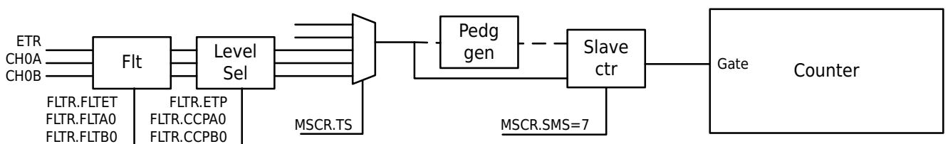
Figure 13-54 Mode2/3 Slave Mode Gating Function
