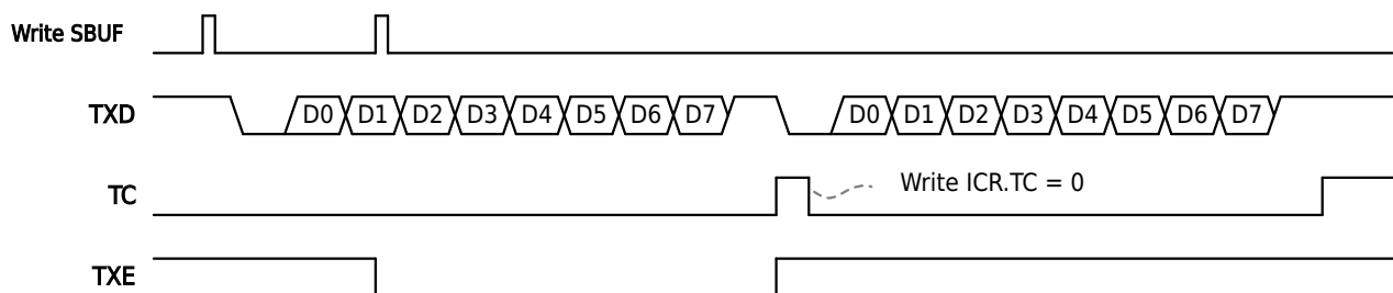
Figure 20-4 Mode1 Data Transmitting
