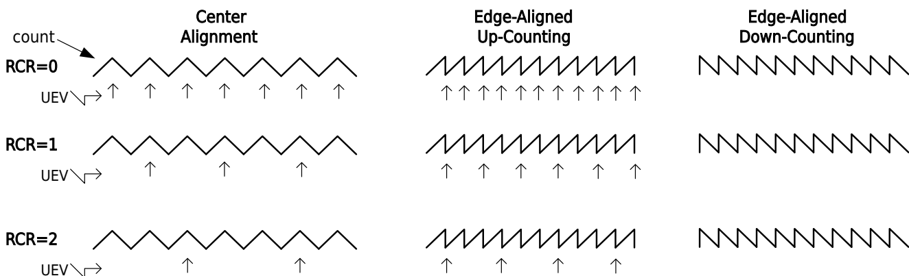
Figure 13-25 Update Timing Generated by Repetition Counter when Underflow Is Masked ( RCR.OV=0 , RCR.UD=1 )
