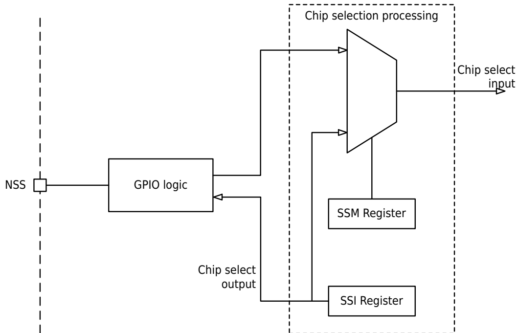
Figure 8-3 Slave Select NSS Pin Configuration
