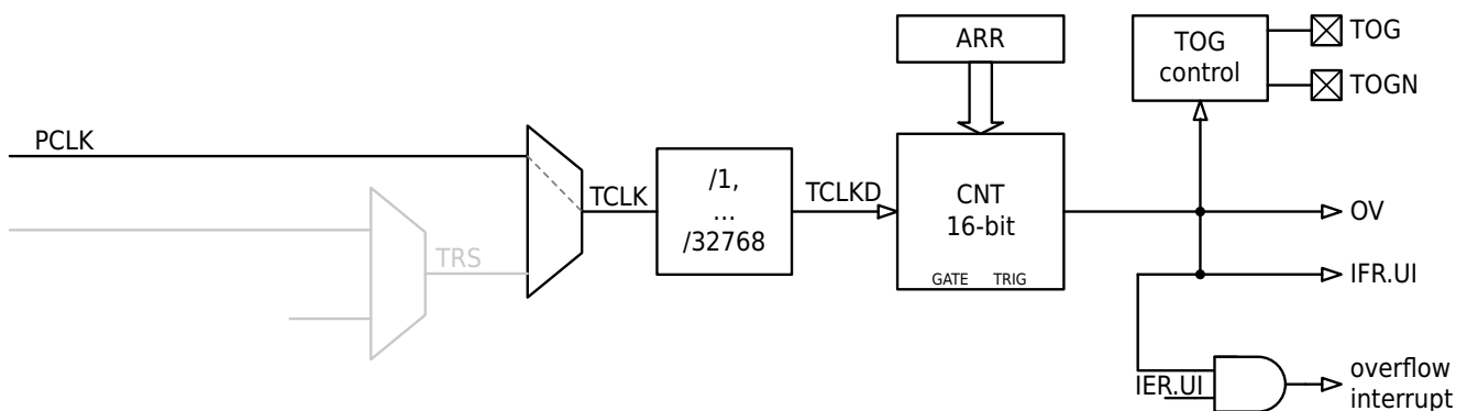
Figure 14-4 BTIM Timing Mode Block Diagram
