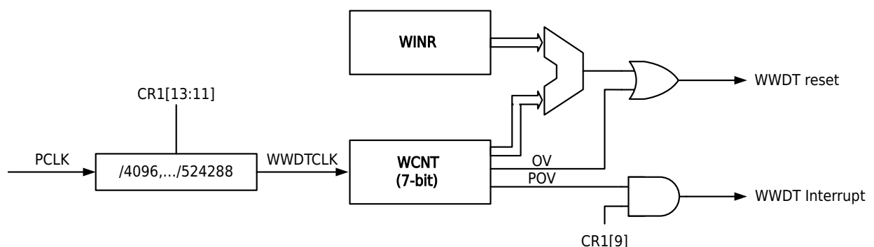
Figure 18-1 WWDT Function Block Diagram
