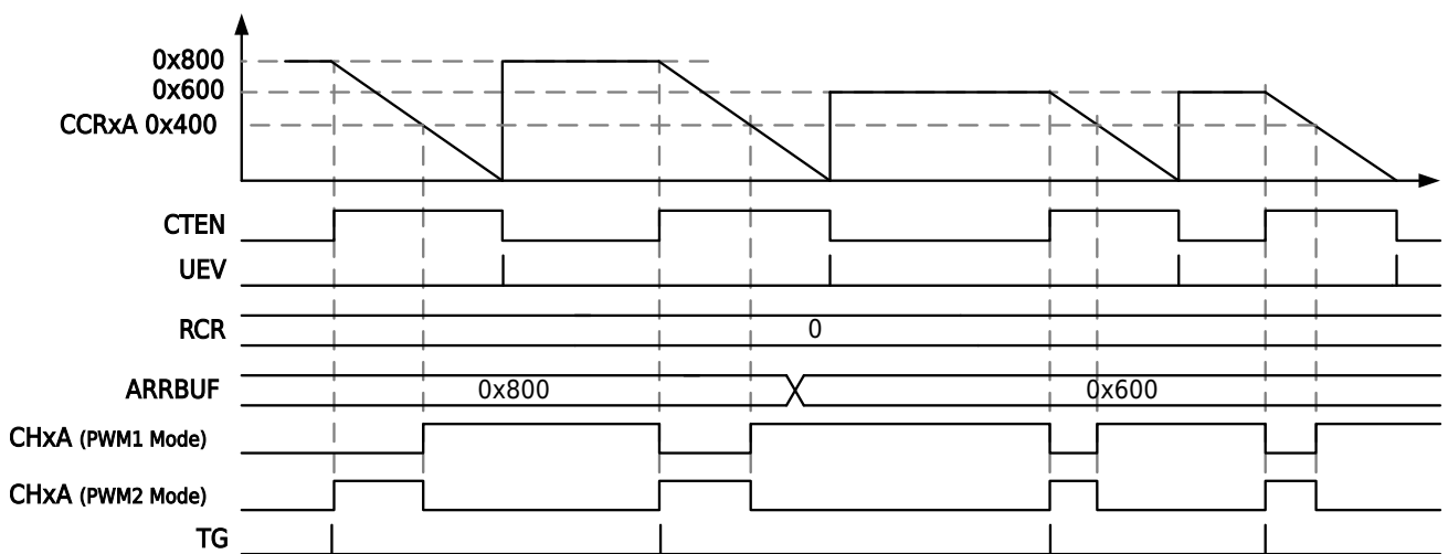
Figure 13-47 Sawtooth Down-Counting Single Pulse Mode
