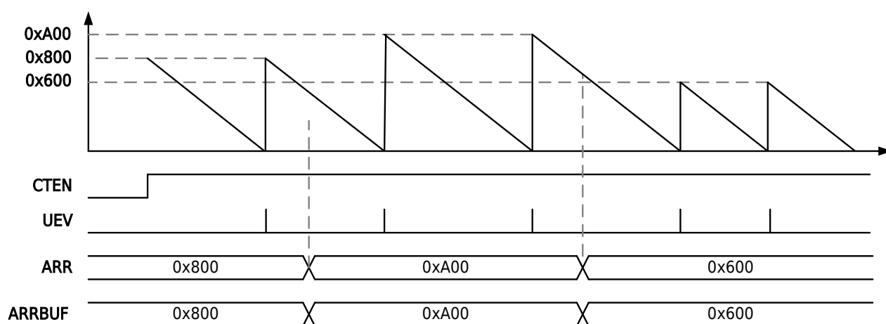
Figure 13-31 Mode 2 Sawtooth Wave Mode Down-Counting with Cache Invalid
