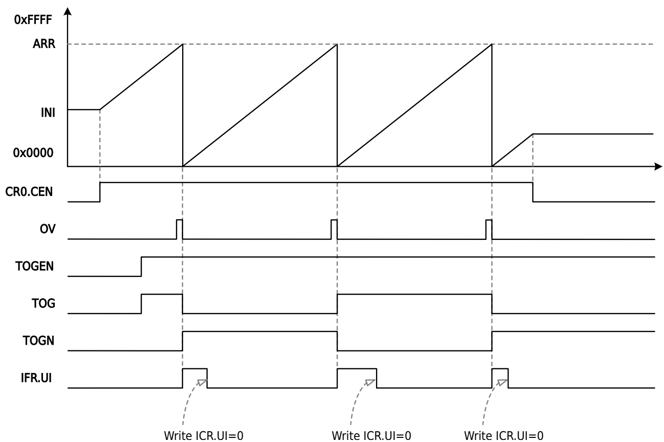
Figure 14-13 GTIM Counter Waveform
