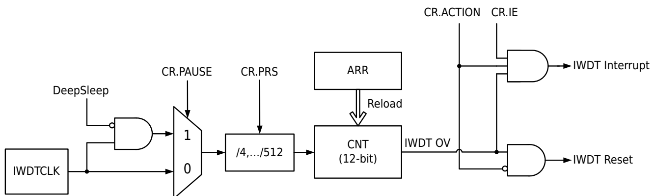
Figure 17-1 IWDT Function Block Diagram
