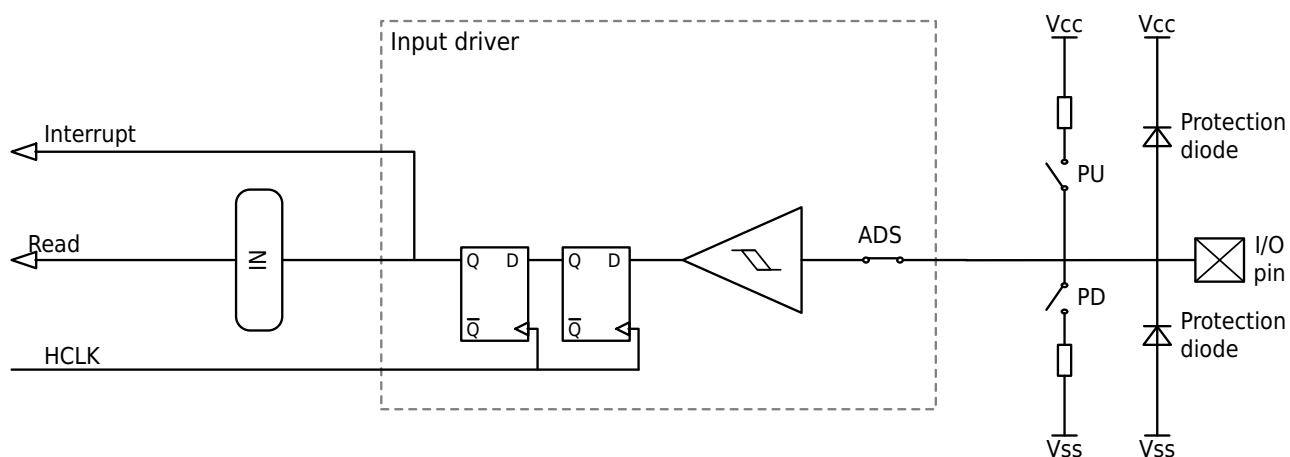
Figure 6-8 Port External Interrupt Diagram
