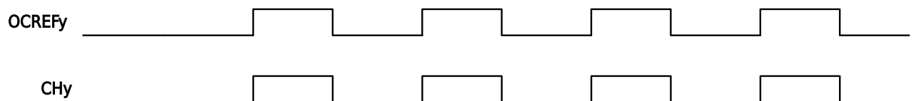
Figure 13-39 PWM Output Waveform When CCPy=0
