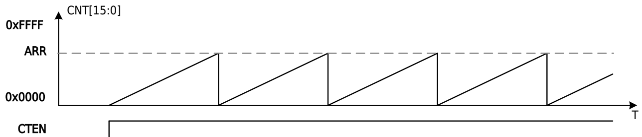
Figure 13-19 Mode2 Edge-Aligned Timer Waveform (M23CR.DIR=0)
