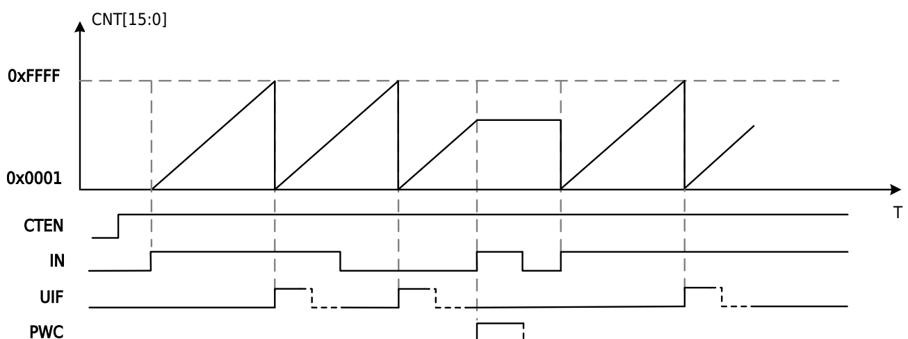
Figure 13-12 Model1: Pulse Width Measurement PWC Rising Edge to Rising Edge Period Measurement
