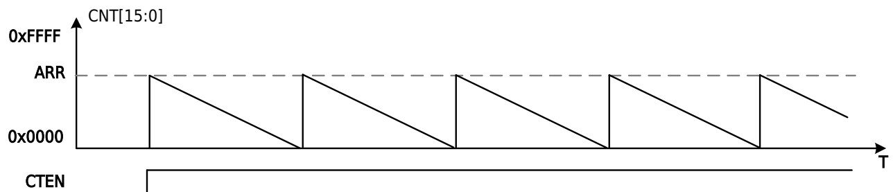
Figure 13-20 Mode2 Edge-Aligned Timer Waveform (M23CR.DIR=1)
