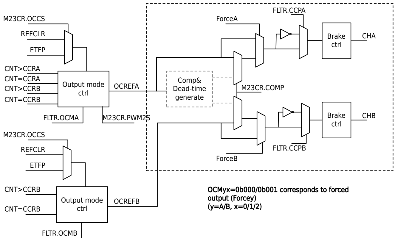
Figure 13-38 Independent PWM Output Block Diagram
