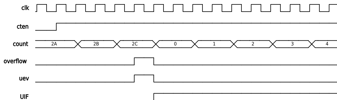
Figure 13-16 Mode 2 Compare Capture Mode Up-Counting With Prescaler
