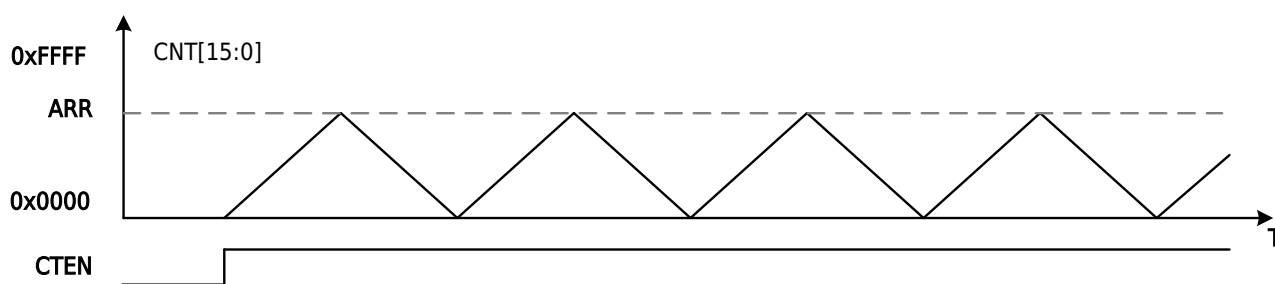
Figure 13-22 Mode3 Center-Aligned Counter Waveform
