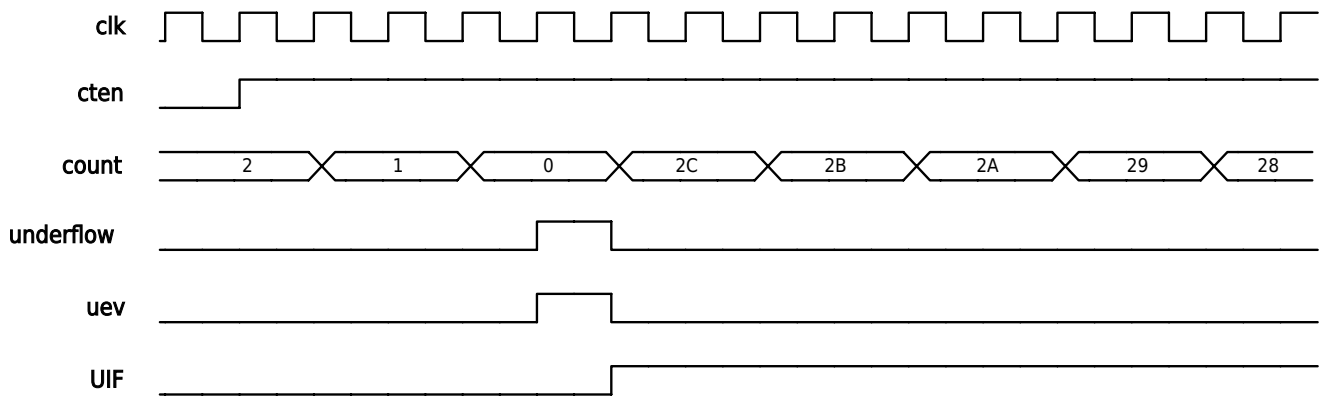
Figure 13-18 Mode 2 Compare Capture Mode Down-Counting With Prescaler
