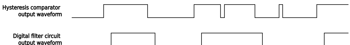
Figure 27-2 LVD Filter Output
