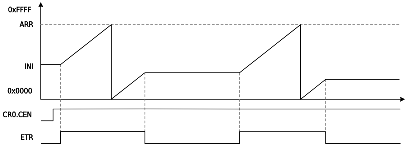
Figure 14-19 GTIM Gating Mode Counting Diagram
