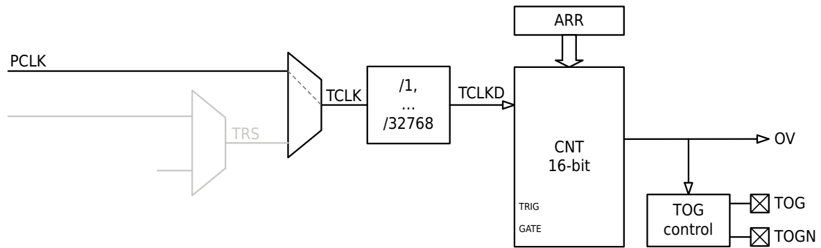
Figure 14-14 GTIM Timing Mode Block Diagram
