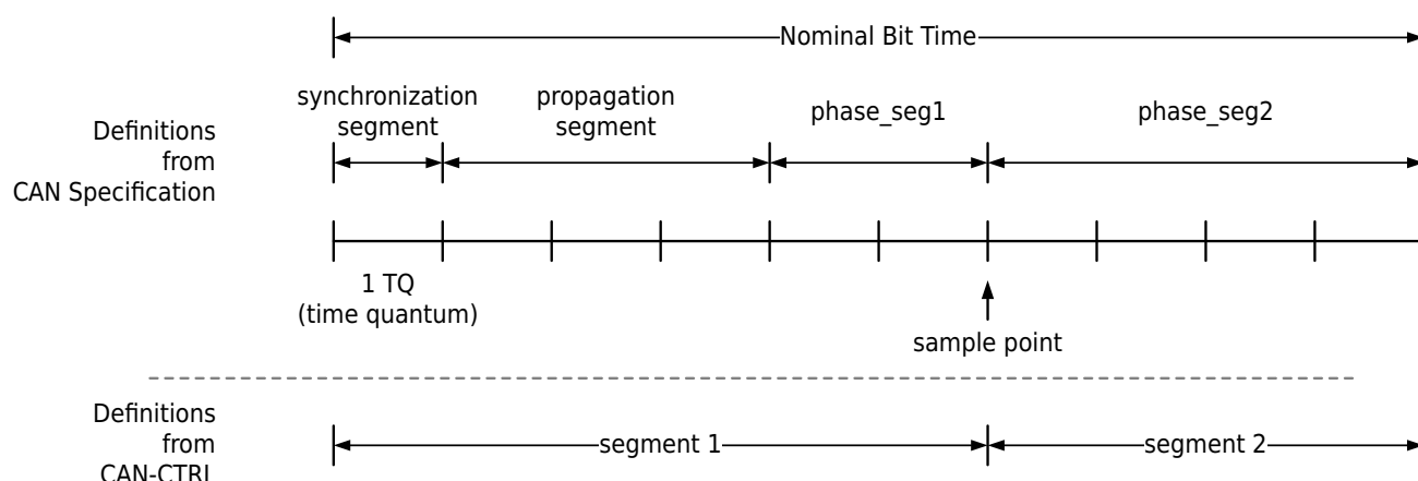
Figure 21-3 CAN Bit Time Definition Diagram
