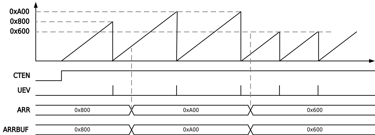
Figure 13-29 Mode 2 Sawtooth Wave Mode Up-Counting with Cache Invalid
