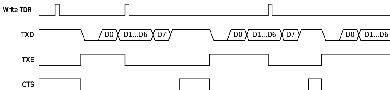
Figure 19-2 CTS Hardware Flow Control Signal
