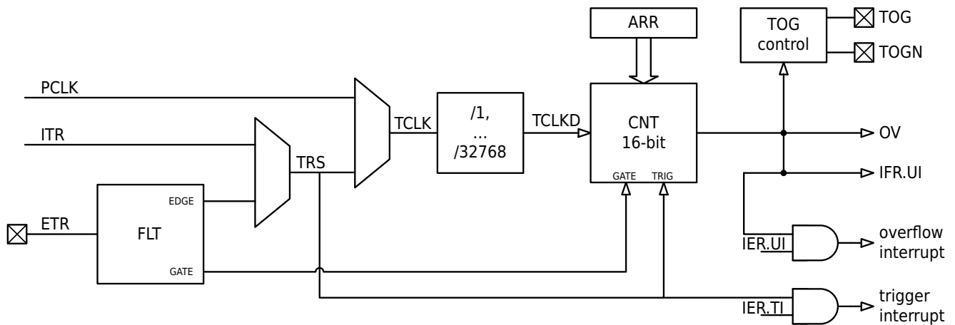
Figure 14-1 BTIM Block Diagram
