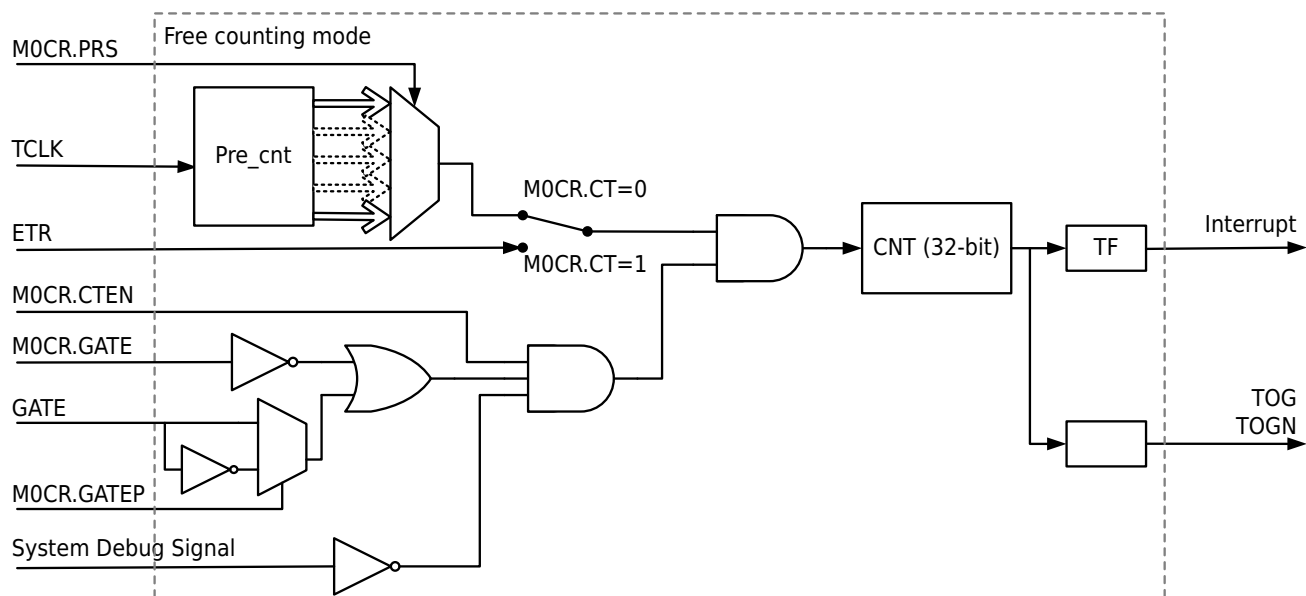
Figure 13-3 Mode0 Count Timer Free Counting Block Diagram
