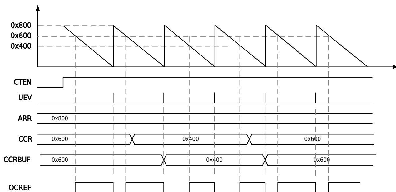
Figure 13-32 Mode2 Sawtooth Wave Down-Counting Mode with Compare Cache Enable
