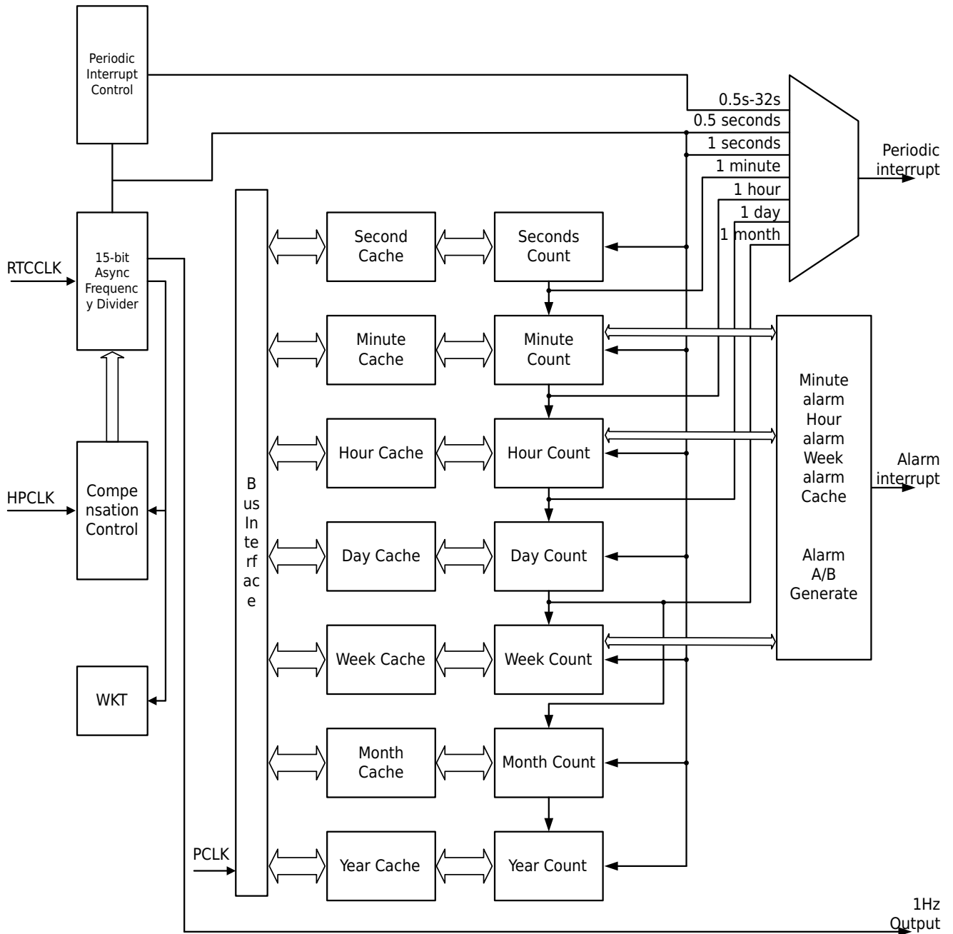
Figure 16-1 RTC Block Diagram
