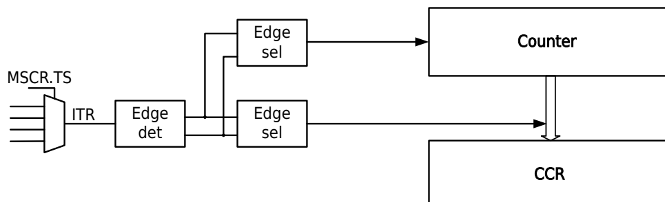
Figure 13-9 Mode1 Pulse Width Measurement PWC Function Block Diagram
