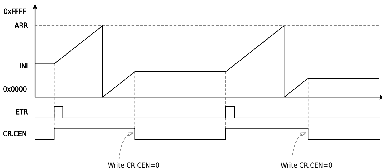
Figure 14-7 BTIM Trigger Start Mode Counting Diagram
