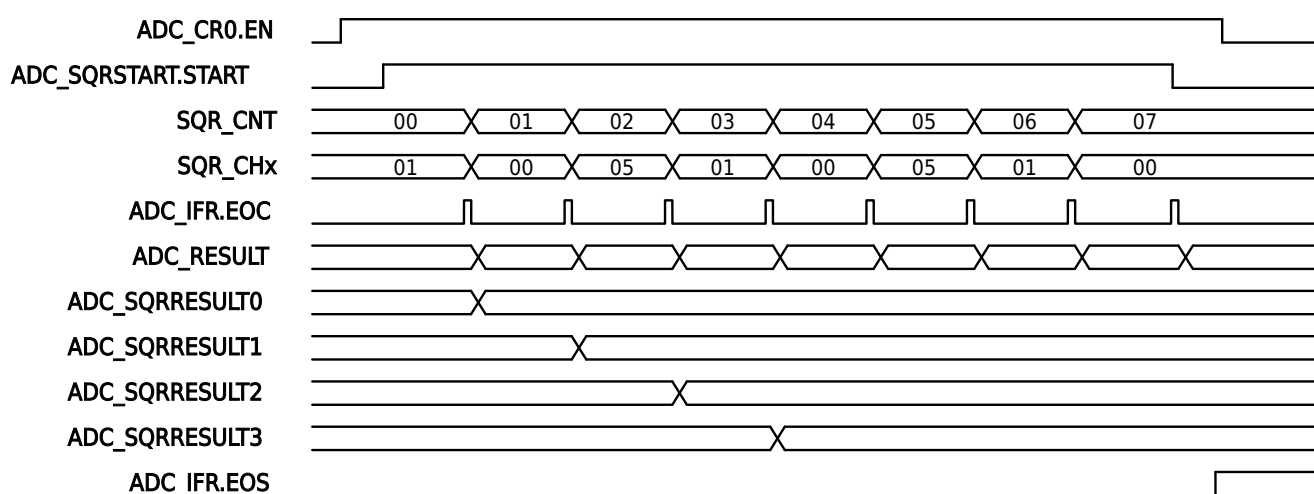
Figure 25-3 Examples of ADC SQR Scan Conversion Process
