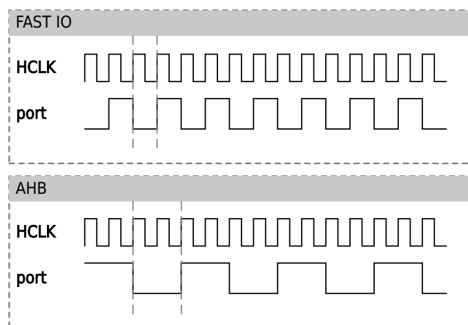
Figure 6-3 AHB/FASTIO Bus Port Changes with System Clock
