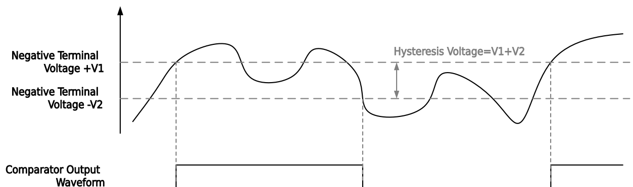
Figure 26-3 VC Hysteresis Function
