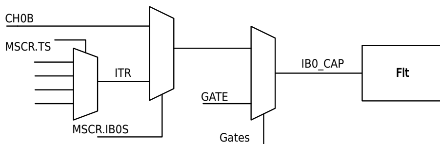
Figure 13-52 CH0B Capture Input Port Selection
