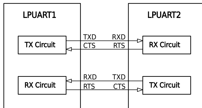
Figure 20-8 LPUART Hardware Flow Control
