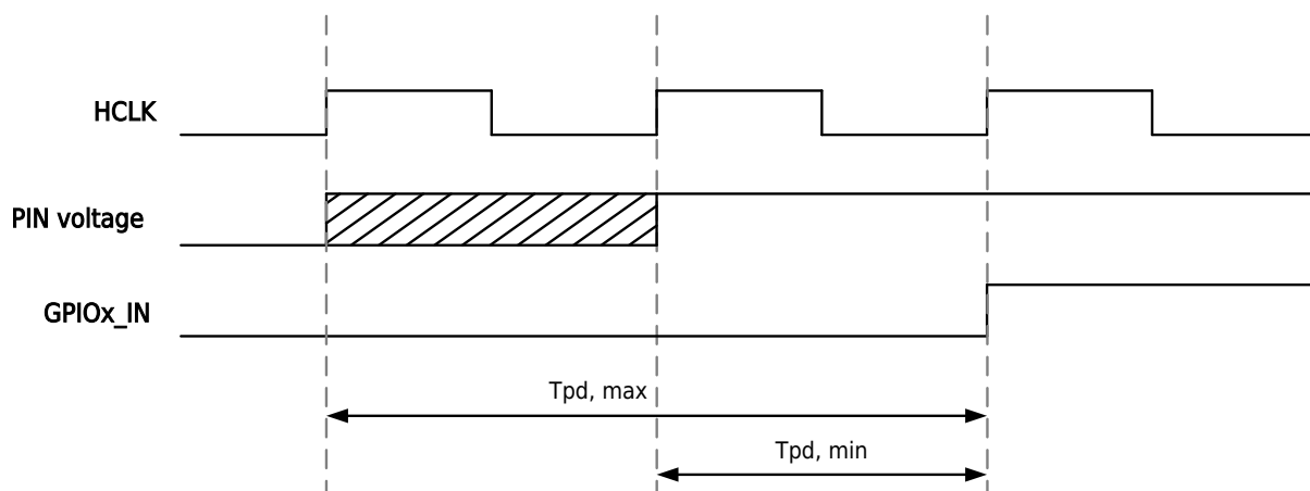
Figure 6-5 Read Port Pin Data Synchronization Diagram
