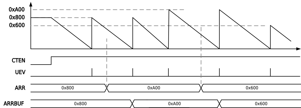
Figure 13-30 Mode 2 Sawtooth Wave Mode Down-Counting with Cache Enable
