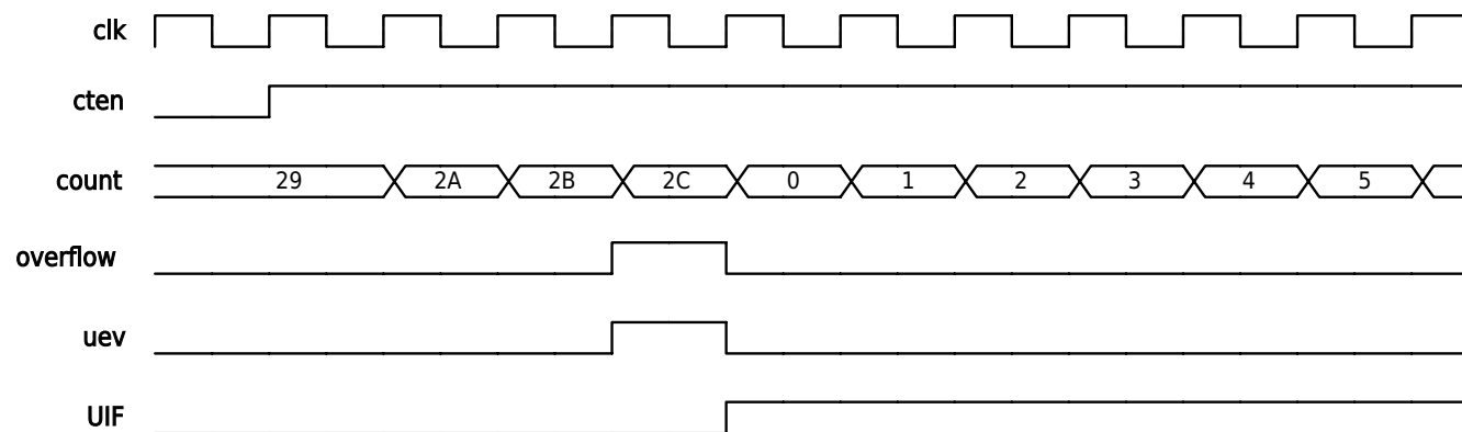
Figure 13-15 Mode 2 Compare Capture Mode Up-Counting Without Prescaler
