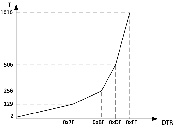
Figure 13-44 Dead Time
