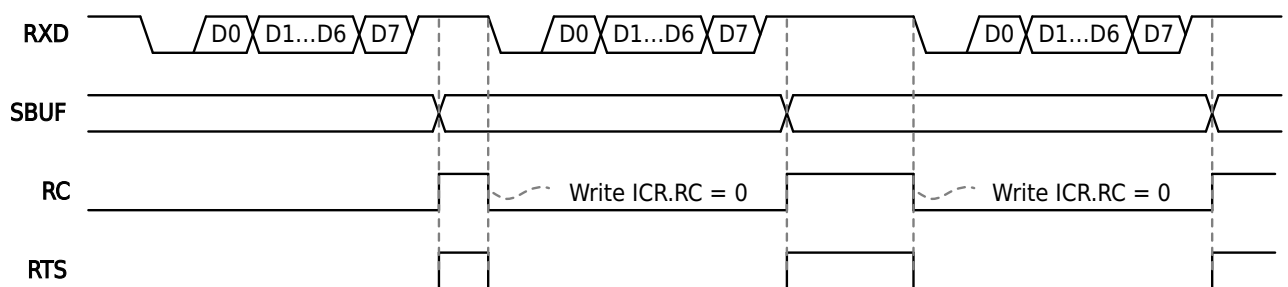
Figure 20-9 RTS Hardware Flow Control Signal
