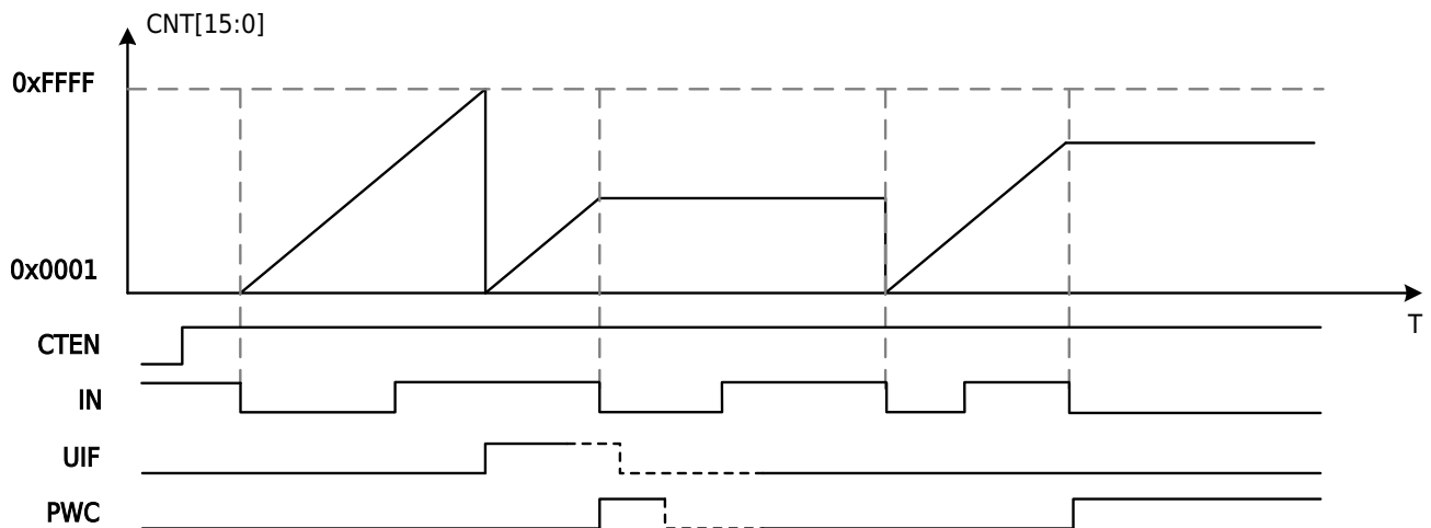
Figure 13-11 Model1: Pulse Width Measurement PWC Falling Edge to Falling Edge Period Measurement
