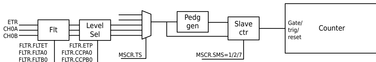
Figure 13-53 Mode2/3 Slave Mode Diagram
