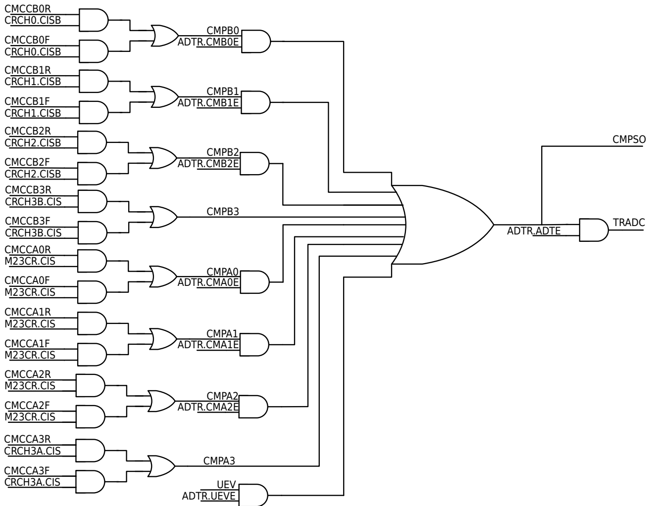
Figure 13-58 Timer Triggers ADC
