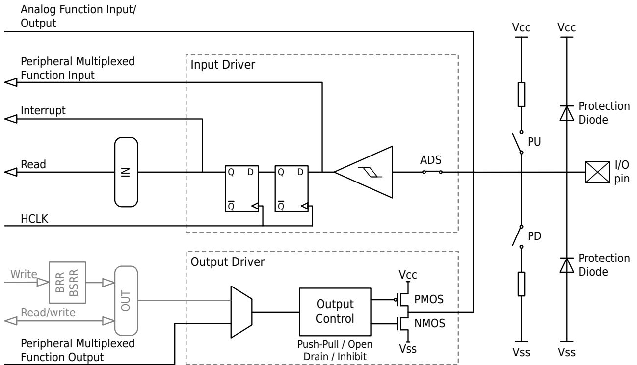
Figure 6-7 Multiplexed Function Configuration Diagram
