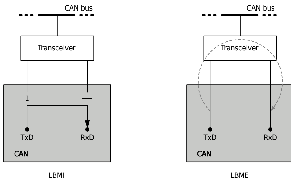
Figure 21-2 CAN LBMI and LBME Schematic Diagram
