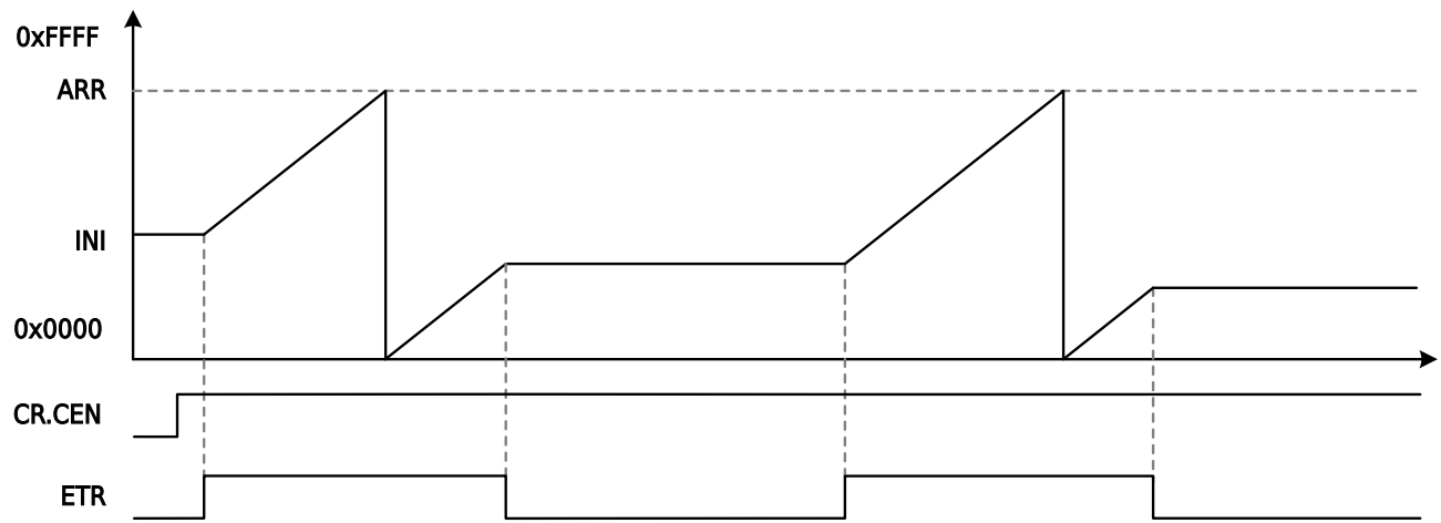
Figure 14-9 BTIM Gating Mode Counting Diagram
