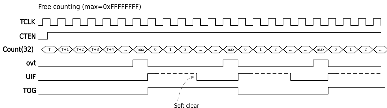
Figure 13-7 Mode0 Count Timer Free Counting Timing Diagram
