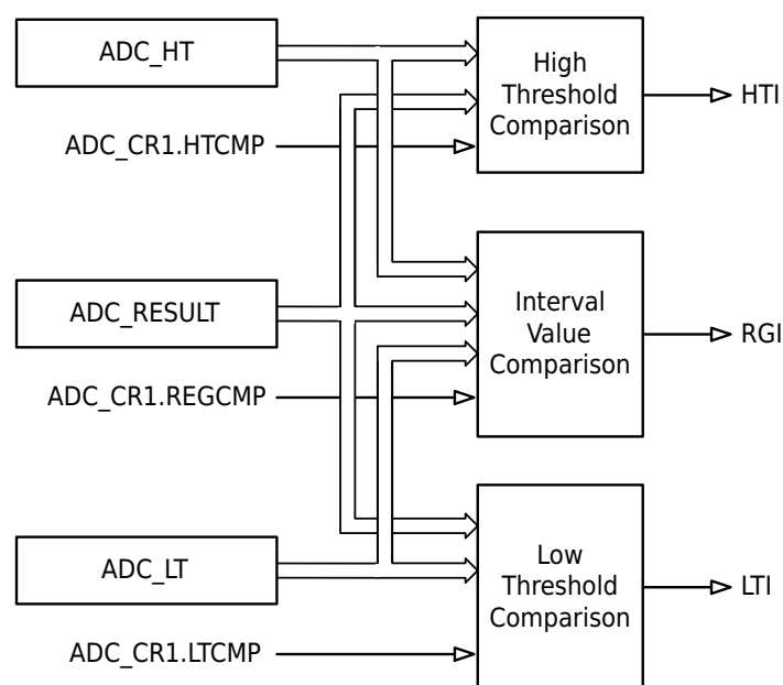
Figure 25-8 ADC Conversion Result Comparison Diagram
