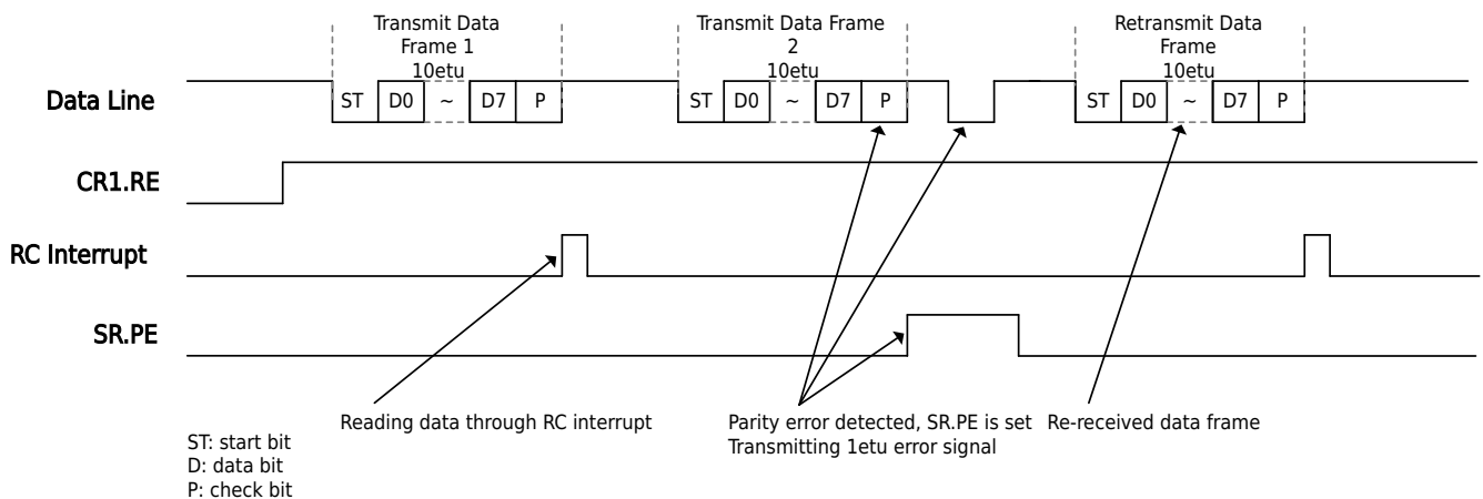
Figure 19-20 Smart Card Mode Receive Data Legend
