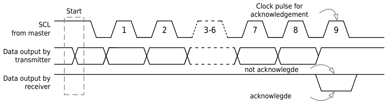
Figure 7-4 Acknowledgment Signal on I2C Bus
