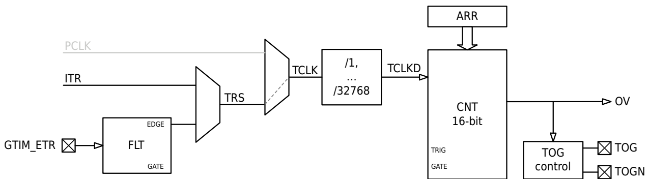
Figure 14-15 GTIM Counter Mode Block Diagram
