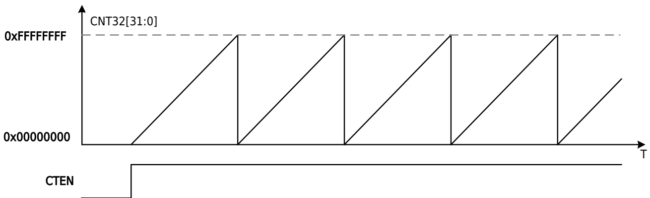
Figure 13-6 Mode0 Count Timer 32-Bit Free Counting Waveform
