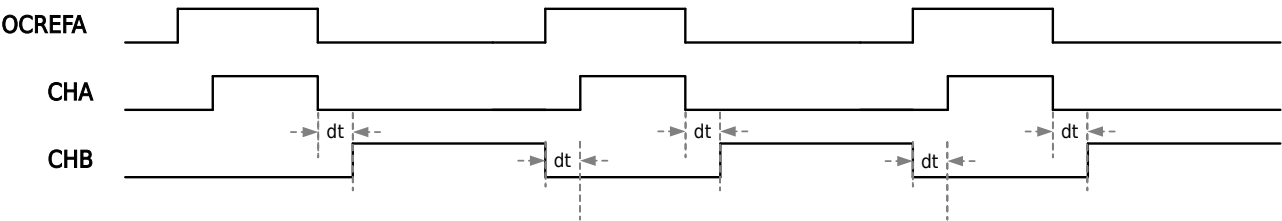
Figure 13-43 Complementary PWM Output Waveform (with Dead Time)
