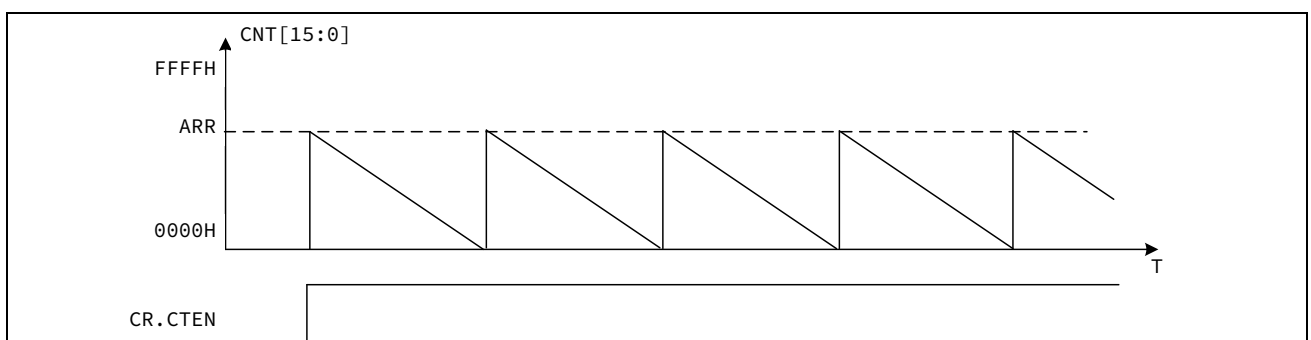
图 13-20 边沿对齐计时器波形 (DIR = 1)
